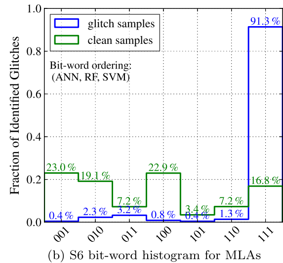
FIG. 6 (color online). Redundancy between MLA classifiers. These histograms show the fractions of detected glitches identified in common by a given set of classifiers at 1% probability of false alarm (blue). The abscissa is labeled with bit-words, which are indicators of which classifier(s) found that subset of glitches (e.g. 011 corresponds to glitches that were not found by ANN, but were found by RF and SVM). The quoted percentages represent the fractions of detected glitches so that 100% represents those glitches which were successfully identified by at least one of the classifiers at 1% false-alarm probability. The three classifiers show a large overlap for glitch identification (bit-word = 111), meaning the classifiers are largely able to identify the same glitch events. Also shown is the fraction of clean samples (green) misidentified as glitches, which shows a comparatively flat distribution across classifier combinations. Panel (a) shows the bit-word histograms for S4 data. Panel (b) shows the bit-word histograms for S6 data.
