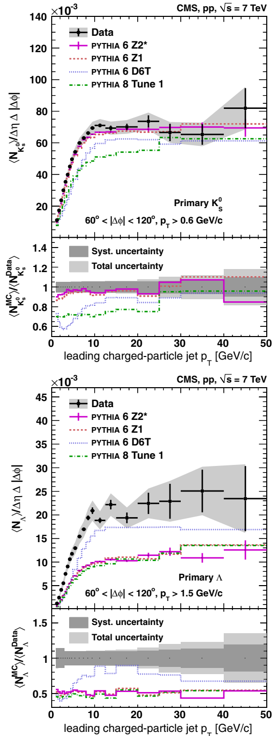
FIG. 4 (color online). Average multiplicity per unit of pseudorapidity and per radian in the transverse region ( |\eta| < 2 , 60^\circ < |\Delta\phi| < 120^\circ ), as a function of the p_T of the leading charged-particle jet: (top) K_S^0 with p_T > 0.6 GeV/c; (bottom) \Lambda with p_T > 1.5 GeV/c. Predictions of PYTHIA tunes are compared to the data, and the ratios of simulations to data are shown in the bottom panels. For the data, the statistical uncertainties (error bars) and the quadratic sum of statistical and systematic uncertainties (error band) are shown, while for simulations the uncertainty is only shown for PYTHIA 6 tune Z2*, for clarity.
