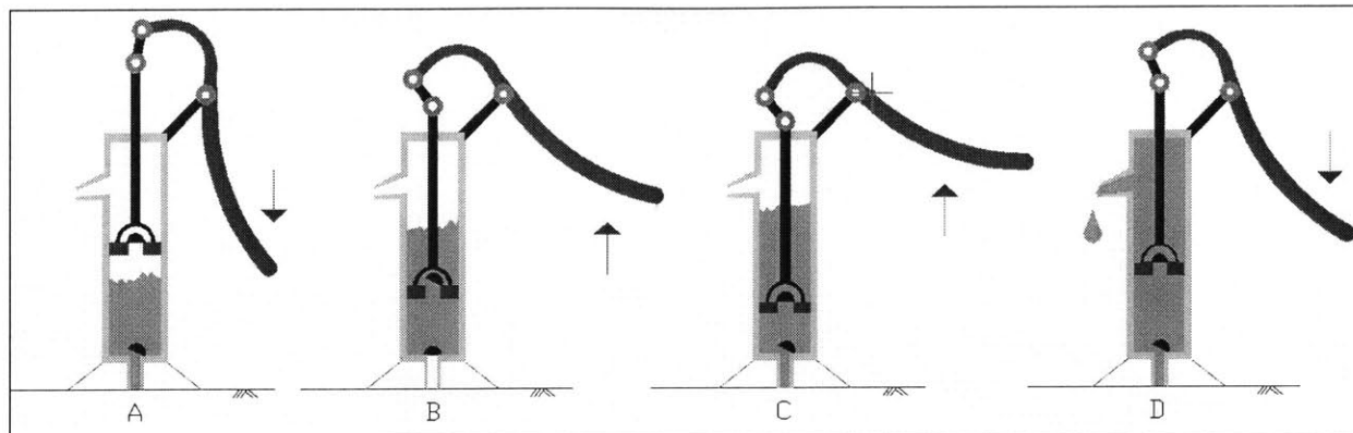
Figure 2-4. How a Suction Handpump Works
