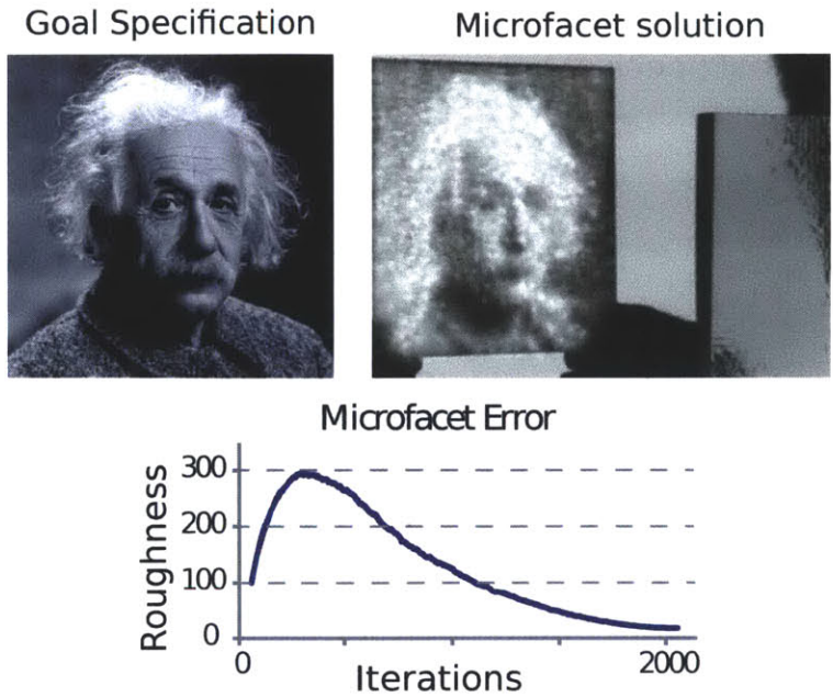
Figure 6-6: 3D printed lens arrays that produce a caustic image of Einstein. The algorithm is proposed by Papas et al. [22]. Below we show convergence plots for the microfacet optimizations. The portrait is available from the United States Library of Congress’s Prints and Photographs division, now in the public domain.
