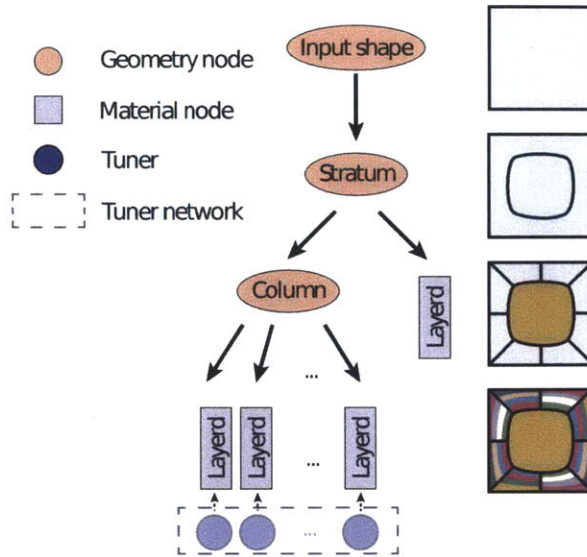
Figure 6-2: Reducer tree for texture.
