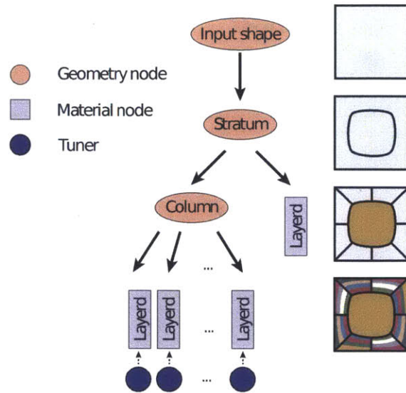
Figure 6-3: Reducer tree for heterogeneous subsurface scattering effect.
