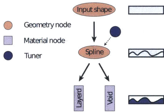
Figure 6-9: Reducer tree for smooth caustics.
