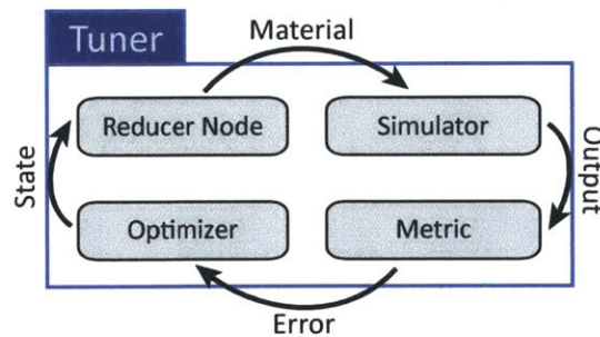
Figure 4-3: A diagram of the tuner workflow. Arrows indicate flow and type of information passed between the individual tuner components.
