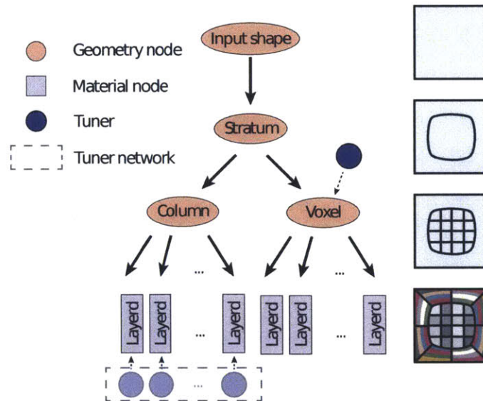
Figure 6-13: Reducer tree for combining texture and elastic behavior.
