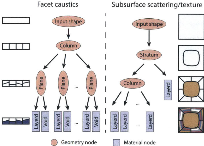
Figure 4-2: Two examples of reducer trees . Left: A tree for caustics effect. Right: a tree for subsurface scattering properties.
