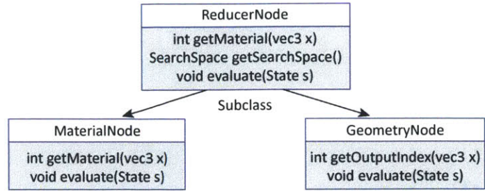
Figure 5-1: Abstract interface for Node and its two subclasses.
