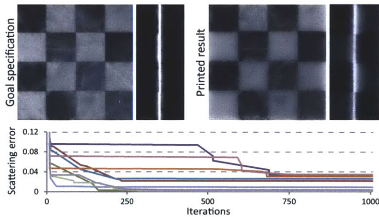
Figure 6-4: A marble chessboard with prescribed subsurface scattering properties produced by Hašan et al. [11]. The insets show the samples under thin line illumination, and the graph shows the convergence of tuners for 10 out of 100 scattering profiles used in the example. The error is measured by square distance between two profiles, each containing 400 coefficients.
