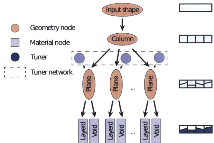
Figure 6-7: Reducer tree for facet caustics.
