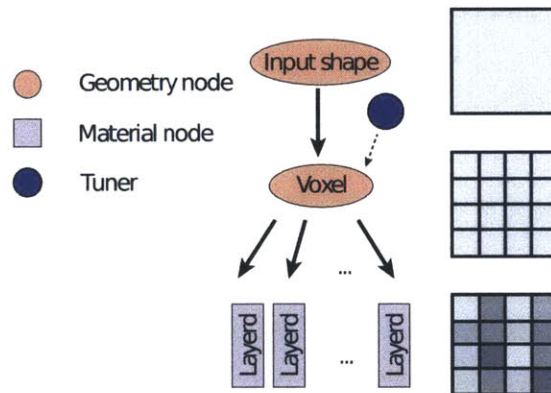
Figure 6-10: Reducer tree for elastic behavior.
