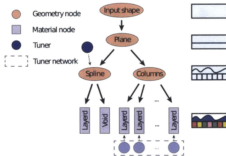
Figure 6-15: Reducer tree for combining texture and smooth caustics.
