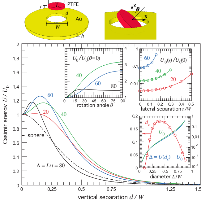
FIG. 1 (color online). Room-temperature Casimir energy U of a PTFE disk (thickness t = 10 nm) suspended above a Au plate (thickness h = 10 nm and inner and outer diameters W = 1 \mu\text{m} and D = 2W ) immersed in water, as a function of vertical separation d (normalized by W ). U is normalized by the energy in the coplanar configuration U_0 \equiv U(d=0) and plotted for multiple aspect ratios \Lambda = L/t , where L is the disk diameter. Also shown is the energy of a sphere of diameter 20t (dashed black line). Top insets: U as a function of rotation angle \theta (left) and lateral translations s (right) for multiple \Lambda . Bottom inset: Unstable equilibrium separation d_c (red circles), along with the energy U_0 (green line) and corresponding energy barrier \Delta = U(d_c) - U_0 (blue line), normalized by k_B T \approx 25 meV, as a function of L . Both d_c and L are normalized by W .
