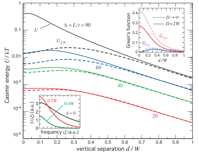
FIG. 2 (color online). Room-temperature Casimir U (solid lines) and Casimir-Polder U_{\text{CP}} (dashed lines) energies, normalized by k_B T \approx 25 meV, for the disk-plate geometry of Fig. 1, as a function of d (normalized by W ), plotted for multiple aspect ratios \Lambda = L/t . U_{\text{CP}} is obtained from the polarizability of the disks, as determined by Eq. (2). Top inset: Diagonal components of the photon GF of the plate evaluated along the axis of symmetry, for both finite D = 2W (solid lines, evaluated numerically) and semi-infinite D \rightarrow \infty PEC (dashed lines, evaluated analytically [33]) plates. Bottom inset: Casimir integrand U(i\xi) , in arbitrary units, as a function of imaginary frequency i\xi at three different separations d = \{0, 0.2, 0.4\}W , for \Lambda = 60 .
