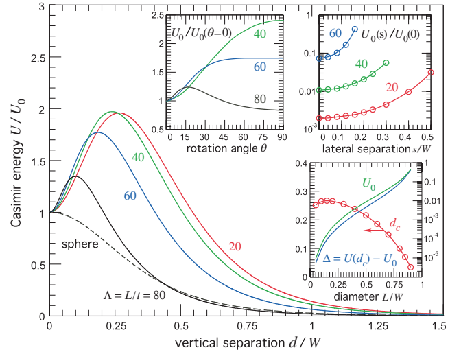
FIG. 3 (color online). Room-temperature Casimir energy U as a function of d for the disk-plate geometry of Fig. 1, but with the Au and PTFE materials interchanged. U is normalized by U_0 and plotted for multiple values of \Lambda . Top insets: U as a function of rotation angle \theta (left) and lateral translations s (right) for multiple \Lambda . Bottom inset: Unstable equilibrium separation d_c (red circles), along with U_0 (green line) and \Delta = U(d_c) - U_0 (blue line), normalized by k_B T \approx 25 meV, as a function of L . Both d_c and L are normalized by W .
