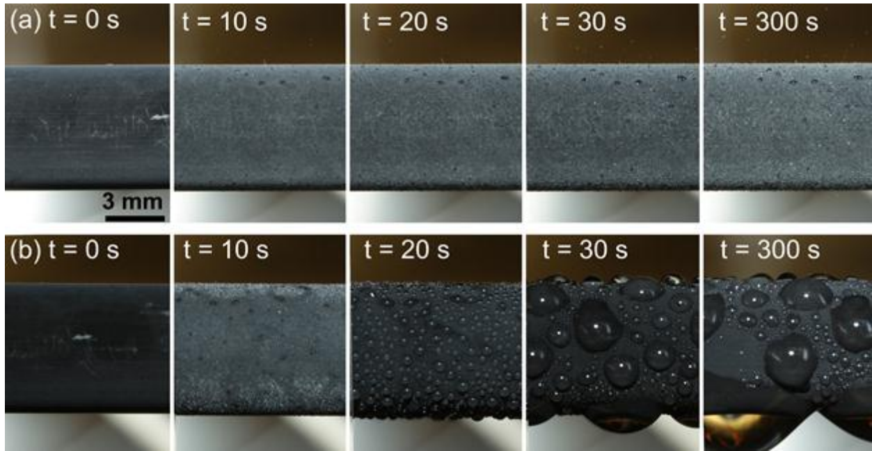
Figure 4 – Jumping and flooded condensation. Time-lapse images of initial water condensation on a 10 minute oxidized CuO sample undergoing (a) jumping, ( S = 1.08 , \Delta T_{LMTD} = 4 K, P_v = 2700 \pm 68 Pa) and (b) flooded condensation ( S = 1.54 , \Delta T_{LMTD} = 12 K, P_v = 2700 \pm 68 Pa). Low supersaturations ( S = 1.08 ) led to highly mobile partially wetting droplet formation and subsequent droplet jumping. High supersaturations ( S = 1.54 ) led to surface flooding and the formation of highly pinned Wenzel droplet morphologies.
