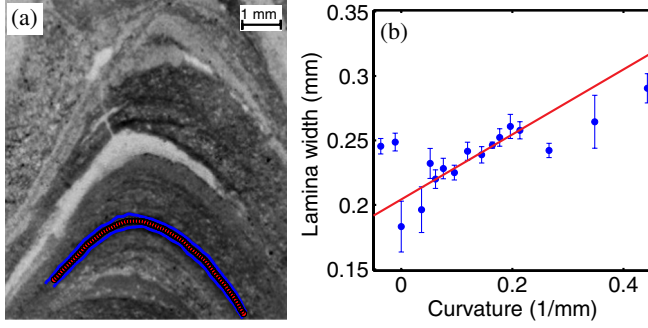
FIG. 3. The shape of stromatolite laminae records the stromatolite's evolution in time. (a) A 2.9 \times 10^9 -yr-old conical stromatolite from the Pongola Supergroup in South Africa cut vertically through the center. The transitions between light and dark laminae record the shape of the stromatolite at different points in time. The two solid blue curves represent the surface of the stromatolite at different times. This curve was measured by visually following the transition between a light lamina and a dark lamina. (b) The width of a lamina increases ( R^2 = 0.57 , p < 10^{-8} ) with curvature. Thus, the rate at which this stromatolite grew is an increasing function of curvature, consistent with Eq. (15). The fit of the measured lamina width and curvature to a straight line gives an estimate of the thickness of the overlying microbial mat \Delta = 1.2 \pm 0.6 \sim 1 mm. Two additional laminae from this sample are shown in the Supplemental Material. Additional curvature-thickness plots are shown in Fig. 5 and the Supplemental Material [41].
