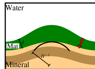
FIG. 7. A toy model of mat growth. Nutrients (arrow) diffuse through a microbial mat and are consumed. Near the nutrient-rich mat surface, the mat grows. At the nutrient-poor mat bottom, the mat decays. As described in Eq. (A15), mat thickness is determined by the balance of growth and decay. The equilibrium thickness varies with the curvature of the underlying stromatolite.
