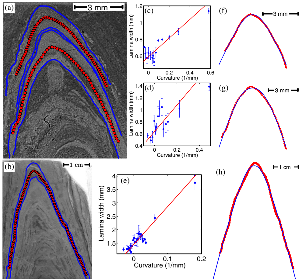
FIG. 5. Comparison of curvature-driven growth to the shapes of large and small conical stromatolites sectioned vertically through the center. (a) Thin section through a 2.9 \times 10^9 -yr-old conical stromatolite (photograph) [38]. Solid blue lines represent the upper and lower boundaries of two laminae. The red points lay along a curve equidistant from the traced laminae. (b) Thin section of a 1.6 \times 10^9 -yr-old stromatolite from the Bakal Formation [39,40] with traced laminae. (c) The thickness of the upper laminae from (a) increases with lamina curvature ( R^2 = 0.81 , p < 10^{-17} , \Delta = 1.9 \pm 0.7 mm), consistent with Eq. (15). (d) Similar agreement is found for the lower lamina ( R^2 = 0.64 , p < 10^{-8} , \Delta = 3.5 \pm 1.7 mm) and in the (e) Proterozoic sample shown in (b) ( R^2 = 0.88 , p < 10^{-44} , \Delta = 9.7 \pm 1.6 mm). (f),(g) Fitting two parameters, the measured shapes of the (f) upper and (g) lower laminae (points) are consistent with the shape (solid curve) of a lamina growing by the curvature-driven growth equation (19). (f) Fit of the sample from (b) to Eq. (19). All samples are cut through the central axis of the cone.
