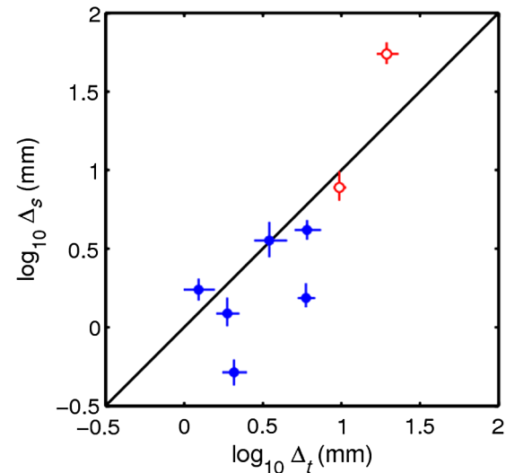
FIG. 6. Two estimates of the thicknesses of ancient stromatolite-forming microbial mats produce consistent values. \Delta_t is estimated from the relation between the curvature of a lamina and the distance to the neighboring laminas. \Delta_s is estimated from the shape of a single lamina. The black line shows equality. The measured slope is m = 2.3 \pm 1.6 , consistent with the predicted value m = 1 . The intercept b < 0 reflects that \Delta_t is systematically larger than the estimate of \Delta_s . Solid blue points represent stromatolites from the 2.9 \times 10^9 -yr-old Pongola Formation [38]. Open red points are from Proterozoic samples.
