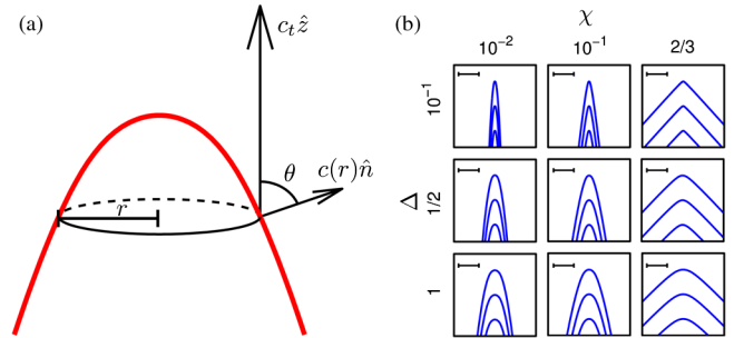
FIG. 4. A balance between curvature-driven growth and translational growth sets the shape of a conical stromatolite. (a) When a curve f(r) (red parabola) evolves due to curvature-driven growth, the normal velocity c is inversely proportional to the mean of the two radii of curvature at that point. When a curve translates forward, there is a geometric relationship between the speed at which a point translates c_t and the speed at which it grows in the normal direction c . (b) The shape of the stromatolite depends on two parameters. \chi^{-1} is the dimensionless speed of upward growth. The dimensional mat thickness \Delta gives the importance of curvature-driven growth. Values of \Delta are given relative to the thickness of the mat d_0 . The scale bar is 5d_0 .
