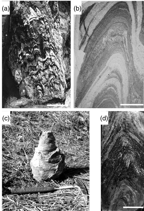
FIG. 1. Conical stromatolites from the Archean and Proterozoic, as seen in the field and in thin sections. (a) A side view of a rock formed by many small conical stromatolites from the Pongola Supergroup [38]. The scale bar is 1 cm. (b) Thin section of a stromatolite from (a). The scale bar is 0.5 cm. (c) Large conical stromatolite from the Bakal Formation [39]. The hammer is approximately 30 cm long. (d) Thin section of a large cone from the Bakal Formation showing thin bands called laminae. These changes in color and texture record the shape and position of the stromatolite surface at different points in time. The scale bar is 1 cm.
