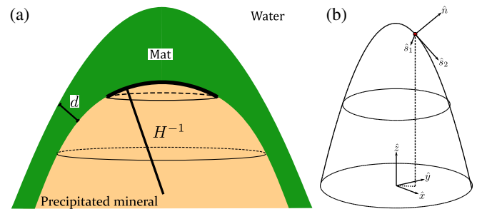
FIG. 2. A schematic of a simplified stromatolite. (a) The stromatolite grows as chemicals diffuse through the microbial mat and precipitate at the base of the mat. The thickness d of the mat varies over the surface of the stromatolite. The shape of the interface between the microbial mat and the stromatolite is described by the local curvature H . At the tip of an axisymmetric stromatolite, H^{-1} is the radius of curvature. (b) The transformation from Cartesian coordinates to the local coordinates of the surface f(x, y) . The unit vectors \hat{s}_1 and \hat{s}_2 are tangent to the surface. The vector \hat{n} is the local normal. The position of the red circle on the stromatolite surface can be expressed in Cartesian coordinates as [x_0, y_0, f(x_0, y_0)] or in the local coordinates as (s_1, s_2, 0) , where s_1 and s_2 are measured along the stromatolite surface from some known point. For the sake of illustration, we have shown f as a paraboloid.
