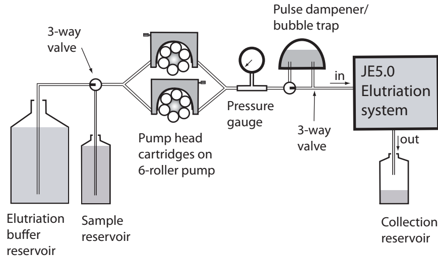
Figure 2-4: Schematic of counterflow centrifugal elutriation system. The specific parts used in my system are listed in Table 2.1 (p.43). This setup was inspired by [170] and the JE5.0 elutriation system instruction manual (©2004). As described in the main text, I used two identically-configured elutriation systems in parallel for most of my experiments.
