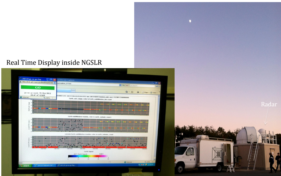
Figure 3. Photograph of NGSLR (right) during an LRO LR measurement session on November 4, 2012 and a display of the near real time LRO feedback (left). The top plot indicates the average arrival time of the detected LR pulses within the 8-ms LR range-gate window over a 1-second integration time. The middle plot shows the peak location of the histogram of the detected LR pulses over a 1-second integration time. The color indicates the frequency of the LR pulse detection, with red indicating near 100% (28Hz) detection. The bottom plot shows the peak location of the histogram away from those in the middle plot and may indicate signal detection from a second ground station during simultaneous ranging. The red line at the bottom of the bottom plot indicates the successful detection of the LR pulses based on their statistics. The pattern of the LR pulses in the range window shown in the plot, alternating between two levels, was the pre-programmed pattern used to show the feasibility of the simultaneous ranging and communication.
