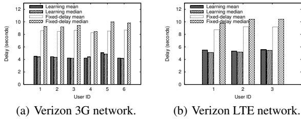
Figure 15: Mean and median delays for traffic bursts using learning algorithm and fixed delay bound scheme.
