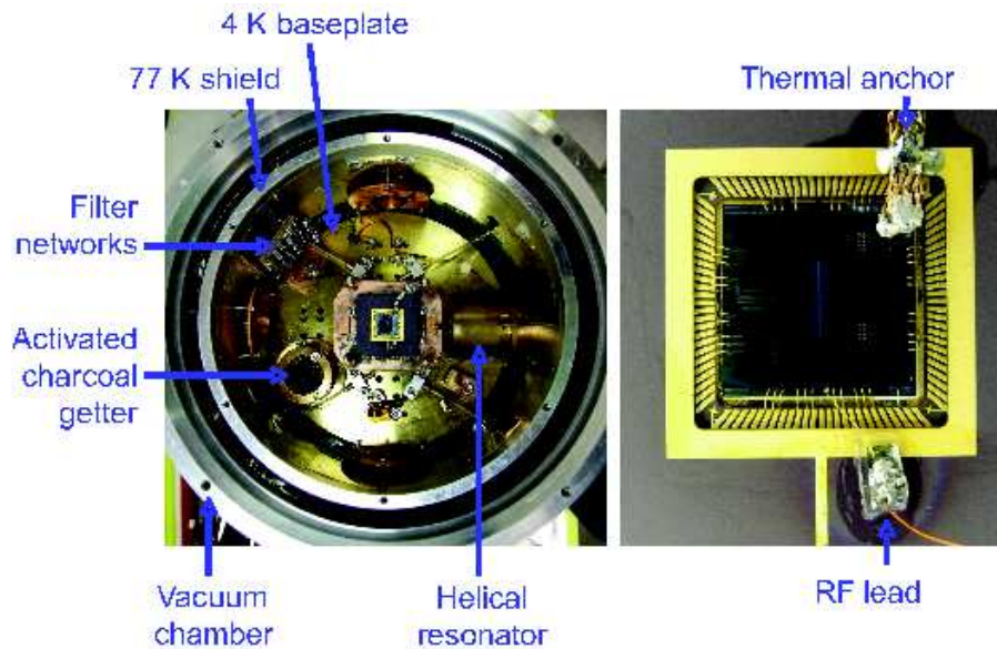
Fig. 8. Setup for cryogenic testing. On the left is a picture of the 4 K baseplate of the cryostat with the trap mounted in the center. Also visible are the electronic filter networks used to reduce the voltage noise on the DC electrodes (thermally anchored to the 4 K baseplate), the helical resonator used to generate the RF trap drive (thermally anchored to the 77 K shield), and one of the activated charcoal getters used to pump the vacuum chamber (thermally anchored to the 4 K baseplate). Not pictured are the Sr oven used to load the trap (which is mounted to the front of the helical resonator) and the aspheric lens used to image the ions (which is mounted above the trap inside the vacuum chamber). On the right is a picture of the trap. The copper braid in the top right corner is used to provide a good thermal contact between the trap and the 4 K cryostat baseplate. The RF lead is not routed through the CPGA to reduce capacitance.
