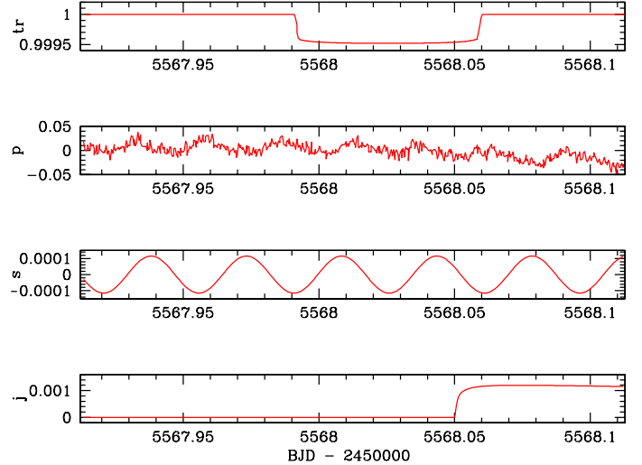
Fig. 5. Spatially- and time-dependent terms of the model function used in Eq. (2). Model terms are described as follows: tr is the transit model, p is the pixel phase correction ( a_2, a_3, a_4, a_5 and a_6 in Eq. (2)), s is the sinusoidal ( a_8, a_9 and a_{10} ) and j is the jump model ( a_{11} and a_{12} ). The linear trend a_7 is not represented.
