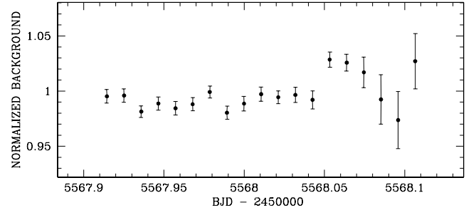
Fig. 2. Background time-series for the 55 Cnc data, after normalization and binning per 15 min intervals.
