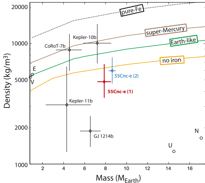
Fig. 7. Density vs. mass of transiting super-Earths. The data for the known transiting super-Earths and mini-Neptunes are shown, as well as the relationships for the four rocky compositions considered in this study. Earth, Venus, Uranus and Neptune are shown for reference. The error bars for the density are calculated as \rho_{\min} = 4\pi/3 (M - \sigma M)/(R + \sigma R)^3 and \rho_{\max} = 4\pi/3 (M + \sigma M)/(R - \sigma R)^3 .
