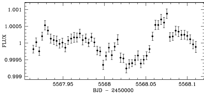
Fig. 3. 55 Cnc light curve corrected for the “pixel-phase” effect using a 2nd order position polynomial and binned to intervals of 5 min.
