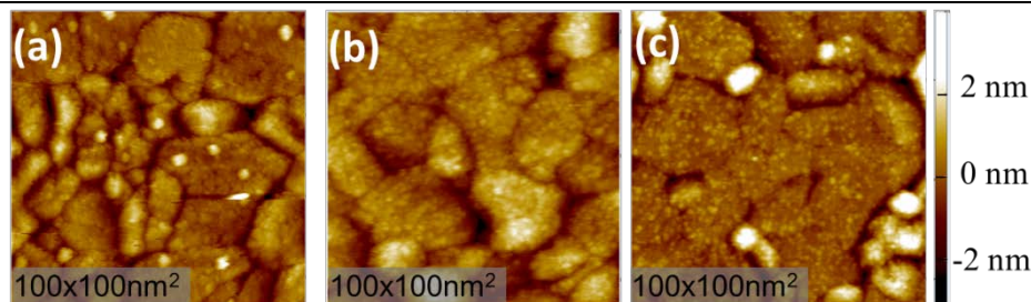
Fig. 1: Surface structure of 20 nm thick (a) \text{SrTi}_{0.95}\text{Fe}_{0.05}\text{O}_3 (STF5), (b) \text{SrTi}_{0.65}\text{Fe}_{0.35}\text{O}_3 (STF35) and (c) \text{SrFeO}_3 (STF100) films, imaged by scanning tunnelling microscopy (STM) at 345 °C and 1 \times 10^{-3} mbar oxygen pressure.
