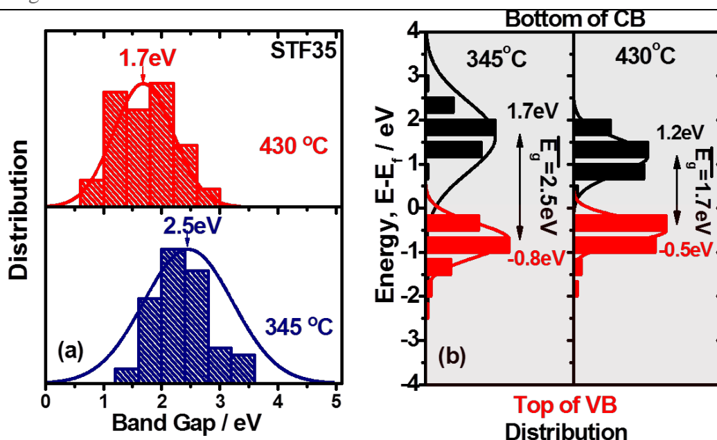
Fig. 5 (a): Comparison of the surface band gap, E_g at the surface of STF35 measured by scanning tunnelling spectroscopy at P_{O_2} \sim 1 \times 10^{-3} mbar and two different temperatures of 345 °C and 430 °C. (b) Distribution of band edges, the top of valence band (in red) and the bottom of conduction band (in black), for STF35 under the same conditions as in (a).
