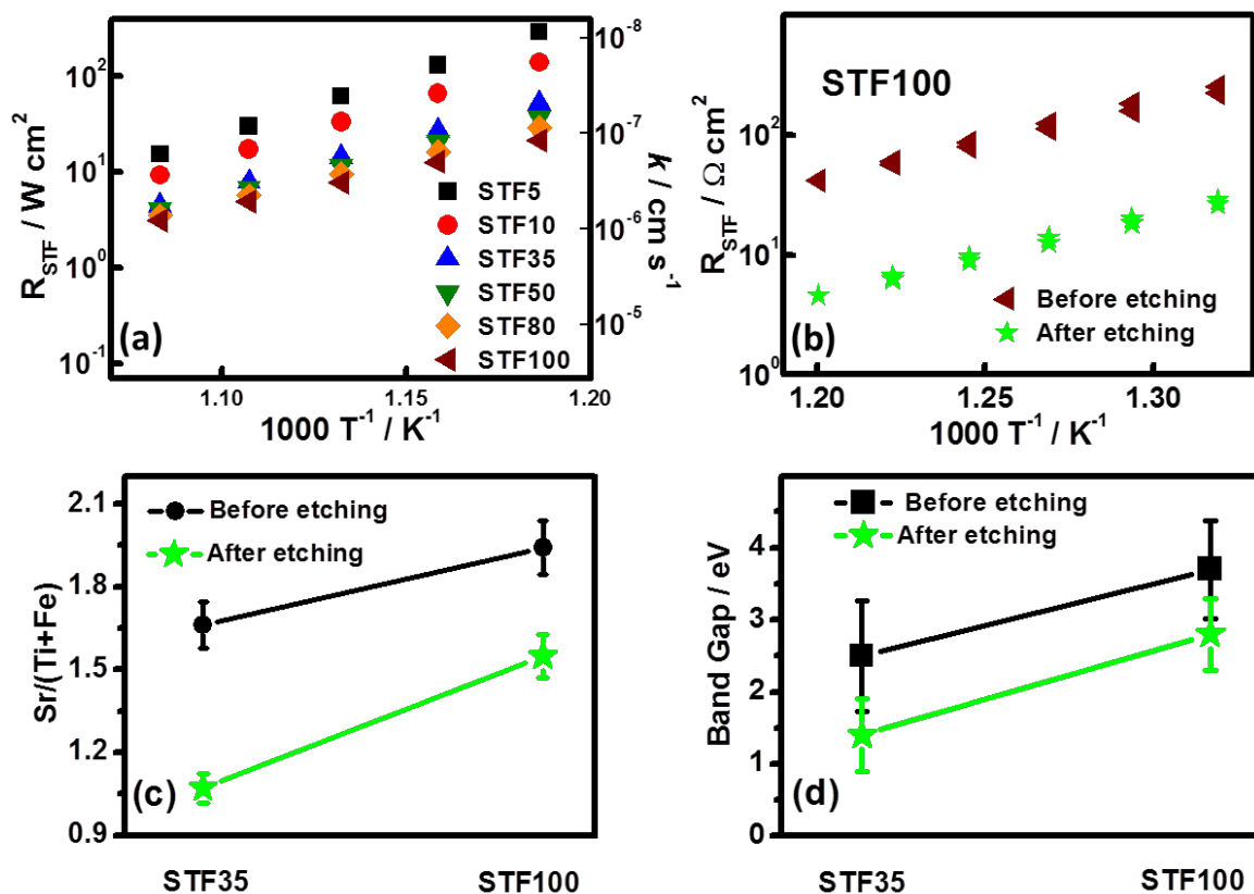
Fig. 7: (a) Temperature dependence of the area specific resistance ( R_{STF} ) and surface exchange coefficient ( k ) for STF thin film electrodes. (b) R_{STF} for STF100 are shown both before and after chemical etching to remove Sr excess phase. (Figures a and b are reproduced with permission from Ref. 18 ) (c) Comparison of the ratio of A site to B site cations, \text{Sr}/(\text{Fe}+\text{Ti}) quantified from XPS, for STF35 and STF100 before and after HCl etching. (d) Comparison of band gap measured by STS for STF35 and STF100 before and after HCl etching.
