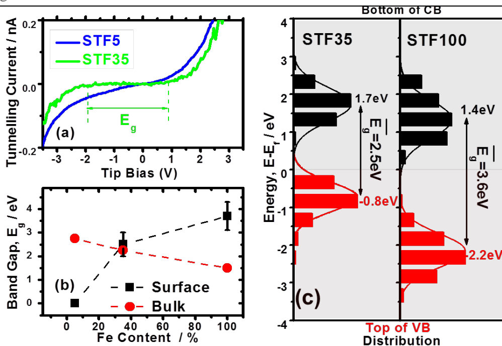
Fig. 4 (a) Representative tunnelling spectra on the STF5 and STF35 surfaces, showing the lack and the presence of a band gap, E_g , respectively. (b) Comparison of the band gap at the surface (black squares) measured by scanning tunnelling spectroscopy (STS) in this work and in the bulk (red circles) for STF5, STF35 and STF100. The “Bulk” values are taken from ref. 30 . (c) Distribution of the band edges, the top of valence band (in red) and the bottom of conduction band (in black), for STF35 and STF100. All surface STS measurements reported in a-c are at P_{O_2} \sim 1 \times 10^{-3} mbar and 345 °C.
