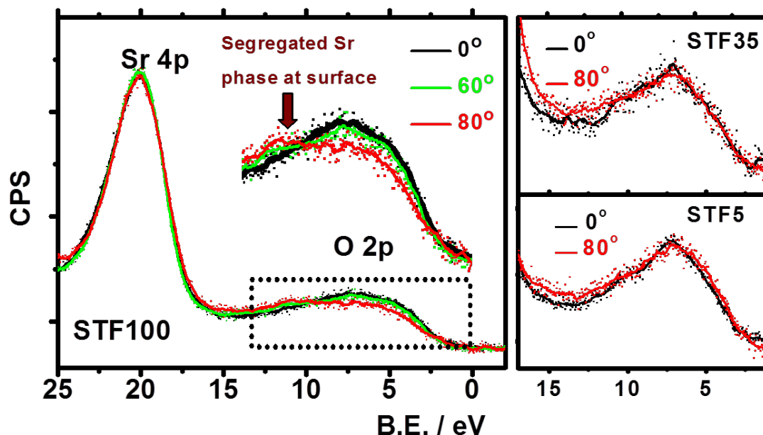
Fig. 6: Valence band structure obtained by angle-resolved x-ray photoelectron spectroscopy on STF100, STF35 and STF5 at different detection angles.
