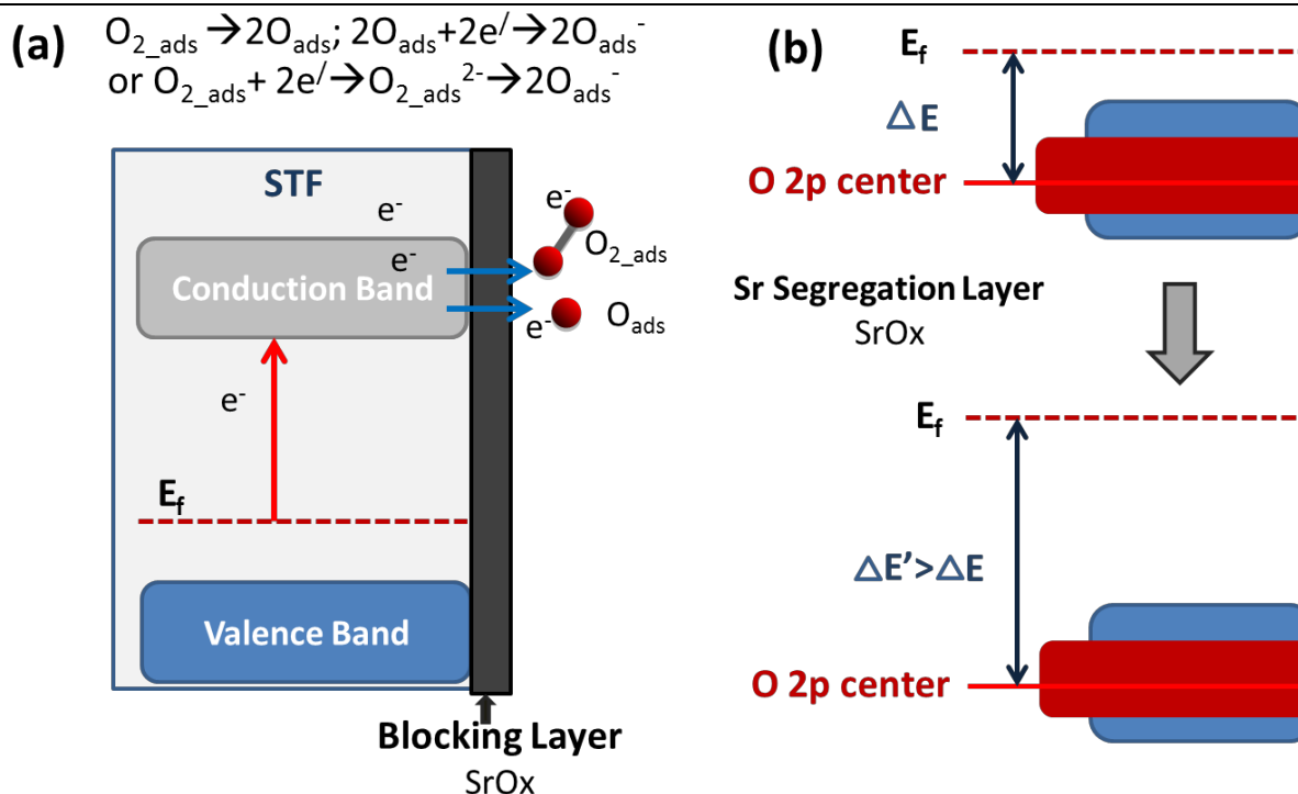
Fig. 8: Two possible mechanisms of how Sr segregation in the form of SrO_x on the surface impacts the oxygen reduction kinetics: (a) The Sr segregation layer, SrO_x serves as a barrier layer that inhibits electron transfer from bulk STF to O_2 or O adsorbing onto the surface; (b) Downshift in the O\ 2p position is associated with a more stable oxygen sub-lattice and consequently a smaller amount of oxygen vacancies are available on the surface for oxygen adsorption and incorporation into the lattice. Red box and blue box represent the O\ 2p states and transition metal 3d states, respectively.
