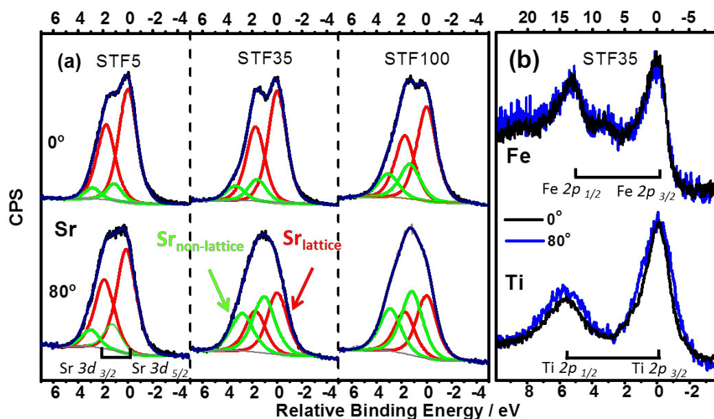
Fig. 2: a) Comparison of the Sr 3d spectra on STF5, STF35 and STF100 at emission angles of 0° and 80°. The red doublets correspond to the bulk-coordinated \text{Sr}_{\text{lattice}} and the green doublets are attributed to the binding environment on the surface \text{Sr}_{\text{non-lattice}} . The binding energy of the Sr spectra was referenced to the peak position of the 3d_{5/2} peak in the main doublet ( \text{Sr}_{\text{lattice}} ) for comparison. b) Comparison of the Fe 2p and Ti 2p spectra of STF35 at emission angles of 0° and 80°. The binding energies on the Fe spectra and Ti spectra were referenced to \text{Fe } 2p_{3/2} and \text{Ti } 2p_{3/2} , respectively.
