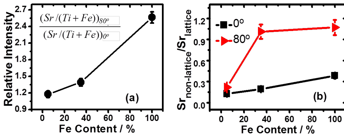
Fig.3: a) Comparison of the relative Sr enrichment on the surface of STF thin films with varying Fe content. b) The ratio of Sr in the non-lattice phase to Sr in the lattice phase (as shown in Fig. 2) on the surface ( \theta = 80^\circ ) and in the bulk ( \theta = 0^\circ ) in SrTi_{0.95}Fe_{0.05}O_3 (STF5), SrTi_{0.65}Fe_{0.35}O_3 (STF35) and SrFeO_3 (STF100).
