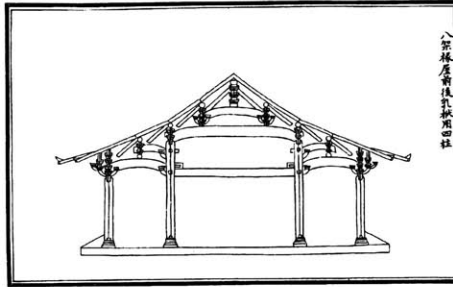
An 8-rafter building, 2-rafter beam in front and back, with 4 columns. 8- jia chuan wu , qian hou rufu , yong 4 zhu .
