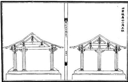
Left [description assumed]. A 4-rafter building, a 1-rafter beam abutting a 3-rafter beam, with 3 columns. 4- jia chuan wu , zhaqian dui 3-chuan fu , yong 3 zhu . Right. A 4-rafter building, centrally divided, with 3 columns. 4- jia chuan wu , fen xin , yong 3 zhu .
