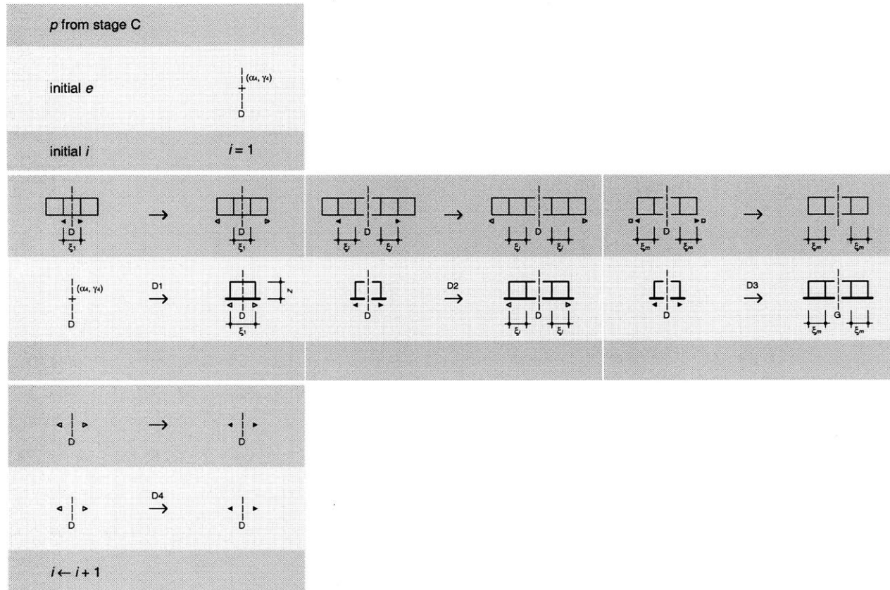
Figure 22. Schemata for generating partial scale elevations (stage D).
