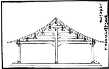
A 10-rafter building, centrally divided, with 3 columns. 10- jia chuan wu , fen xin , yong 3 zhu .
