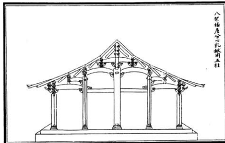
An 8-rafter building, centrally divided, a 2-rafter beam in front and back, with 5 columns. 8- jia chuan wu , fen xin , qian hou rufu , yong 5 zhu .
