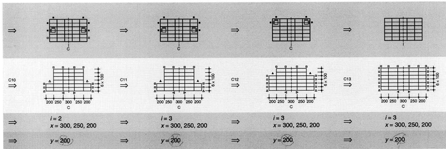
Figure 19b. Derivation of a plan with x = (300, 250, 200) and y = 100 (stage C), continued.
