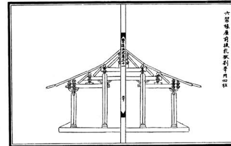
A 6-rafter building, a 2-rafter beam in front and back, with 4 columns. 6- jia chuan wu , qian hou rufu , yong 4 zhu .
