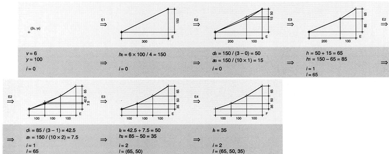
Figure 25. Derivation of a roof section with v = 6 and y = 100 (stage E).
