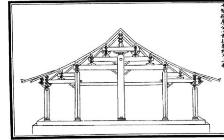
A 10-rafter building, centrally divided, 2-rafter beam in front and back, with 5 columns. 10- jia chuan wu , fen xin , qian hou rufu , yong 5 zhu .
