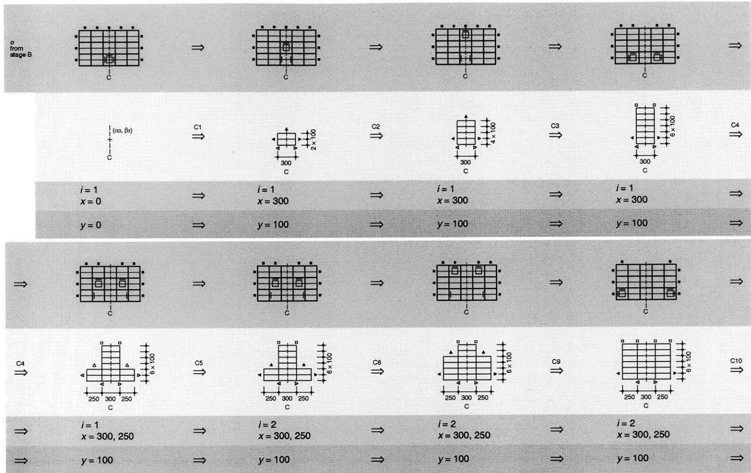
Figure 19a. Derivation of a plan with x = (300, 250, 200) and y = 100 (stage C).
