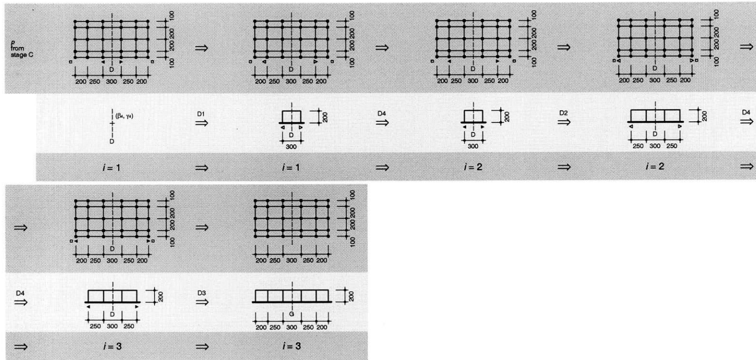
Figure 23. Derivation of a partial elevation with x = (300, 250, 200) and z = 200 (stage D).
