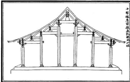
A 10-rafter building, double 2-rafter beams in front and back, with 6 columns. 10- jia chuan wu , qian hou bing rufu , yong 6 zhu .
