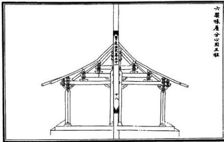
A 6-rafter building, centrally divided, with 3 columns. 6- jia chuan wu , fen xin , yong 3 zhu .
