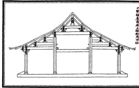
A 10-rafter building, 3-rafter beam in front and back, with 4 columns. 10- jia chuan wu , qian hou 3-chuan fu , yong 4 zhu .
