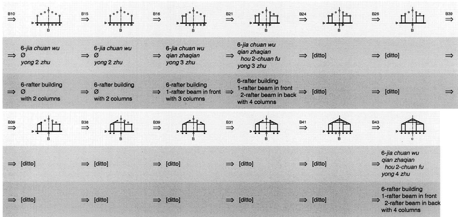
Figure 12. Derivation of a 6-rafter building, 1-rafter beam in front, 2-rafter beam in back, with 4 columns (stage B).
