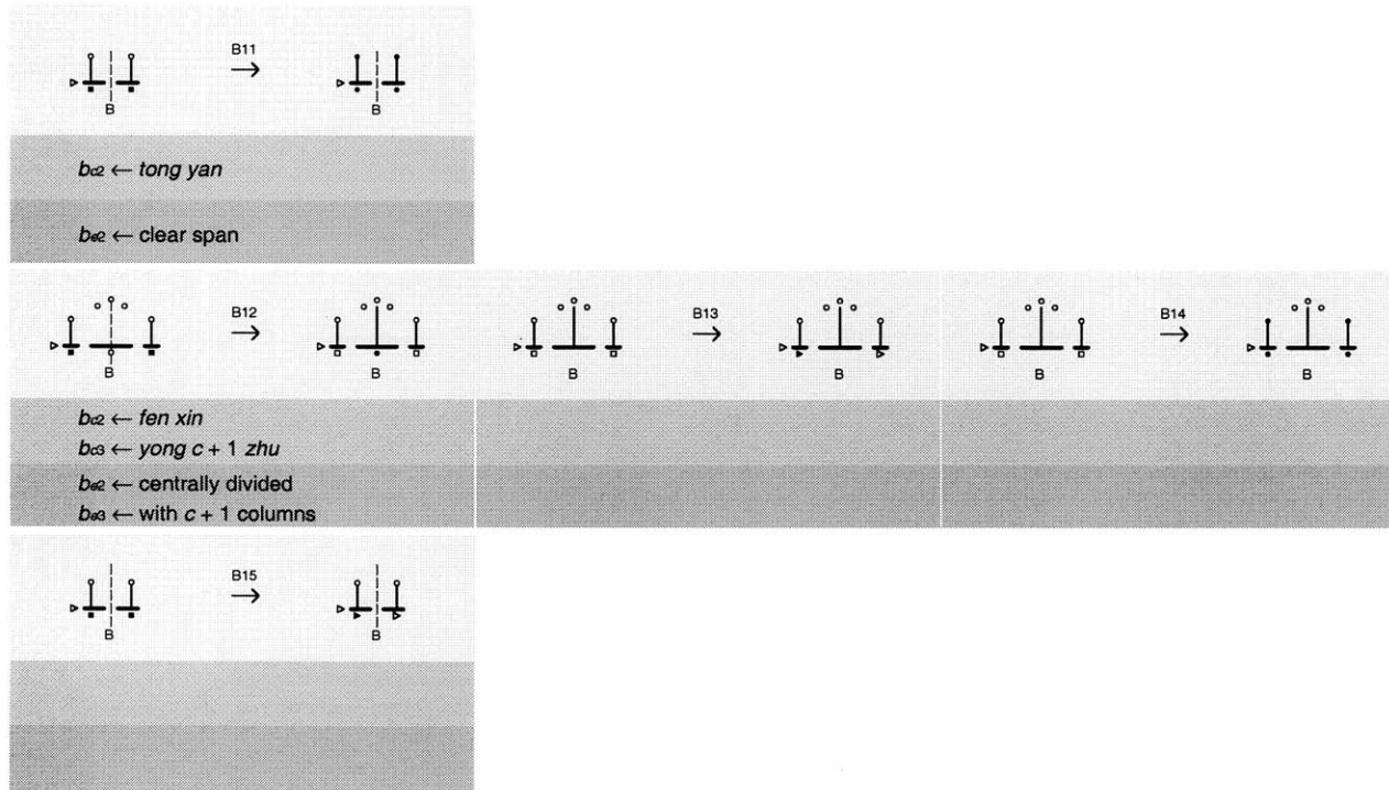
Figure 8a. Schemata for instantiating beams in section diagrams (stage B).
