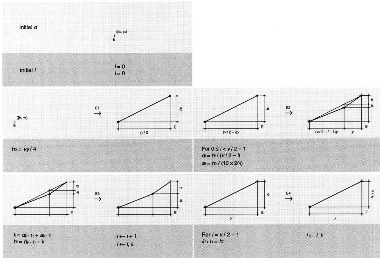
Figure 24. Schemata for generating the roof section, juzhe (stage E).
