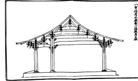
An 8-rafter building, 2-rafter beam in front, 6-rafter beam in back, with 3 columns. 8- jia chuan wu , rufu dui 6-chuan fu , yong 3 zhu .
