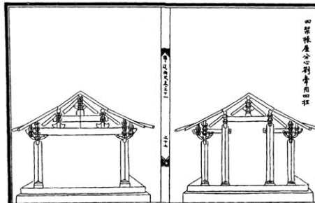
Left [description assumed]. A 4-rafter building, clear span, with 2 columns. 4- jia chuan wu , tongyan , yong 2 zhu . Right. A 4-rafter building, centrally divided, a 1-rafter beam, with 4 columns. 4- jia chuan wu , fen xin , zhaqian , yong 4 zhu . [The description is wrong. For centrally divided, fen xin , read in front and back, qian hou .]
