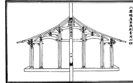
An 8-rafter building, 1-rafter beam [and 2-rafter beam] in front and back, with 6 columns. 8- jia chuan wu , qian hou zhaqian [rufu] , yong 6 zhu .
