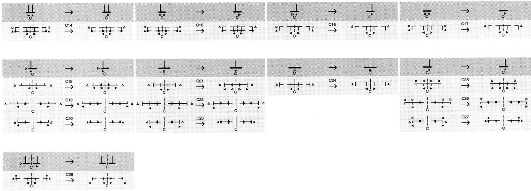
Figure 18. Schemata for instantiating the disposition of beams in plans (stage C).
