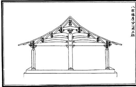
An 8-rafter building, centrally divided, with 3 columns. 8- jia chuan wu , fen xin , yong 3 zhu .
