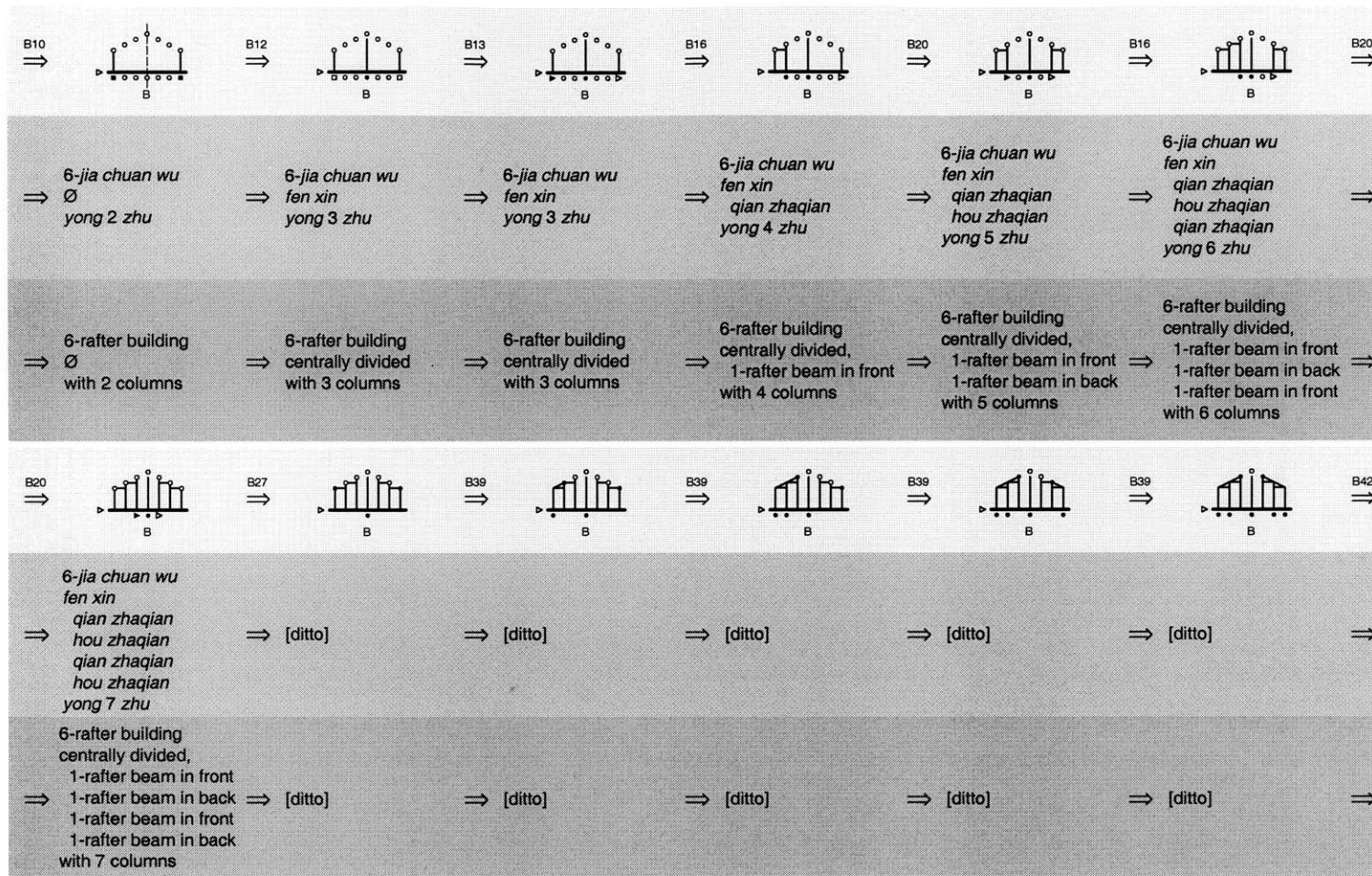
Figure 11a. Derivation of a 6-rafter building, centrally divided, with a double 1-rafter beam in front and back (stage B). This section diagram is probably illegal.
