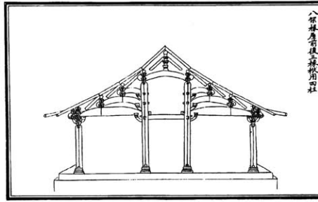
An 8-rafter building, a 3-rafter beam in front and back, with 4 columns. 8- jia chuan wu , qian hou 3-chuan fu , yong 4 zhu .
