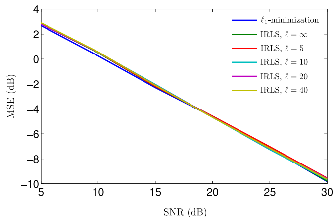
Fig. 3. Mean square error ( 20 \log_{10} \|\bar{x} - x\|_2 ) as a function of \ell and SNR, for \nu = 1/2 and \epsilon(5) = 10^{-4} . This figure highlights the sparsifying properties of f_\nu(\cdot) -minimization by IRLS for \nu < 1 . As in the previous figure, only a few number of IRLS iterations are required to reach a satisfactory value of the MSE.
