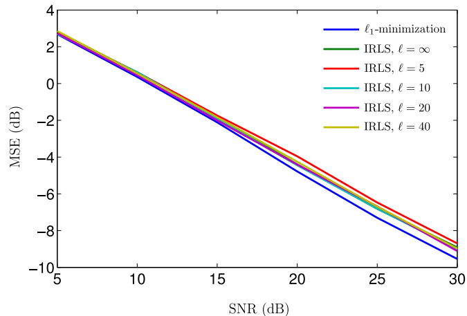
Fig. 2. Mean square error ( 20 \log_{10} \|\bar{x} - x\|_2 ) as a function of \ell and SNR, for \nu = 1 and \epsilon(5) = 10^{-4} . The figure shows that the stability of IRLS compares favorably to that of \ell_1 -minimization. More importantly, only a few number of IRLS iterations are required to reach a satisfactory value of the MSE.
