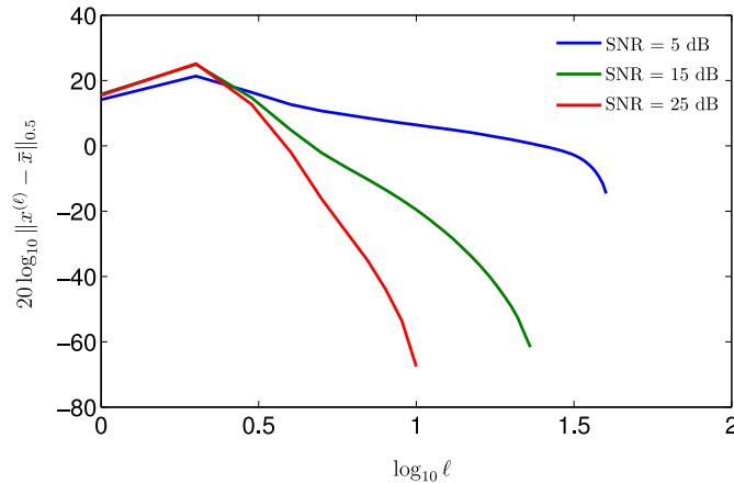
Fig. 8. 20 \log_{10} \|x^{(\ell)} - \bar{x}\|_{0.5} as a function of \log_{10} \ell and SNR, for \nu = 0.5 and fixed \epsilon = 10^{-4} . The figure shows that the IRLS converges with a relatively small number of iterations ( \ell ).
