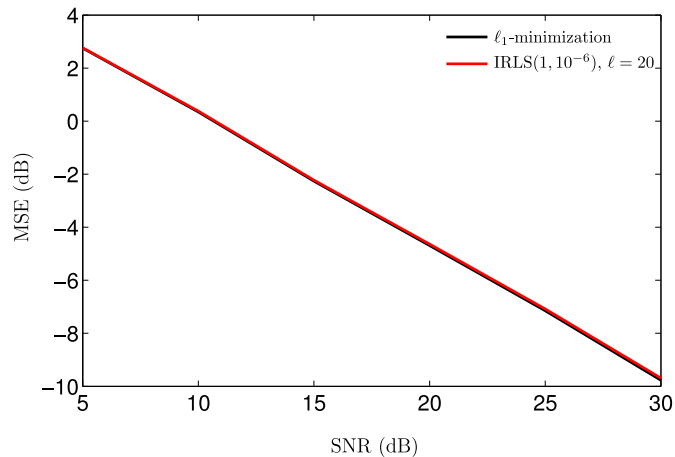
Fig. 4. Mean square error ( 20 \log_{10} \|\bar{x} - x\|_2 ) as a function of \ell and SNR, for \nu = 1 and \epsilon(5) = 10^{-6} . The figure shows that, as one decreases \epsilon , the approximation to the \ell_1 -norm improves.
