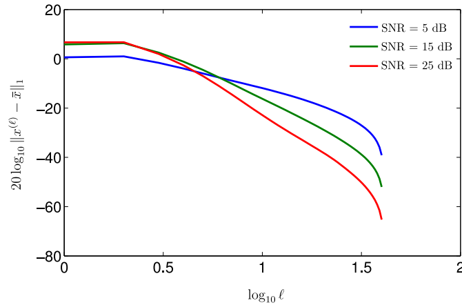
Fig. 6. 20 \log_{10} \|x^{(\ell)} - \bar{x}\|_1 as a function of \log_{10} \ell and SNR, for \nu = 1 and fixed \epsilon(5) = 10^{-4} . The figure shows that the IRLS converges with a relatively small number of iterations ( \ell ).
