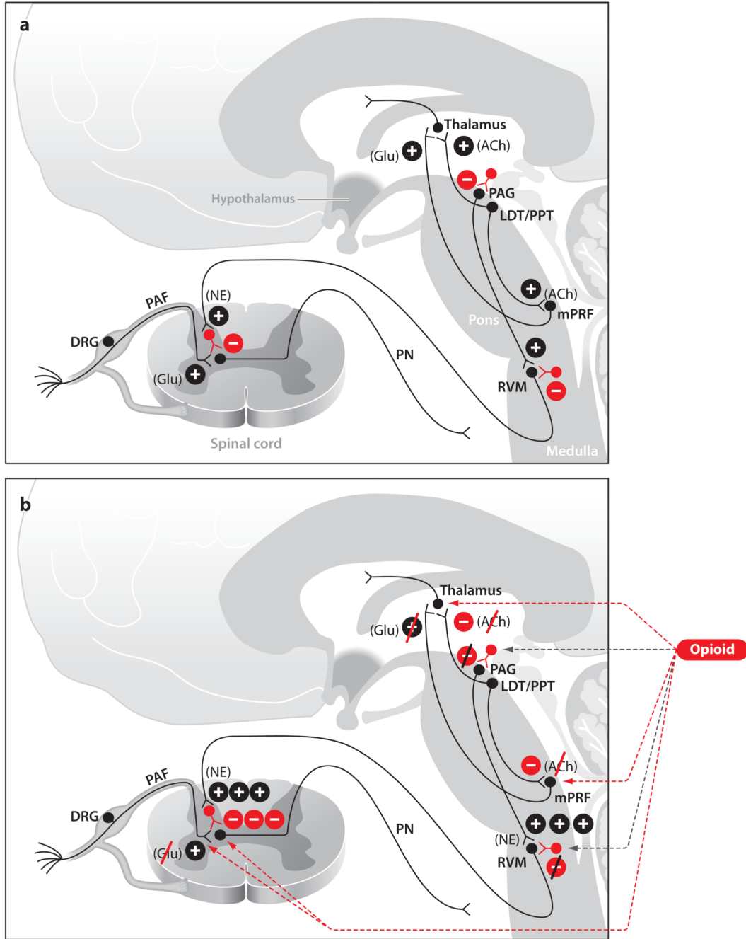
Figure 3. Sites of opioid receptor effects during the awake state (a) and during opioid administration (b). (a) Normal cholinergic signaling during wakefulness and normal nociceptive signaling from the spinal cord to brain stem. (b) Illustrates opioid-induced decrease in arousal through a decrease in cholinergic signaling and the mechanisms of opioid-induced analgesia. Abbreviations: ACh, acetylcholine; DRG, dorsal root ganglia; Glu, glutamate; LDT, laterodorsal tegmental area; mPRF, medial pontine reticular formation; NE, norepinephrine; PAF, peripheral afferent fiber; PAG, periaqueductal gray; PN, projection neuron; PPT, pedunclopontine tegmental area; RVM, rostral ventral medulla.
