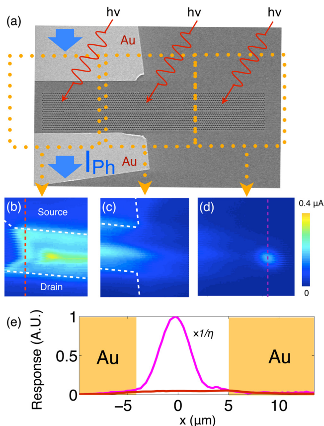
FIG. 3. (a) SEM image of the graphene detector on the PPC cavity. Scale bar: 3 \mu m . (b)–(d) Spatial mapping of the photocurrent at the three areas indicated in (a). The white dashed lines show the boundary of the metal contacts. (e) The trace of photocurrent data in (b) and (d), showing the comparison of the photocurrent with (magenta) and without (red) coupled to the PPC cavity. The trace across the coupler of the PPC cavity is normalized to the coupling efficiency \eta , and the edge of the metal are labeled by the yellow shaded region.
