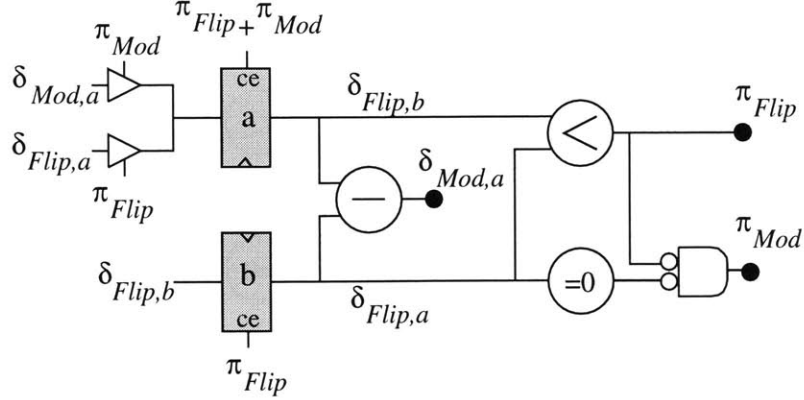
Figure 2-2: Circuit for computing Gcd(a, b) .
