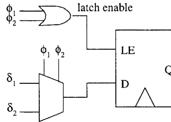
Figure 3-4: Circuits for merging two transitions' actions on the same register.
