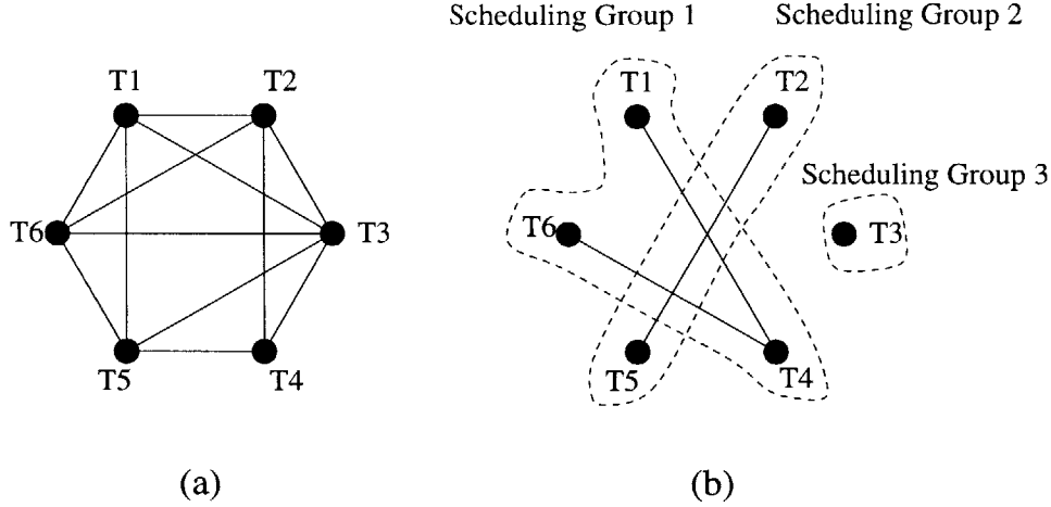
Figure 3-6: Scheduling conflict-free rules: (a) \langle \rangle_{CF} graph (b) Corresponding conflict graph and its connected components.
