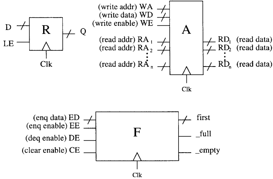
Figure 3-2: Synchronous state elements.
