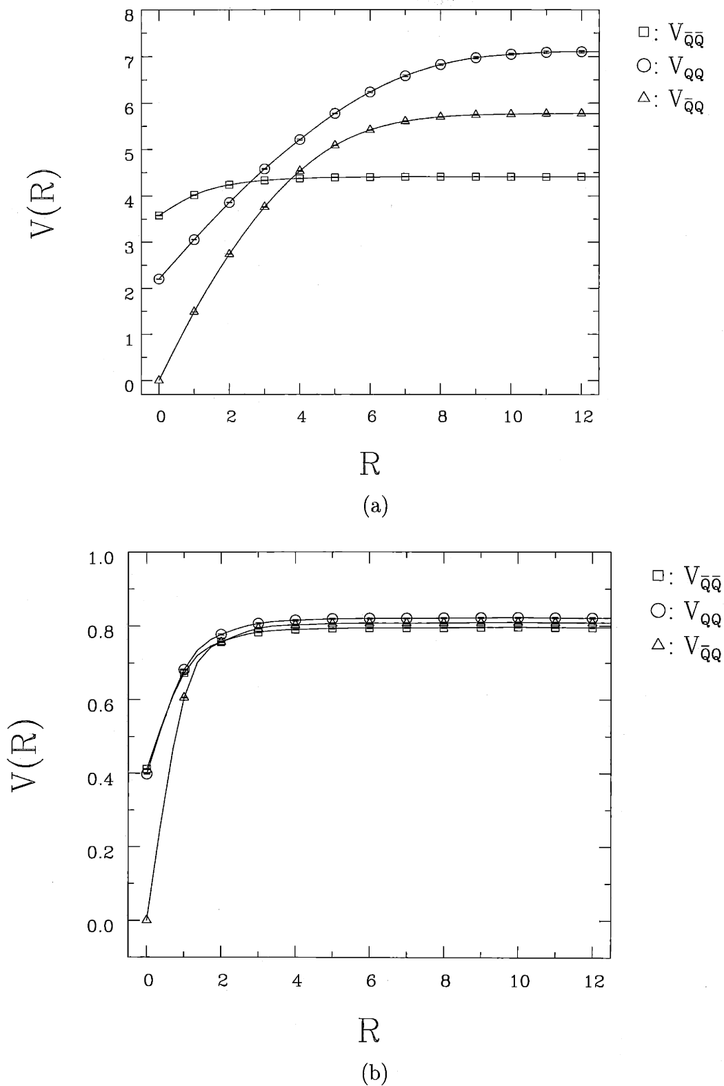
Figure 3-2: The static quark-anti-quark, quark-quark and anti-quark-anti-quark potentials (a) on the confined side (at h = 0.01, \kappa = 0.50 ) and (b) on the deconfined side (at h = 0.01 and \kappa = 0.56 ) of the crossover.
