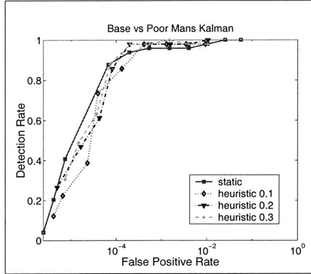
Figure 6-4: ROC curves for the static and Poor Man’s Kalman detection systems. The numbers associated with each PMK curve indicates the tolerance for persevering detections.
