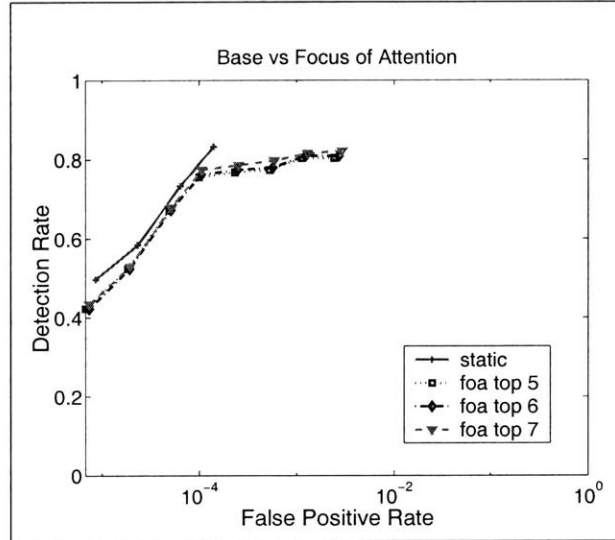
Figure 5-6: ROC curves for people detection comparing the base system to one that preprocess an image by focusing attention on certain salient regions in the image.
