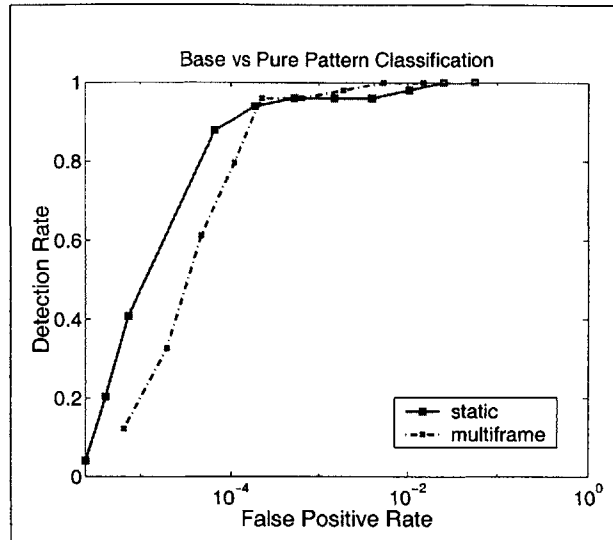
Figure 6-2: ROC curves for the static and pure pattern classification detection systems. The detection rate is plotted against the false positive rate, measured on a logarithmic scale. The false positive rate is defined as the number of false detections per inspected window.
