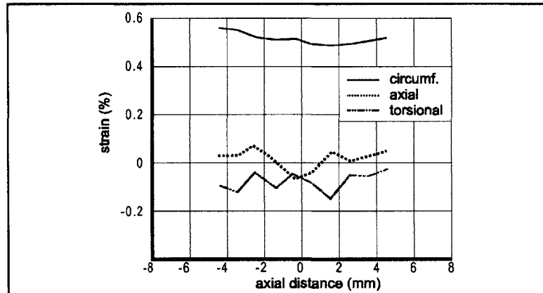
Figure 3.5: The spatially varying arterial surface strain tensor at a balloon pressure of 8 atm. The artery is substantially uniformly expanded circumferentially. Negligible torsion is present.
