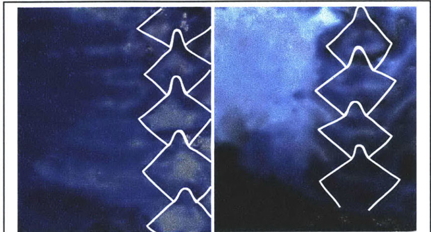
Figure 3.11: En face preparation of arterial section stented with conventional stent (left) and variable geometry stent (right) and stained with Evan's Blue. The stent image is highlighted. Light blue regions indicate areas of intact endothelium; dark blue regions such as the expanse to the left of the stent in the left panel show areas where the endothelial layer has been denuded exposing the basement membrane. Marks that appear to have been scraped appear in the left panel.
