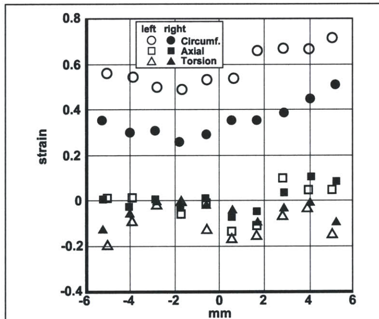
Figure 2.10: The system can measure strains in an in vivo environment. Here strains are shown generated in two rabbit femoral arteries by 3 mm stents mounted on balloon catheters pressurized to 4 atm. The end-first opening characteristic can be clearly seen, accompanied by slight axial shortening and relatively minor torsion, similar to that seen in vitro at similar pressures.
