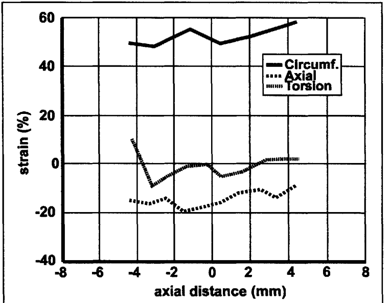
Figure 2.7: Arterial surface strain tensor components after in vitro stent expansion to 8 atm. The stent's middle region has expanded and circumferential strain is now evenly distributed along the length of the stent. Notice the degree of axial contraction that has occurred as the center expanded.
