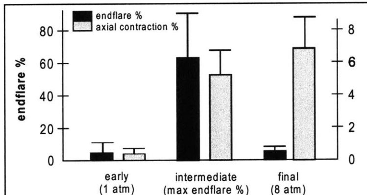
Figure 3.6: The progression of endflare and excess axial strain in the circumferentially expanding stent. The dogbone-like shape introduced by end-first expansion is a transient effect, however axial contraction of the stent monotonically increases with increasing expansion pressure. Excess axial strain refers to the difference between stent and arterial axial strain.
