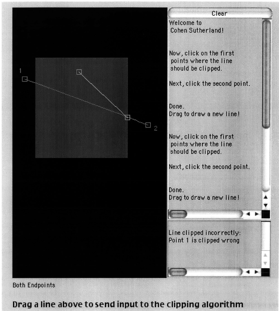
Figure 1-3: The visualization panel allows a student to explore the inner workings of an algorithm
