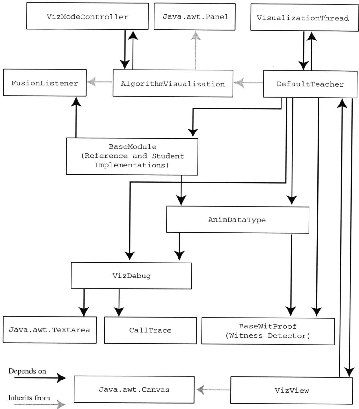
Figure 4-2: Module Dependency Diagram for Visualization Panel.
