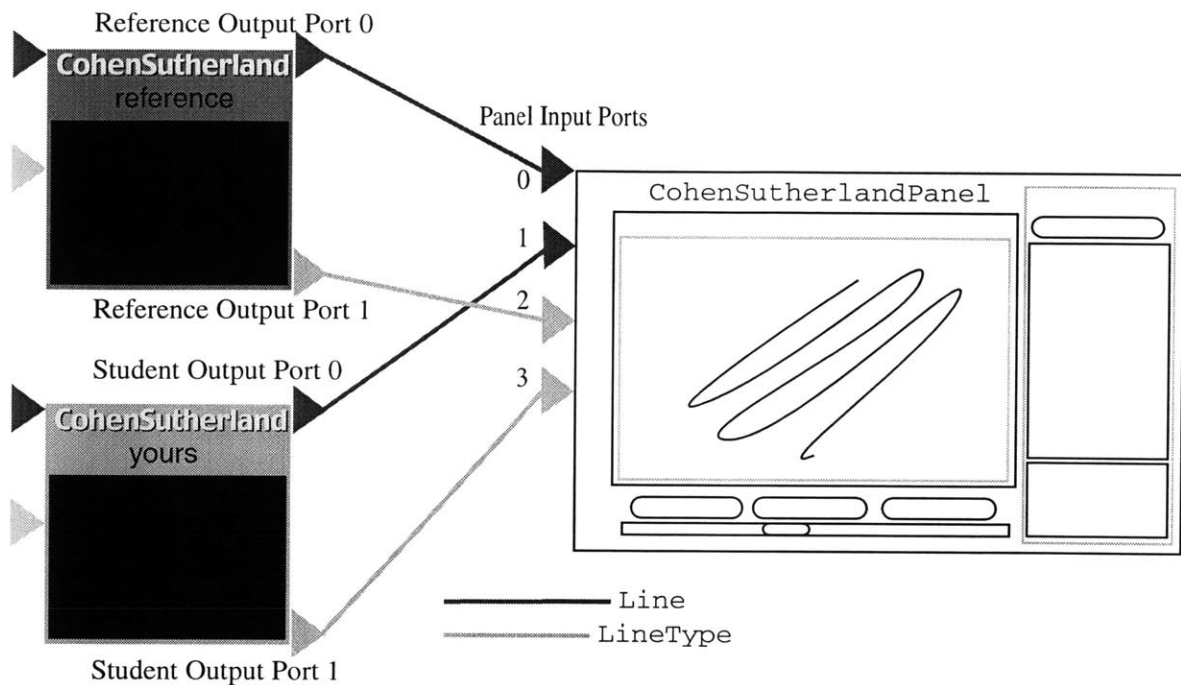
Figure 4-4: A pseudo-concept graph, displaying links from modules to visualization panels
