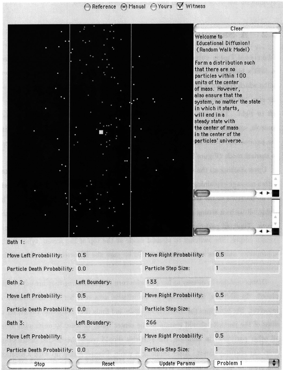
Figure 5-1: An Educational Fusion simulation of random walk diffusion
