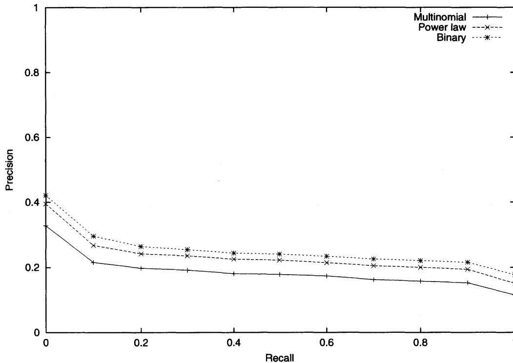
Figure 5-7: Learning from the correct distribution.
