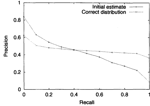
(b) Power law model – initial estimate v. correct distribution
