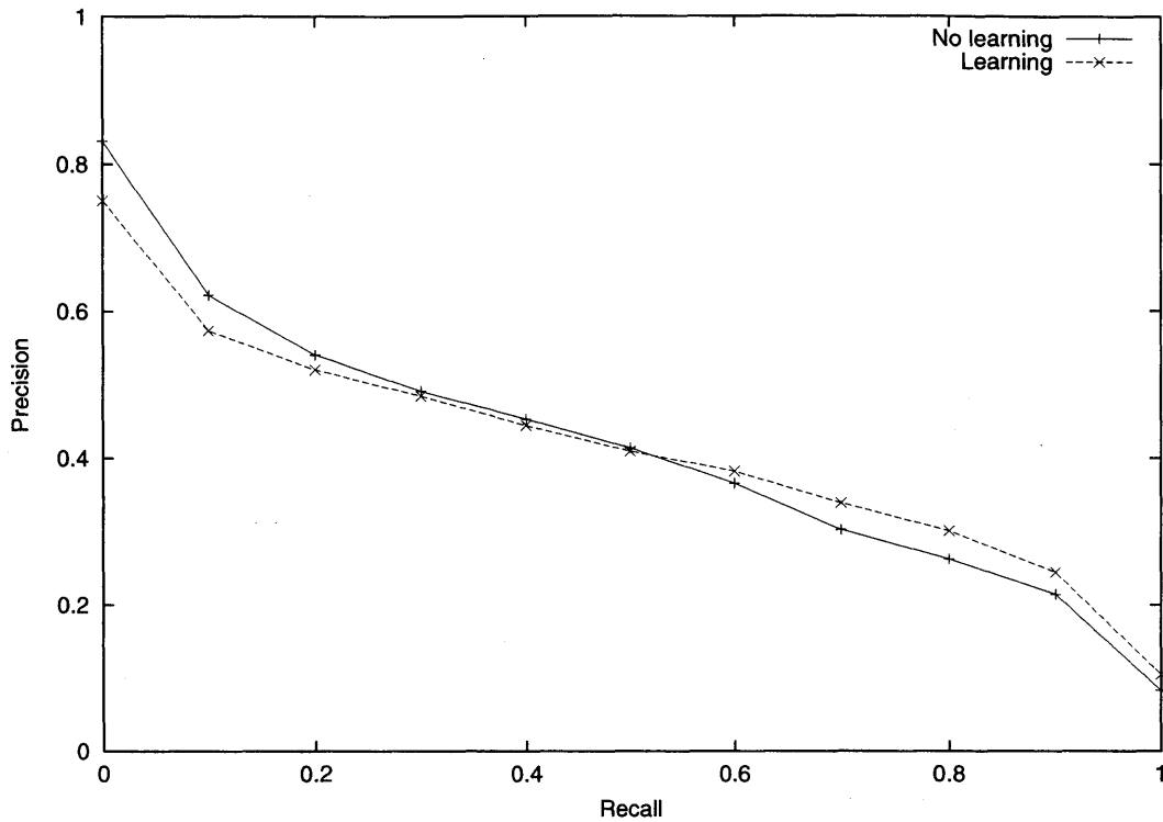
Figure 3-5: Results found using the multinomial model. The relevant distribution is found using learning, with good values for the prior weight and query weight set.
