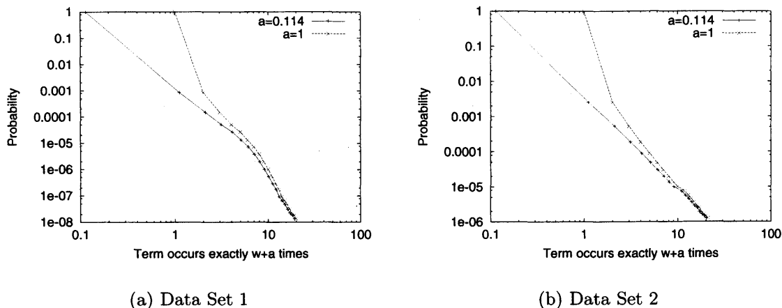
Figure 5-2: The empirical t.o.p.d. for terms in Data Set 1 and 2 shown on a log-log scale, with different values for \alpha . A straight line implies a power law distribution.
