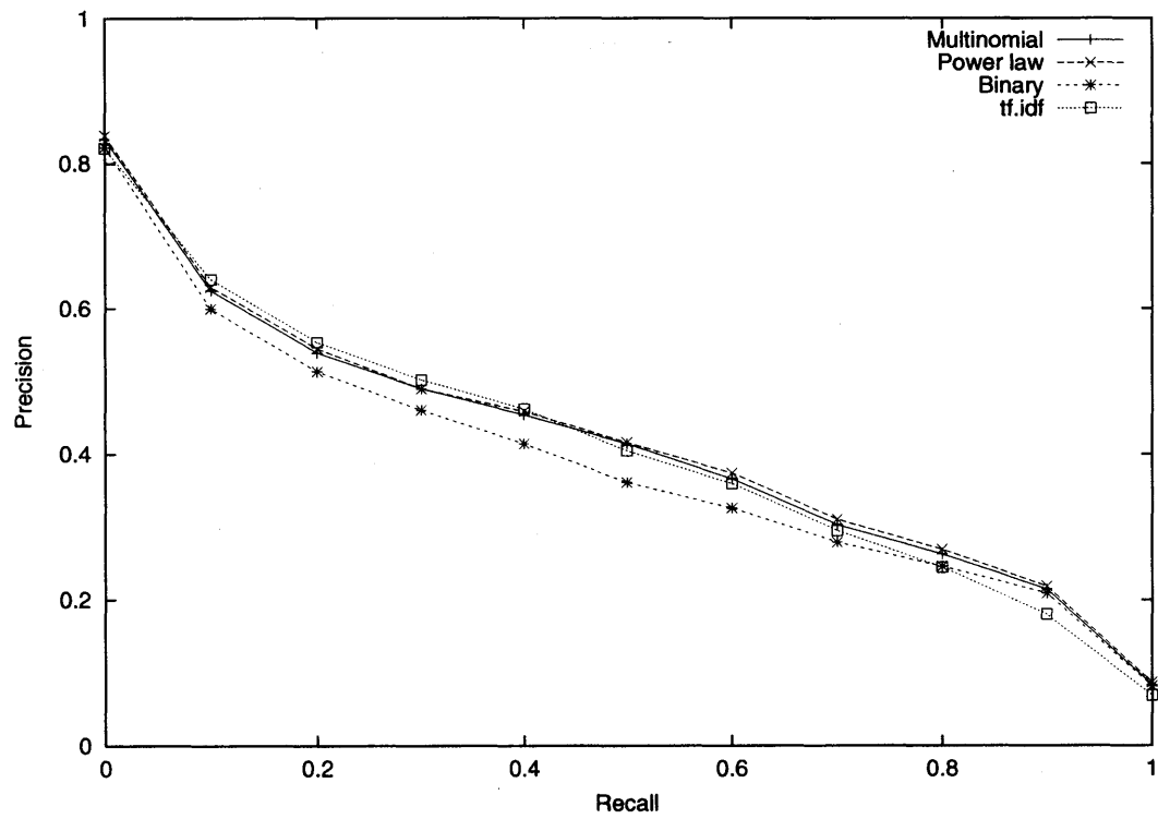
Figure 5-4: Results found using the new models. The relevant distribution used is the initial estimated distribution.
