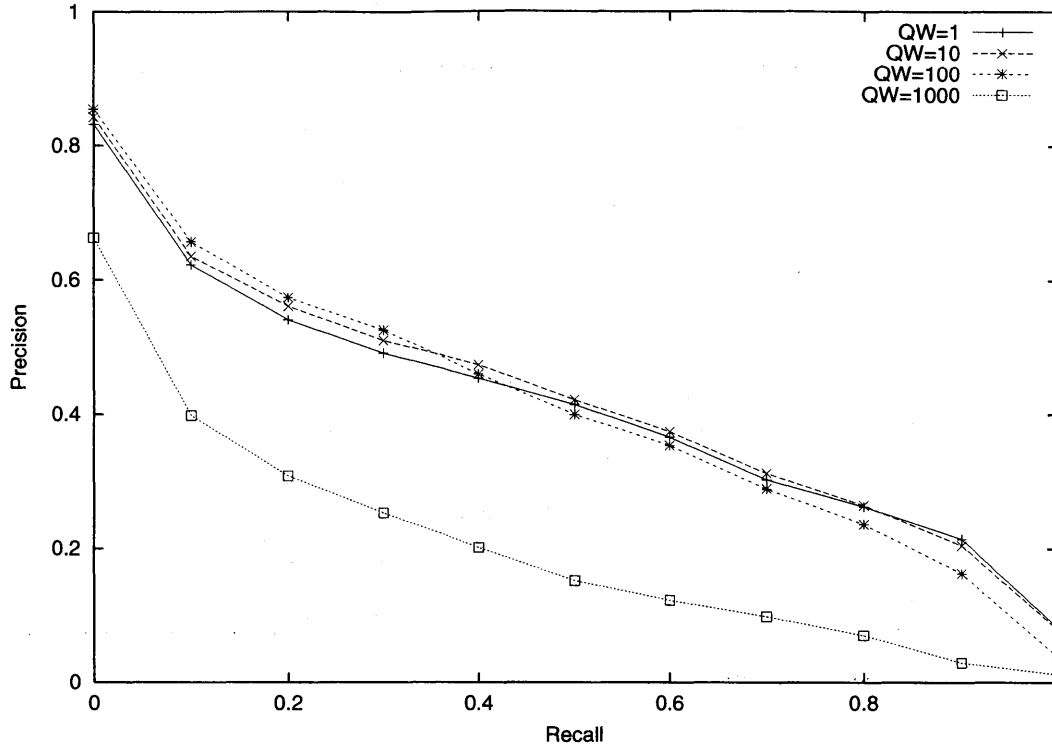
Figure 3-2: Results found using the multinomial model. The relevant distribution is the initial estimated distribution with varying query weights.
