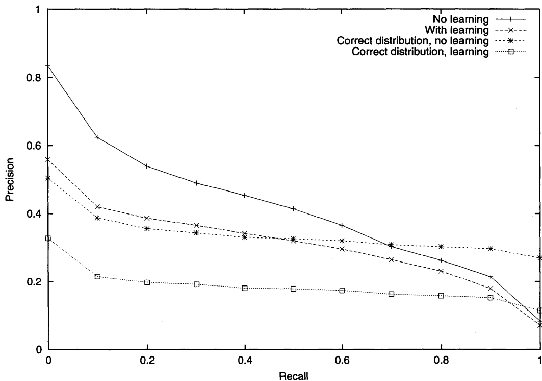
Figure 3-6: Results found using the multinomial model. The relevant distribution is the correct distribution.
