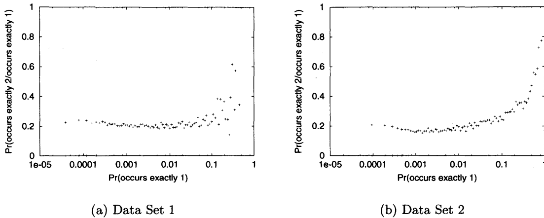
Figure 4-8: Probability of a term occurring once compared with the probability of a term occurring two times.
