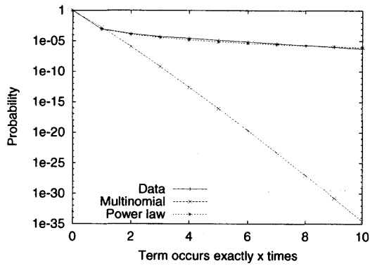
(a) Data Set 1 – with multinomial
