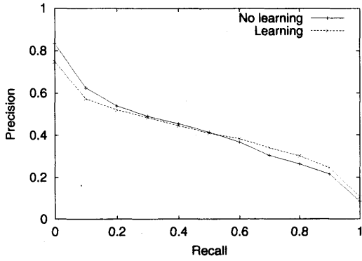
(a) Multinomial model – no learning v. learning
