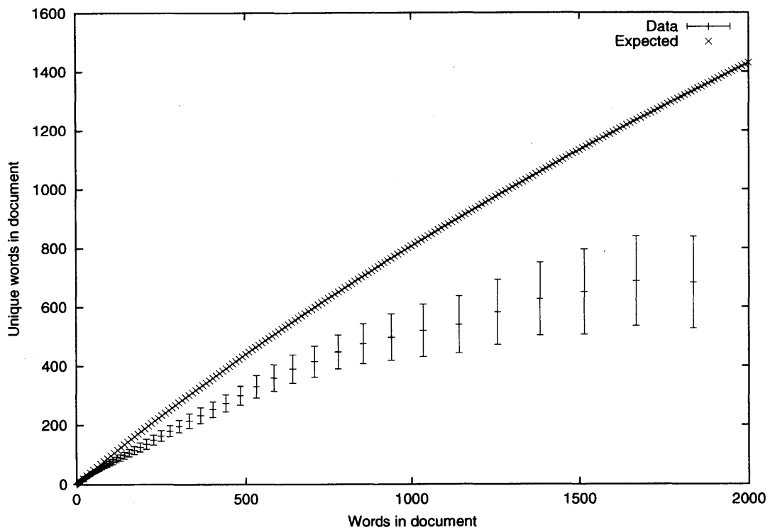
Figure 4-4: Number of unique terms in a document compared with the number of terms in a document. Graph displays empirical values and what is predicted given the multinomial model. For clarity, the empirical data has been binned. Error bars on the empirical data represents the standard deviation within each bin.
