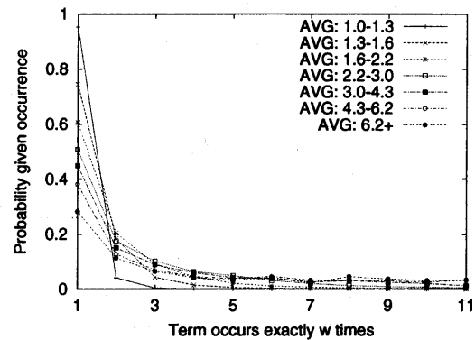
(b) Data Set 2
