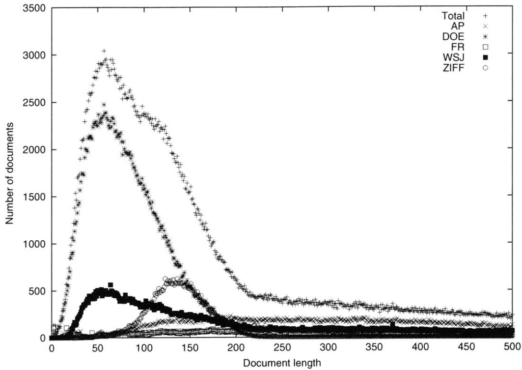
Figure 4-2: The number of documents of length n . Document length displayed by source, and for the corpus as a whole.
