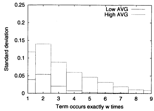
(b) avg – Data Set 1
