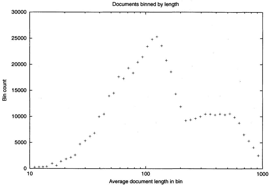
Figure 4-3: The number of documents within a bin. Each bin represents a document length range. The length range of a bin grows exponentially to keep the relative variation within a bin similar.
