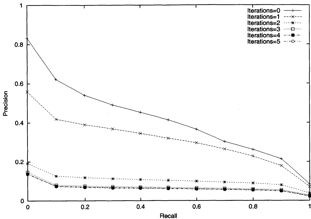
Figure 3-3: Results found using the multinomial model. The relevant distribution is found using learning. Results are compared for different number of iterations during the learning process.
