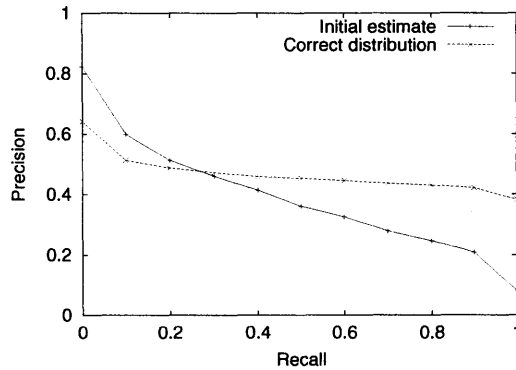
(c) Binary model – initial estimate v. correct distribution
