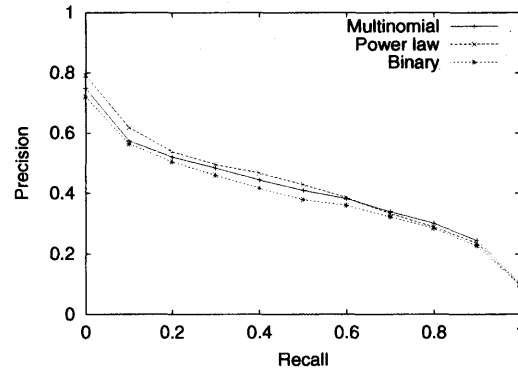
(d) Comparison of learning across models
