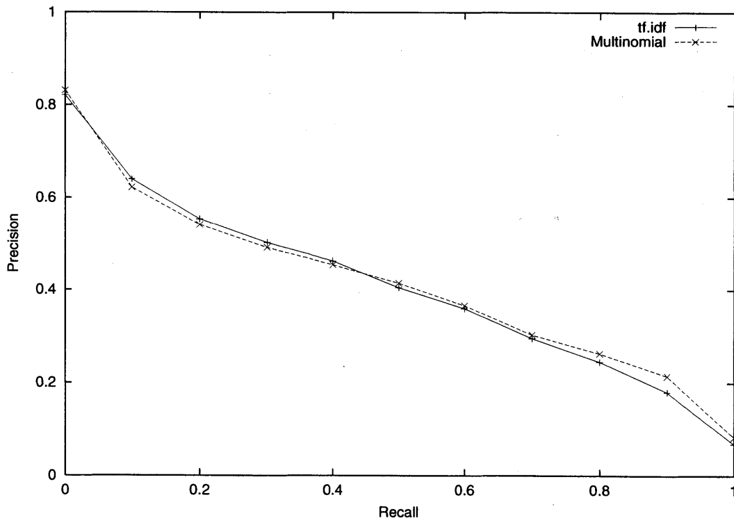
Figure 3-1: Results found using the multinomial model. The relevant distribution used is the initial estimated distribution. Results are compared with tf.idf.
