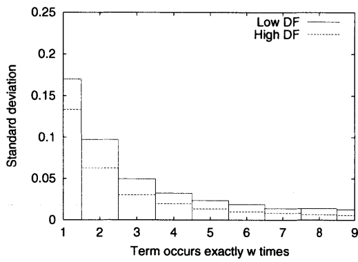
(c) df – Data Set 2
