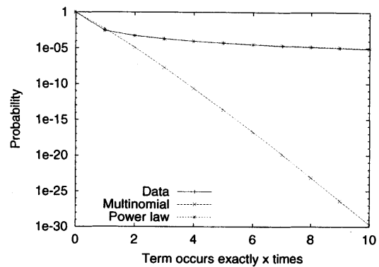
(b) Data Set 2 – with multinomial
