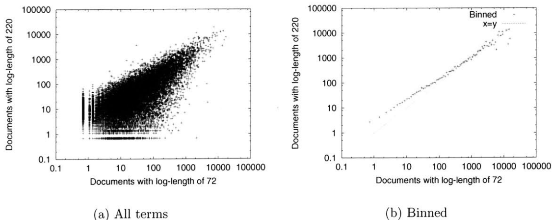
Figure 5-3: The average value of \log(1 + \omega) for a term when it appears in documents of two different log lengths. Although the relationship is reasonably close to linear, it is not actually linear.
