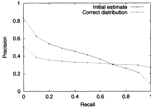
(a) Multinomial model – initial estimate v. correct distribution
