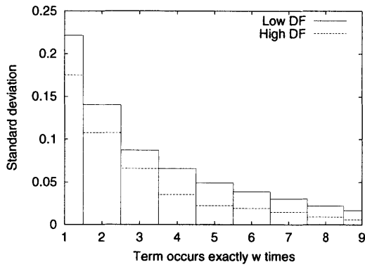
(a) df – Data Set 1
