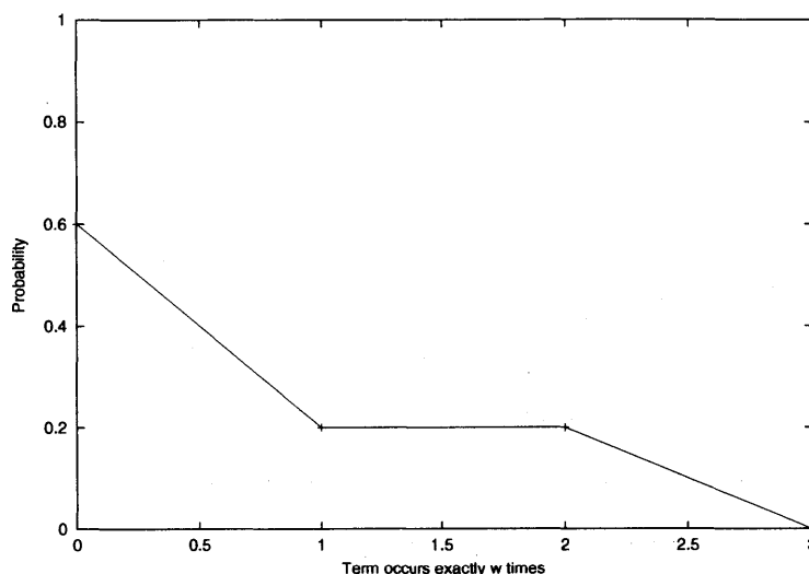
Figure 4-1: An example t.o.p.d. for the term “granny” in our example corpus. By looking at a term’s empirical t.o.p.d. we hope to be able to find the underlying hidden parameter we assume describes the term’s occurrence.
