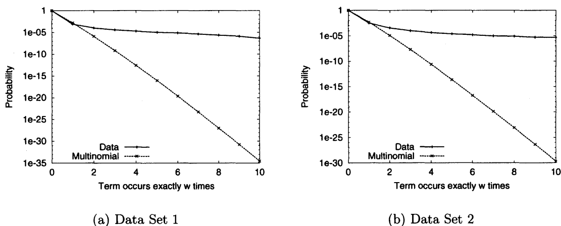
Figure 4-5: The empirical t.o.p.d. for terms compared with what is expected from the multinomial model. Terms occurrence appears to be more clustered than expected.
