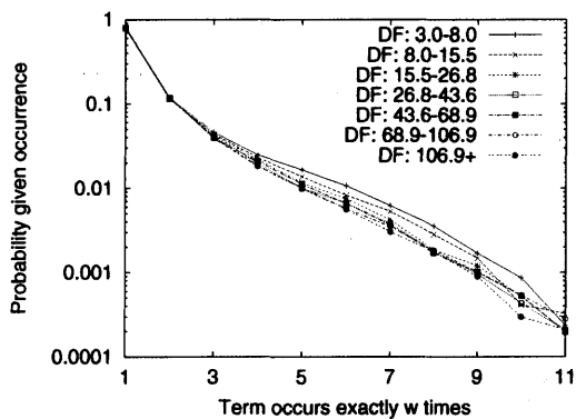
(c) Data Set 1 - Log scale
