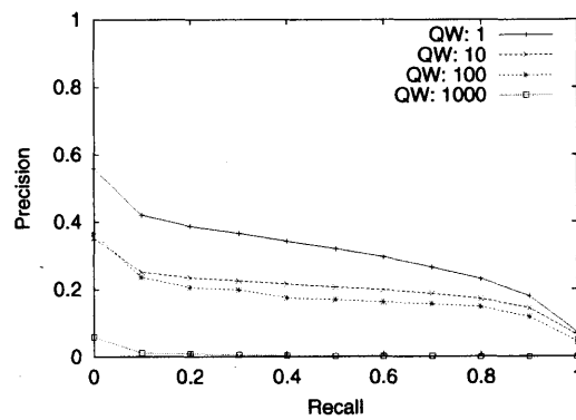
(b) Changing query weight
