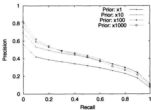
(a) Changing prior knowledge weight
