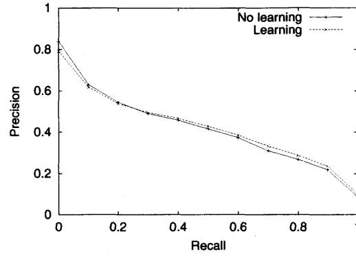
(b) Power law model – no learning v. learning
