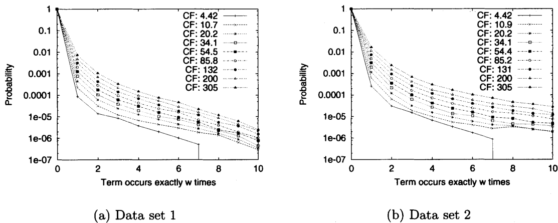
Figure 4-6: The t.o.p.d. for terms with different corpus frequencies.
