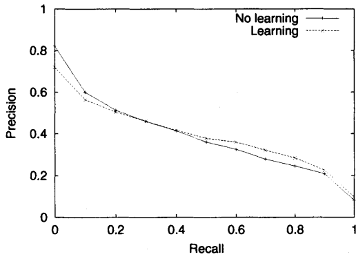
(c) Binary model – no learning v. learning
