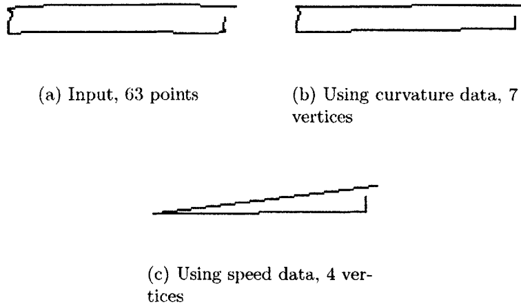
Figure 4-1: Average based filtering using speed data misses a vertex. The curvature fit detects the missed point (along with vertices corresponding to the artifact along the short edge of the rectangle on the left).
