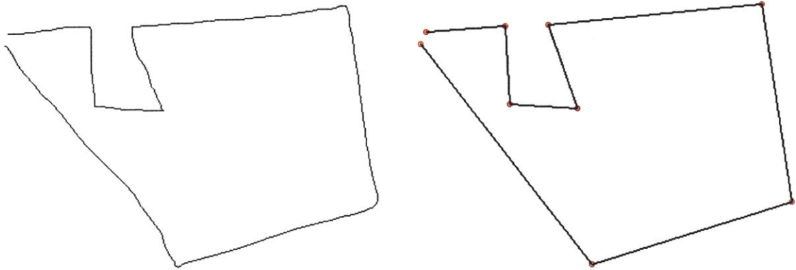
Figure 3-13: The input stroke (on the left) and the features detected by looking at the scale space of the curvature (on the right).
