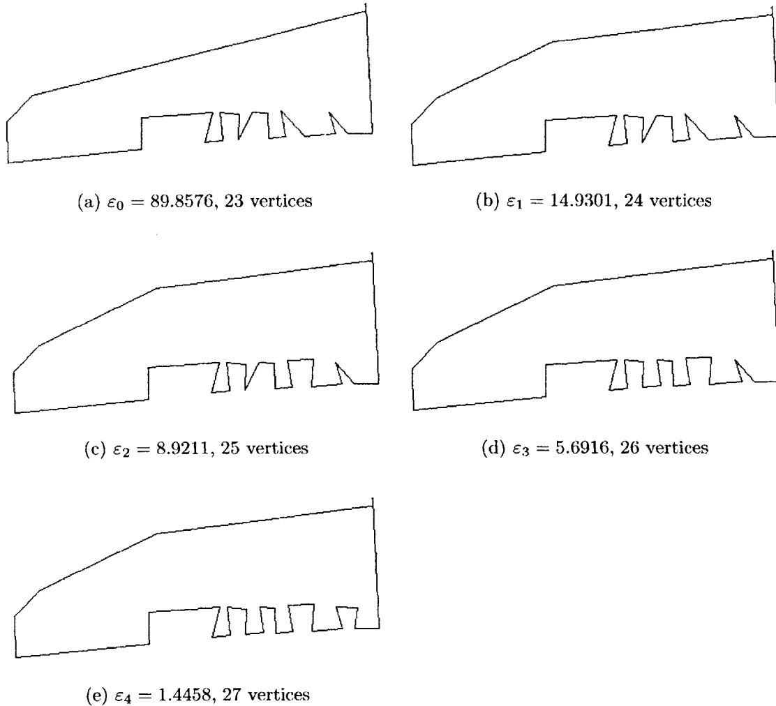
Figure 4-5: The series of hybrid fits generated for the complex stroke in Fig. 4-4. The fits successively get better.
