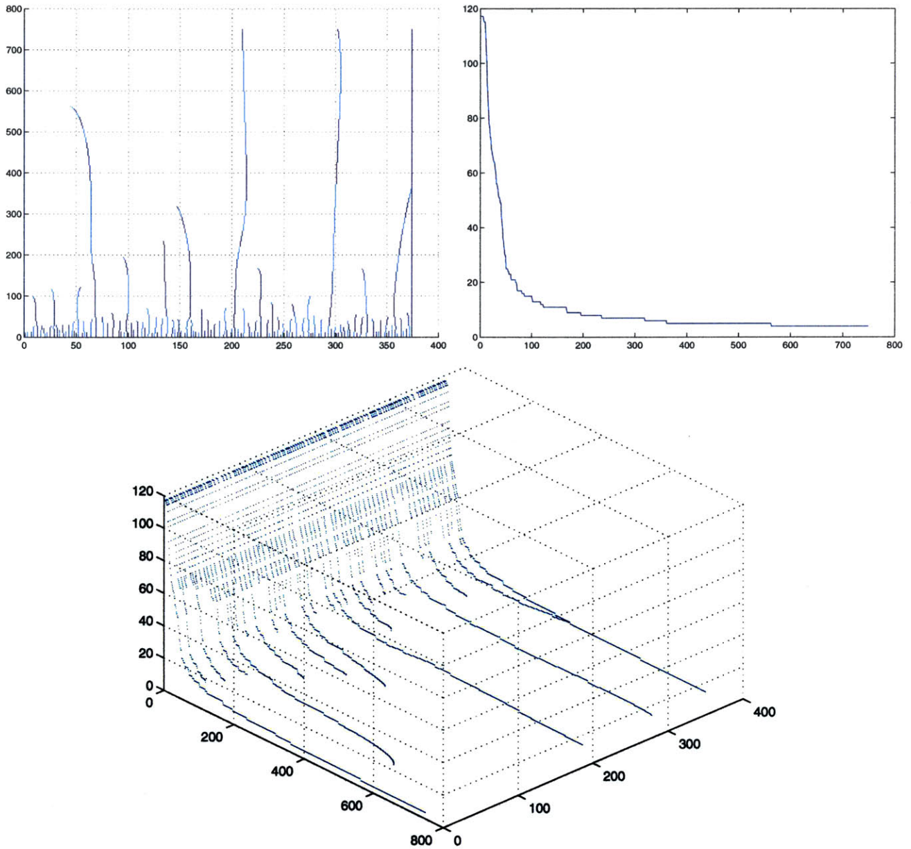
Figure 3-20: The scale-space, feature-count and joint graphs for the speed data of the stroke in Fig.3-14. In this case, the scale selected by our algorithm is 72.
