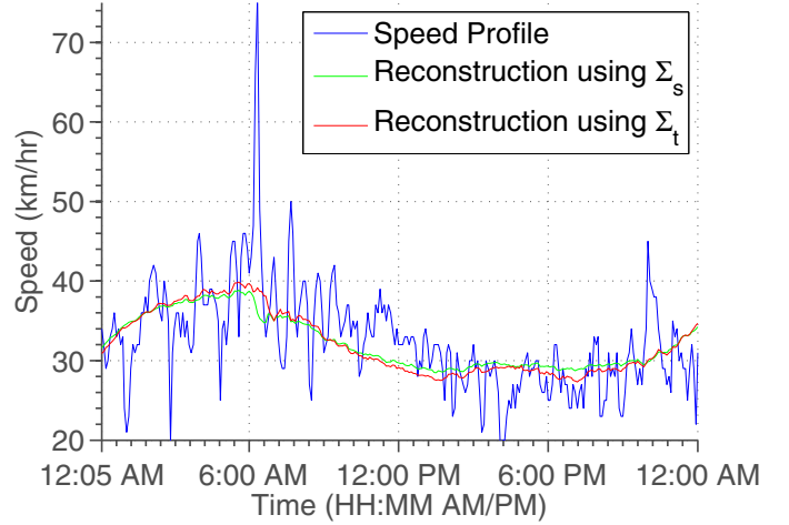
Fig. 6: Data reconstruction for a typical link, using just the 1 st principal components obtained from \Sigma_s and \Sigma_t . Principal components corresponding to basis vectors \phi_{s1} and \phi_{t1} provide similar performance.
