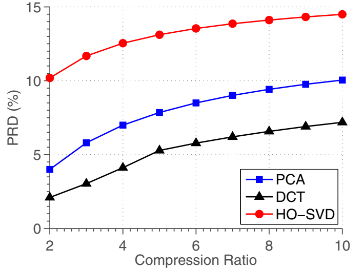
Fig. 9: Compression efficiency of different techniques.
