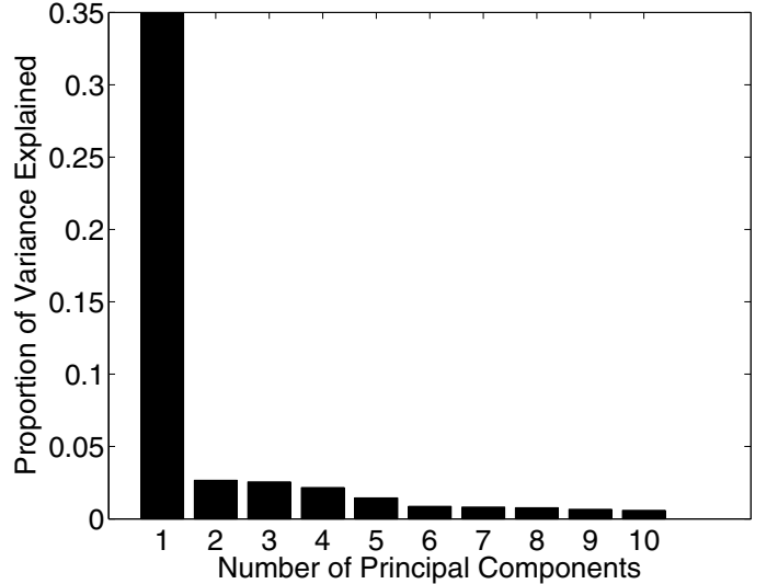
Fig. 7: Proportion of variance in \Sigma_s explained by principal components.
