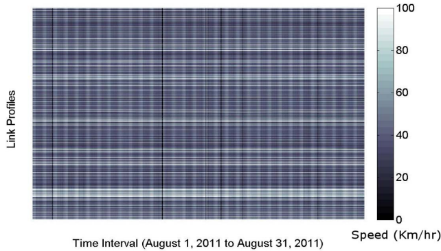
Fig. 3: Reconstructed speed profiles of links in \mathbf{X}_G^T using DCT compression. Color bar represents colors corresponding to different speed values.
