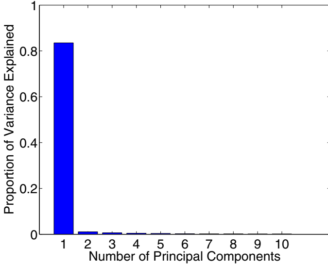
Fig. 8: Proportion of variance in \Sigma_t explained by principal components.
