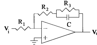
Fig. 6. Loop filter structure for the prototype system. C = 0.68 \mu\text{F} , R_1 = 90.9 \text{ k}\Omega , R_2 = 10 \text{ k}\Omega , and R_3 = 10 \text{ M}\Omega .
