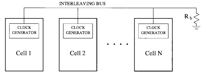
Fig. 5. The distributed interleaving approach.
