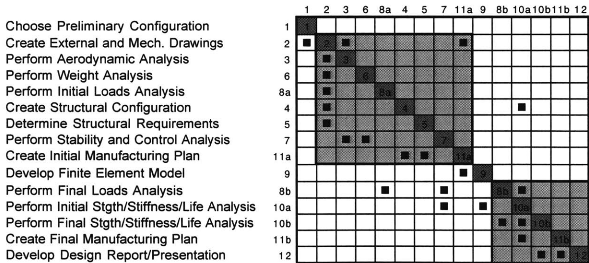
Figure 39. Improved DSM: Heuristics 1-7
