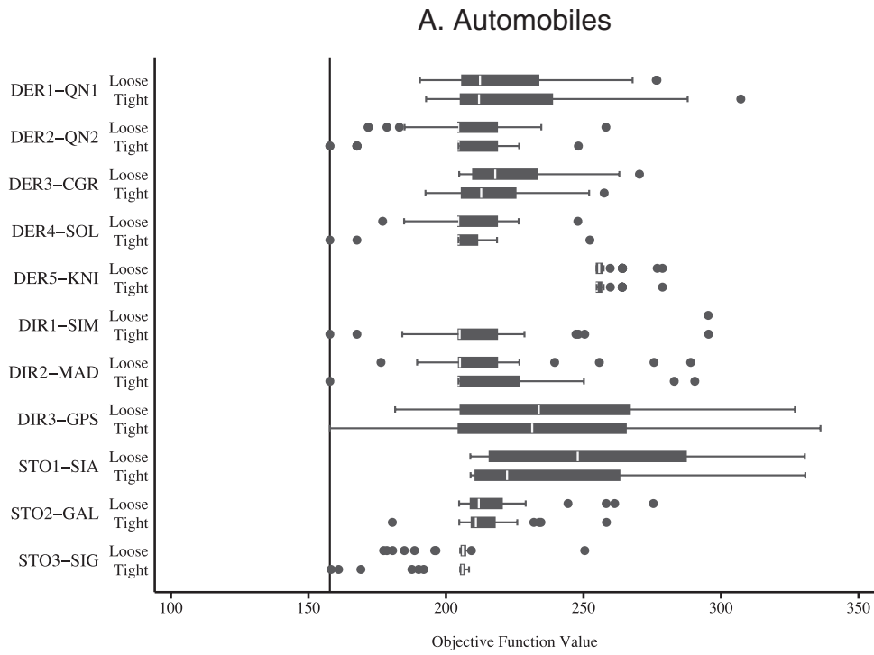
FIGURE 1.—BOX-AND-WHISKER PLOTS OF THE OBJECTIVE FUNCTION VALUE
