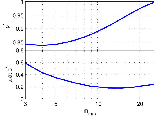
Figure 11: Asymptotic model p^* values for different split designs w satisfying c_A = 2.5 , for the 4-SFPA on the B -side. In the split designs, node degrees are either one or approximately m_{max} .
