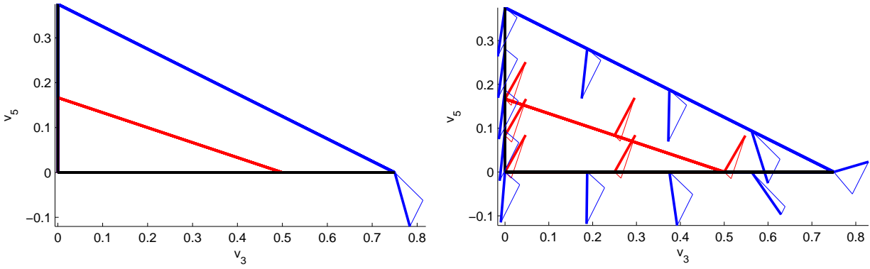
Figure 5: The linear (left) and nonlinear (right) gradients and their projections onto the active planes, for c_A = 3.5 . The polytope is viewed from the along the negative v_4 -axis.
