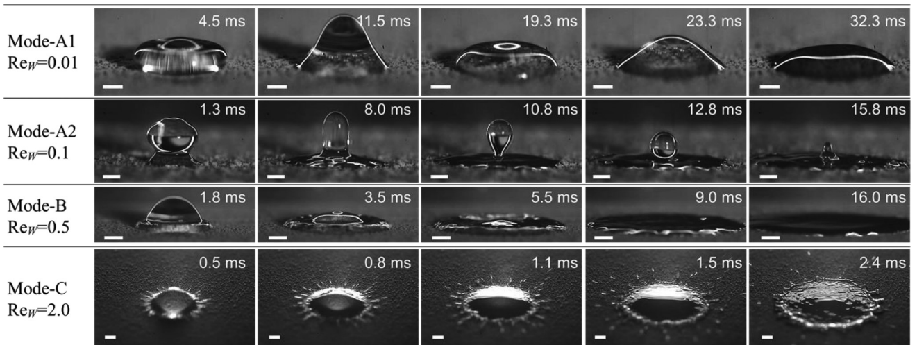
FIG. 2. Droplets show four different impingement modes depending on the Washburn-Reynolds number after impacting highly wetting porous surfaces. The Washburn-Reynolds number can be expressed as Re_W = U_o \rho r_c \cos \theta / \mu , where U_o is the impact velocity, \rho is the liquid density, r_c is the effective capillary radius, \theta is the surface contact angle, and \mu is the liquid viscosity. Mode A1: compressing-oscillating, Mode A2: necking and spreading, Mode B: spreading, and Mode C: radial jetting and spreading (see Supplemental Material [14]). A high-speed camera (Photron) was used to record the behavior of liquid droplets on the surfaces. The scale bar in each image is 1 mm.
