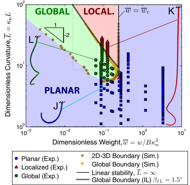
FIG. 3 (color online). Phase diagram for the rod configurations: planar (2D) and nonplanar (3D, global and localized helices). Each experimental data point is plotted on the (\bar{L}, \bar{w}) space, whereas only the phase boundaries are shown for the numerics. Theoretical curves for the planar-to-localized and localized-to-global transitions are superposed on the data. Three experimental reconstructions are shown as insets: (j) planar (blue, \kappa_n = 49.5 \text{ m}^{-1} , L = 10 \text{ cm} ), (k) localized helix (red, \kappa_n = 49.5 \text{ m}^{-1} , L = 40 \text{ cm} ), and (l) global helix (green, \kappa_n = 62.3 \text{ m}^{-1} , L = 20 \text{ cm} ).
