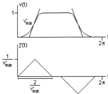
Figure 3.7 Triangular ISF Approximation
