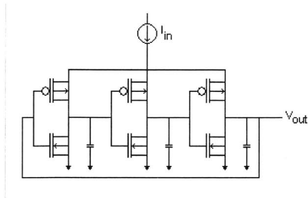
Figure 4.4 Current-Controlled Oscillator
