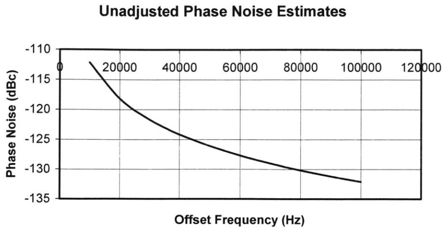
Figure 6.1 Phase Noise Estimates
