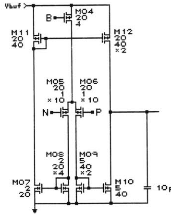
Figure 5.3 Low-Power High-Gain Op-amp
