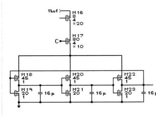
Figure 5.5 ICO with Cascoded Input
