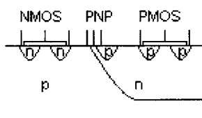
Figure 4.8 PNP Bipolar Transistor on CMOS Process
