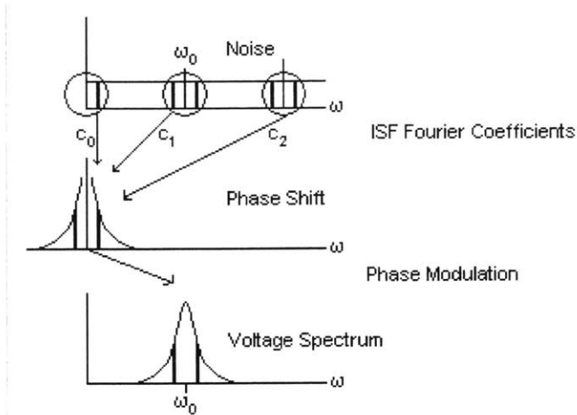
Figure 3.6 Device Noise to Phase Noise Path
