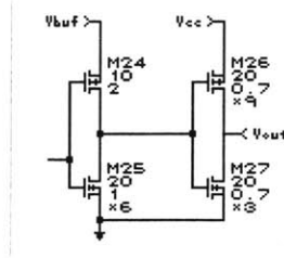
Figure 5.6 Output Buffers
