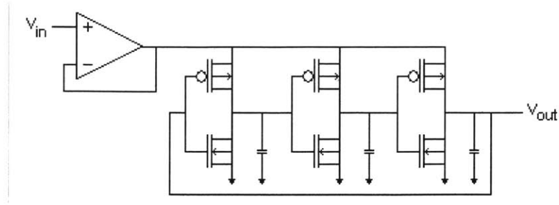
Figure 4.3 Possible Frequency Control Scheme
