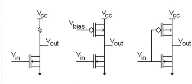
Figure 4.2 Possible Inverters
