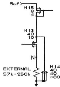
Figure 5.4 Voltage-to-Current Converter and Low-Pass Filter
