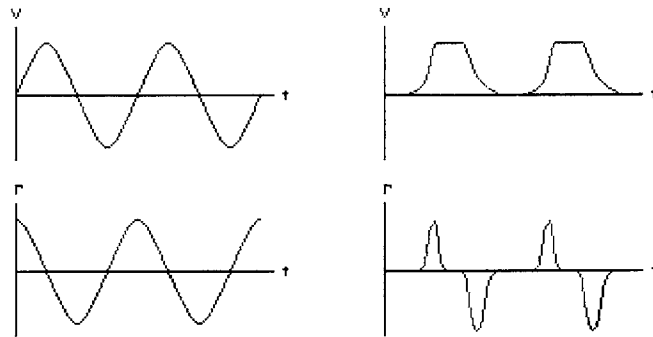
Figure 3.5 ISF's for Possible Oscillators
