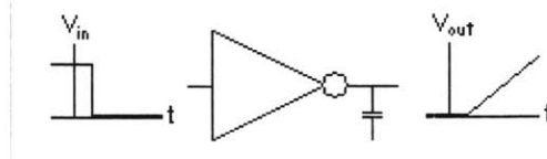
Figure 4.1 Slew-Rate Limited Inverter
