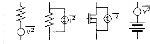
Figure 3.2 Circuit Models for Noisy Devices
