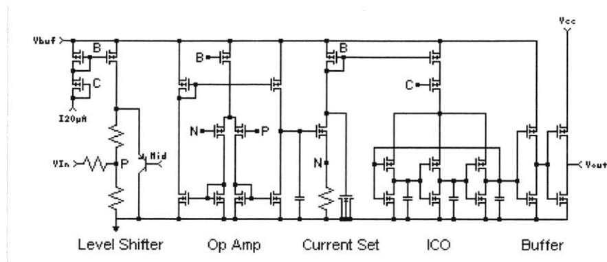
Figure 5.1 Total VCO Schematic
