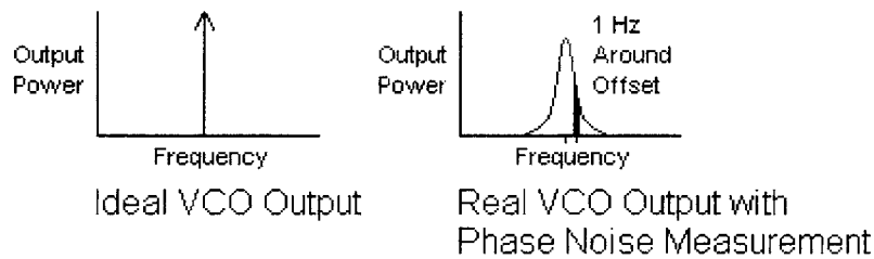
Figure 3.1 Spectral Appearance of Phase Noise
