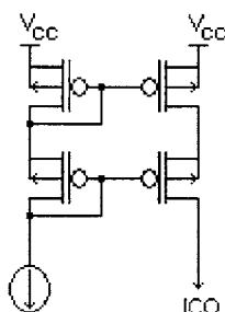
Figure 4.6 Cascode with Rail-Controlled Bias
