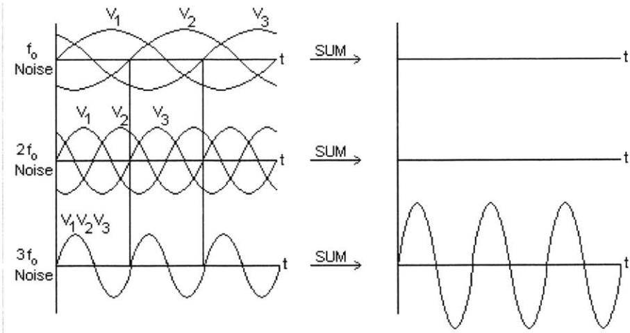
Figure 4.5 Effect of Correlated Noise Sources
