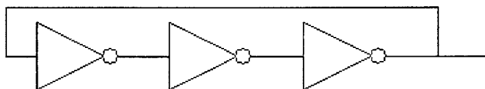
Figure 2.2 Basic Ring Oscillator
