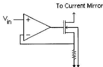
Figure 4.7 High Output Impedance V-to-I Converter
