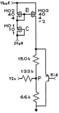
Figure 5.2 Mid-Buffer and Level-Shifter
