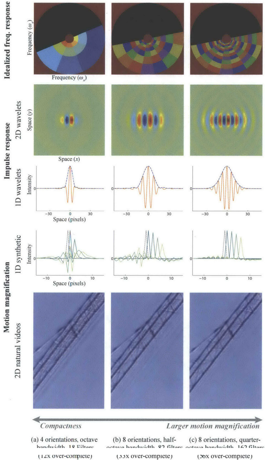
Figure 3.18: A comparison between octave and sub-octave bandwidth pyramids for motion magnification. Each color in the idealized frequency response represents a different filter. (a) The original steerable pyramid of Portilla and Simoncelli [37]. This pyramid has octave bandwidth filters and four orientations. The impulse response of the filters is narrow (rows 2–3), which reduces the maximum magnification possible (rows 4–5). (b-c) Pyramid representations with two and four filters per octave, respectively. These representations are more over-complete, but support larger magnification factors.
