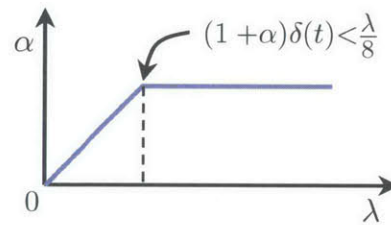
Figure 3.6: Amplification factor, \alpha , as function of spatial wavelength \lambda , for amplifying motion. The amplification factor is fixed to \alpha for spatial bands that are within our derived bound (Equation 3.14), and is attenuated linearly for higher spatial frequencies.
