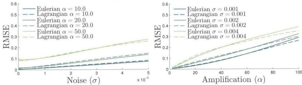
(c) Error as function of \sigma and \alpha , Spatiotemporal noise
