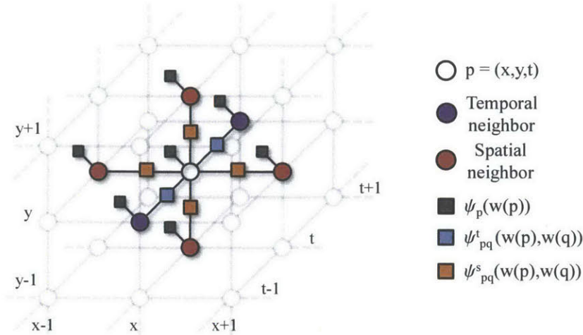
Figure 2.4: An illustration of the graphical model corresponding to Equation 2.5. Note that each node contains the three (unknown) components of the spatiotemporal displacement at that location.
