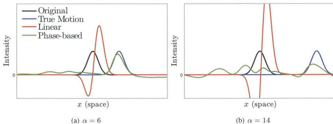
Figure 3.19: For general non-periodic structures, we achieve performance at least four times that of the linear technique, and do not suffer from clipping artifacts (a). For large amplification, the different frequency bands break up due to the higher bands having a smaller window (b).
