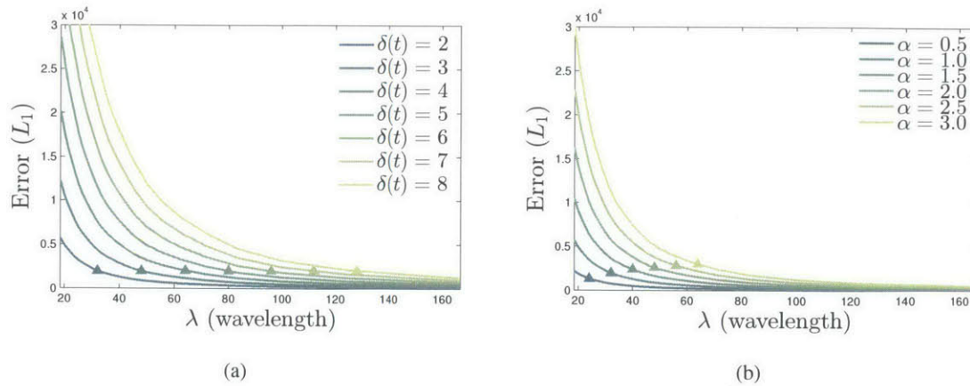
Figure 3.5: Motion magnification error, computed as the L_1 -norm between the true motion-amplified signal (Figure 3.4(a)) and the temporally-filtered result (Figure 3.4(b)), as function of wavelength, for different values of \delta(t) (a) and \alpha (b). In (a), we fix \alpha = 1 , and in (b), \delta(t) = 2 . The markers on each curve represent the derived cutoff point (1 + \alpha)\delta(t) = \frac{\lambda}{8} (Equation 3.14).
