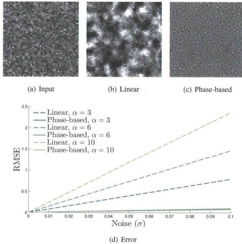
Figure 3.21: Comparison between linear and phase-based Eulerian motion magnification in handling noise. (a) A frame in a sequence of IID noise. In both (b) and (c), the motion is amplified by a factor of 50, where (b) uses the linear technique (Section 3.2) and (c) uses the phase-based approach. (d) shows a plot of the error as function of noise for each method, using several magnification factors.
