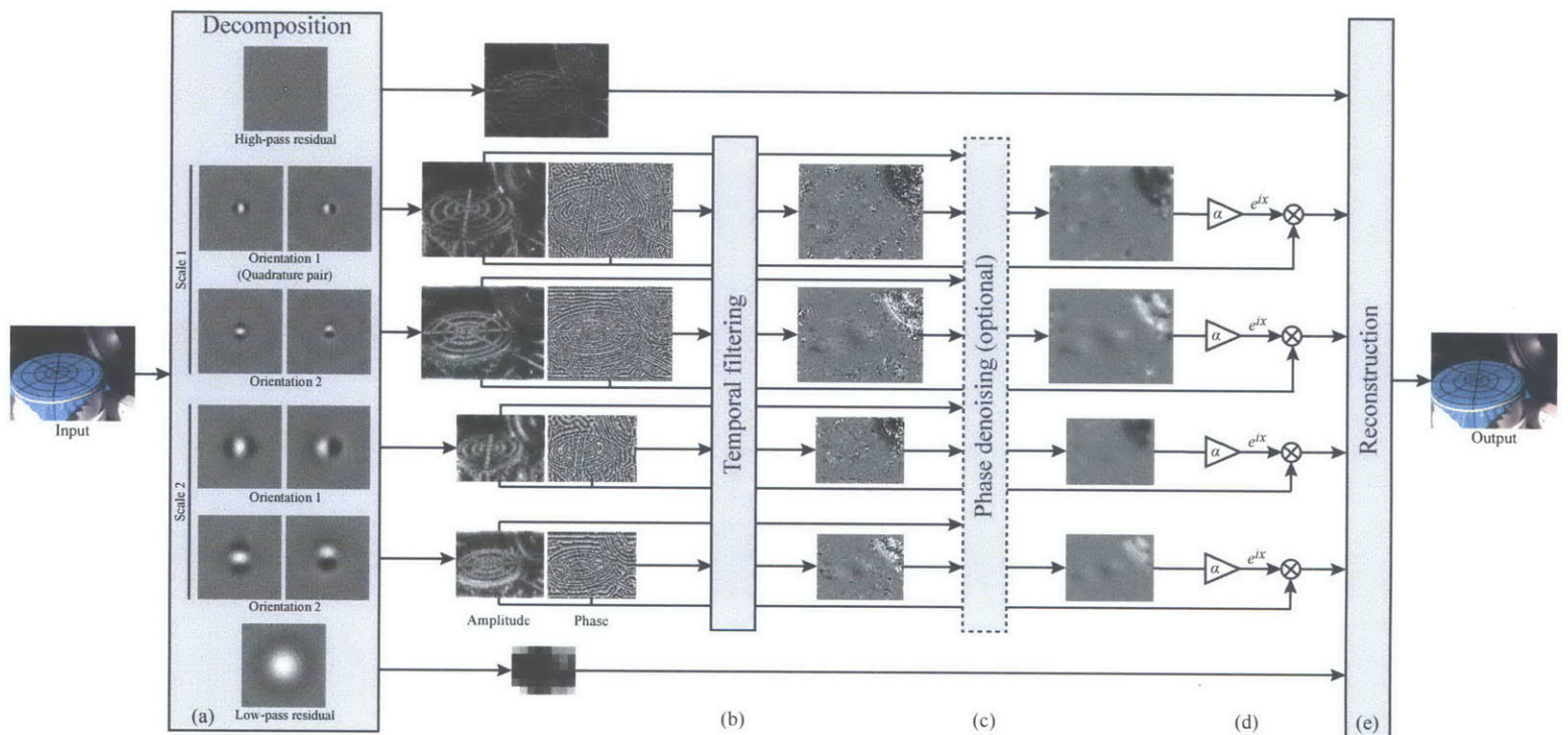
Figure 3.16: Our phase-based approach manipulates motion in videos by analyzing the signals of local phase over time in different spatial scales and orientations. We use complex steerable pyramids to decompose the video and separate the amplitude of the local wavelets from their phase (a). We then temporally filter the phases independently at each location, orientation and scale (b). Optionally, we apply amplitude-weighted spatial smoothing (c, Sect. 3.3.6) to increase the phase SNR, which we empirically found to improve the results. We then amplify or attenuate the temporally-bandpassed phases (d), and reconstruct the video (e). This example shows the processing pipeline for the membrane sequence (Sect. 3.3.7), using a pyramid of two scales and two orientations (the relative difference in size between the pyramid levels is smaller in this figure for clarity of the visualization).
