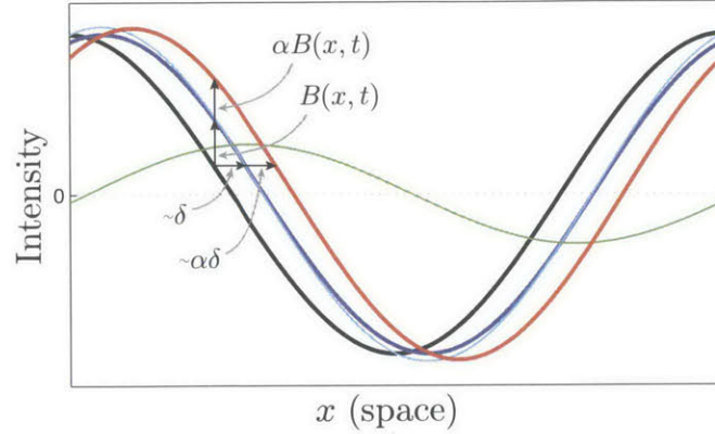
Figure 3.3: Temporal filtering can approximate spatial translation. This effect is demonstrated here on a 1D signal, but equally applies to 2D. The input signal is shown at two time instants: I(x, t) = f(x) at time t and I(x, t + 1) = f(x + \delta) at time t + 1 . The first-order Taylor series expansion of I(x, t + 1) about x approximates well the translated signal. The temporal bandpass is amplified and added to the original signal to generate a larger translation. In this example \alpha = 1 , magnifying the motion by 100%, and the temporal filter is a finite difference filter, subtracting the two curves.
