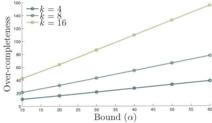
Figure 3.22: Over-completeness as function of the bound on the amplification factor, \alpha , in our pyramid representation with different number of orientations, k , 1 – 6 filters per octave (points left to right), and assumed motion \delta(t) = 0.1 pixels. For example, a half-octave, 8-orientation pyramid is 32x over-complete, and can amplify motions up to a factor of 20, while a similar quarter-octave pyramid can amplify motions by a factor of 30, and is 43x over-complete.
