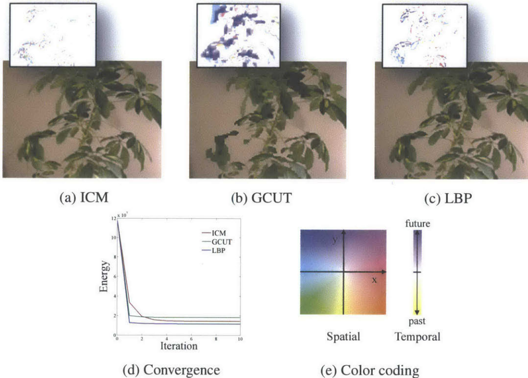
Figure 2.5: Comparison between different optimization techniques for solving Equation 2.5, demonstrated on the plant time-lapse sequence (Figure 2.7). (a-c) Representative frames from each result. The spatial components of the displacement fields (overlaid) illustrate that different local minima are attained by the different optimization methods (the full sequences are available in the accompanying material). (d) The energy convergence pattern over 10 iterations of the algorithms. (e) The color coding used for visualizing the displacement fields, borrowed from [3].
