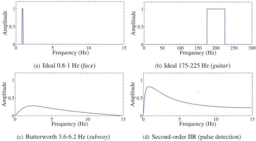
Figure 3.10: Temporal filters used in the thesis. The ideal filters (a) and (b) are implemented using DCT. The Butterworth filter (c) is used to convert a user-specified frequency band to a second-order IIR structure that can be used for real-time processing (Section 3.4). The second-order IIR filter (d) also allows user input. These second-order filters have a broader passband than an ideal filter.
