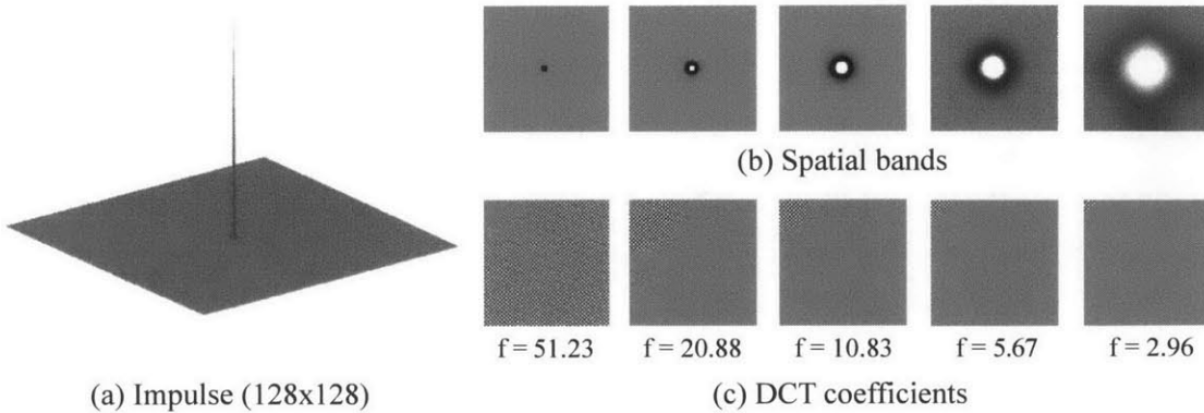
Figure 3.7: Spatial frequencies of the Laplacian pyramid. To estimate the spatial frequencies at each pyramid level, we decompose an impulse image (a) to its spatial frequency bands (b), and compute the DCT coefficients for each band (c). We estimate the spatial frequency for each band (given below the DCT coefficients in (c)) as the average magnitude of its corresponding DCT coefficients, weighted by their distance from the origin (upper left corner in (c)).
