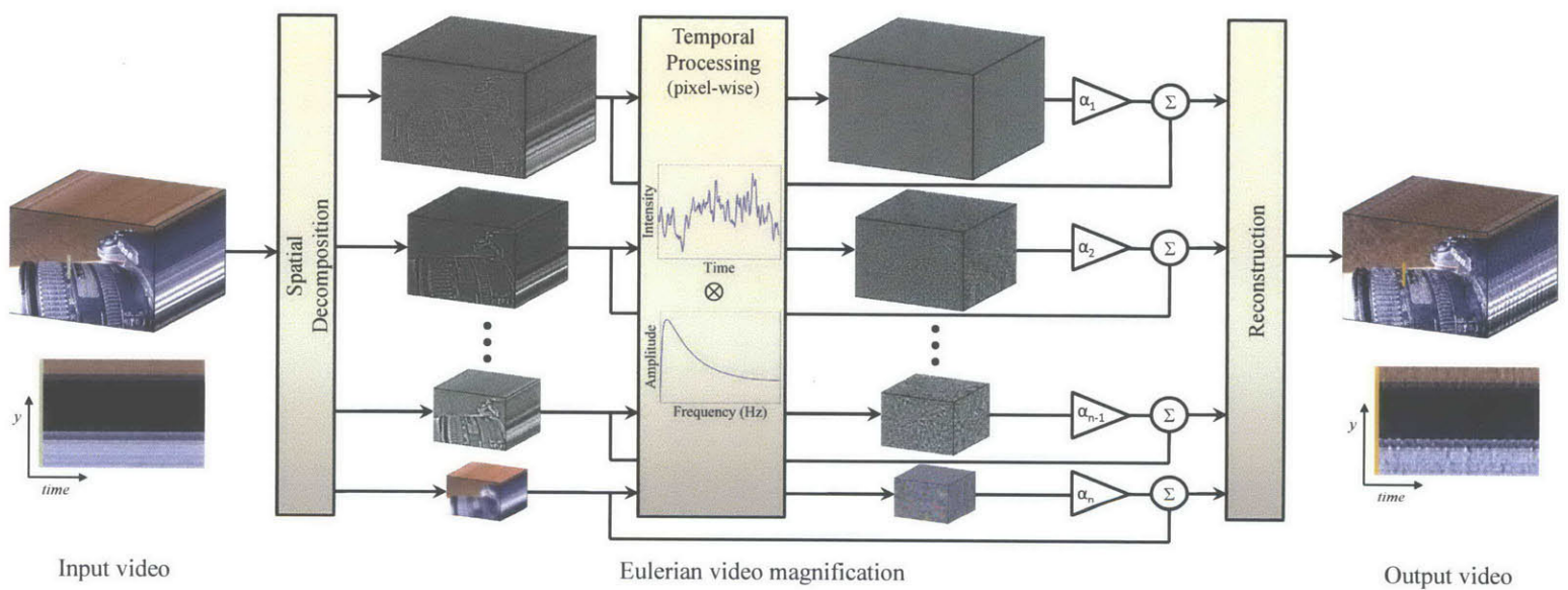
Figure 3.2: Overview of the Eulerian video magnification framework. The system first decomposes the input video sequence into different spatial frequency bands, and applies the same temporal filter to all bands. The filtered spatial bands are then amplified by a given factor \alpha , added back to the original signal, and collapsed to generate the output video. The choice of temporal filter and amplification factors can be tuned to support different applications. For example, we use the system to reveal unseen motions of a Digital SLR camera, caused by the flipping mirror during a photo burst ( camera ; full sequences are available in the supplemental video).
