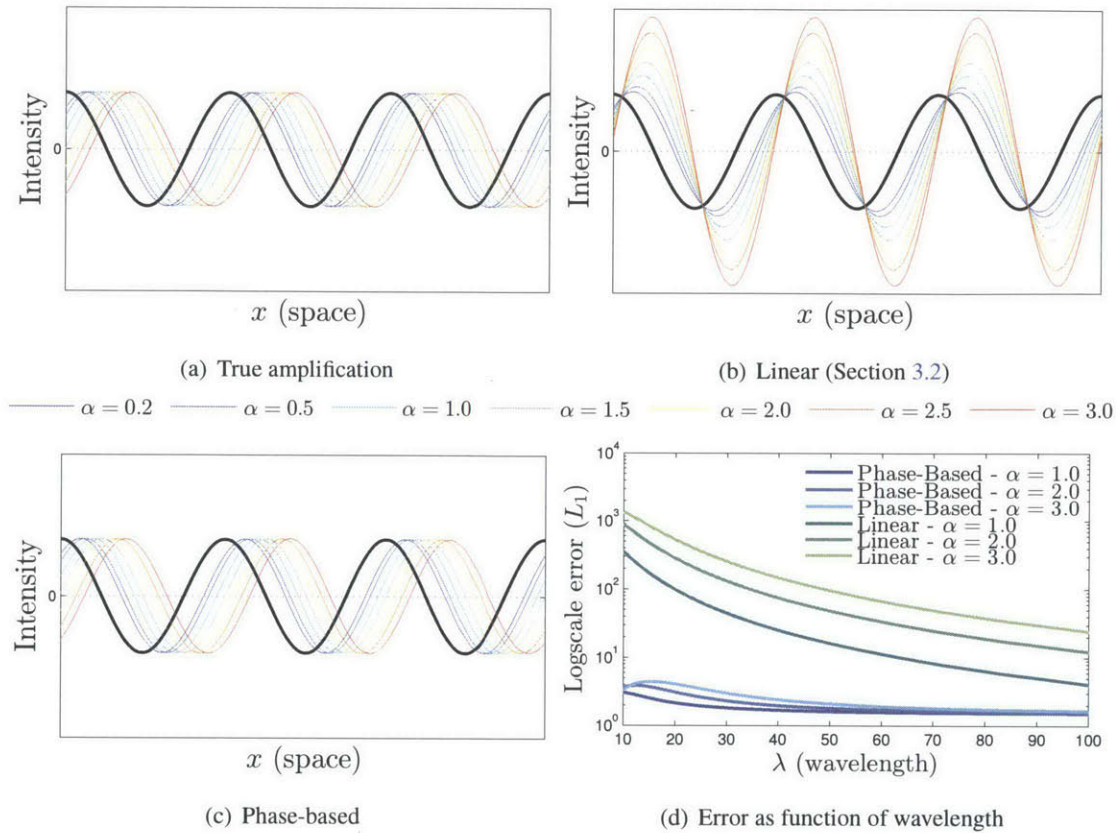
Figure 3.17: Phase-based motion magnification is perfect for sinusoidal functions. In these plots, the initial displacement is \delta(t) = 1 . While the errors for the linear technique (Section 3.2) are dependent on wavelength for sinusoids, there is no such dependence for the present technique and the error is uniformly small. The vertical axis in (d) is logarithmic.
