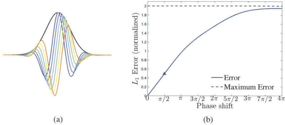
Figure 3.20: The impulse response of the steerable filter bank illustrates the artifacts that arise when modulating phase to magnify motion. (a) The impulse response of a wavelet being phase shifted. As the phase increases (orange corresponds to \frac{3\pi}{4} ), the primary peak shifts to the right decreasing under the Gaussian window. A secondary peak forms to the left of the primary peak. (c) Error in magnification of the impulse response as the impulse is moved under the Gaussian window. The maximum (normalized) error occurs when the phase-shifted wavelet no longer overlaps with the true-shifted one. The constant C = \sigma is marked on the curve.
