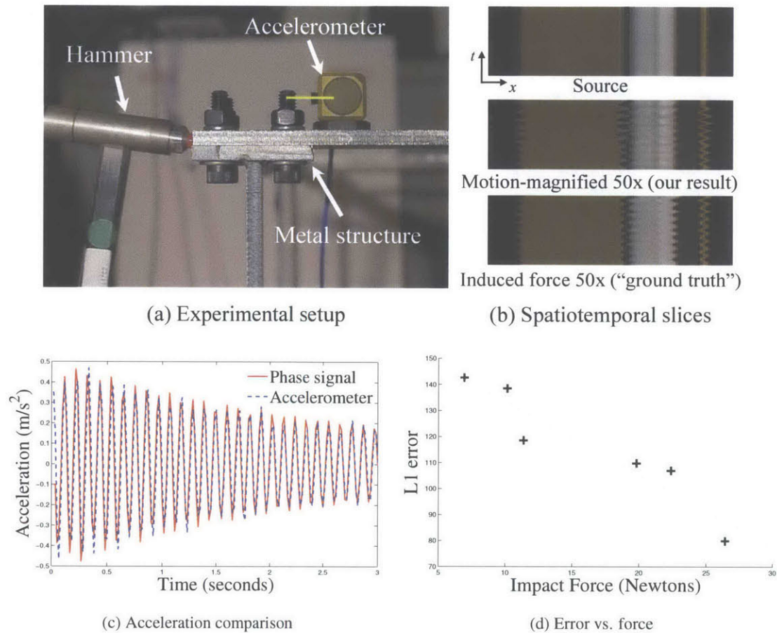
Figure 3.24: A controlled motion magnification experiment to verify our framework. (a) A hammer strikes a metal structures which then moves with a damped oscillatory motion. (b) A sequence with oscillatory motion of amplitude 0.1 pixels is magnified 50 times using our algorithm and compared to a sequence with oscillatory motion of amplitude 5 pixels (50 times the amplitude). (c) A comparison of acceleration extracted from the video with the accelerometer recording. (d) The error in the motion signal we extract from the video, measured as in (c), as function of the impact force. Our motion signal is more accurate as the motions in the scene get larger. All videos are available in the supplementary material.
