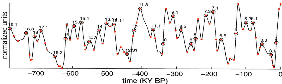
Figure 3-19: The SPECMAP \delta^{18}O stack [ Imbrie et al. , 1984] with each of its ACPs labeled as red dots. The thirty ACPs used to construct the high-resolution EOF1 are indicated by black circles and are numbered according the decimal notation used for the SPECMAP stack. Time goes from left to right and the units are normalized.
