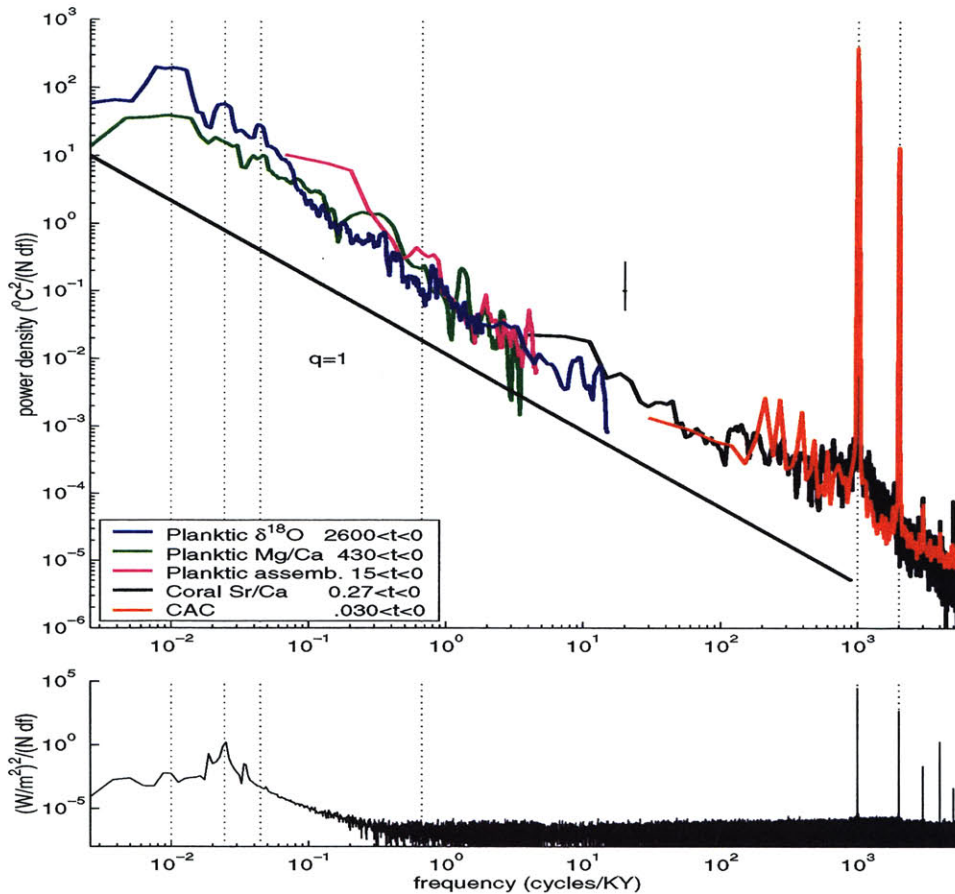
Figure 1-1: top: Power-density spectra of tropical sea surface temperature variability. Temperature variability is estimated using, from lowest to highest frequency, marine planktic \delta^{18}O (blue), planktic Mg/Ca measurements (green), planktic assemblages (magenta), coral Sr/Ca (black), and instrumental tropical pacific sea surface temperatures from the Climate Analysis Center (red). The length of each record is indicated in the legend in KY BP; references are provided in Appendix A. A least squares estimate of the spectral slope between 1/100 and 1000 cycles/KY gives a power law relationship with q \approx 1 . At frequencies above the annual cycle, the power-law steepens to about 2 (not shown). The annual and semi-annual estimates are adjusted to have the power-density expected for a record 800 KY long — the duration of the planktic \delta^{18}O records. bottom Periodogram of diurnally averaged insolation at 65^\circ N over the last 1000 KY BP and sampled monthly. Vertical dashed lines indicate bands centered on 1/100, 1/41, 1/23, 1/1.5, 1000, and 2000 cycles per KY. The power-density units are in degrees Celsius squared divided by the number of samples, N , and the spectral band-width, df . The vertical bar indicates the approximate 95% confidence level. Estimates are made using the multi-taper method with three windows. This insolation spectra is discussed more fully in Chapter 2, specifically with regard to the weak 1/100KY and absence of energy at the 1/23KY precession band.
