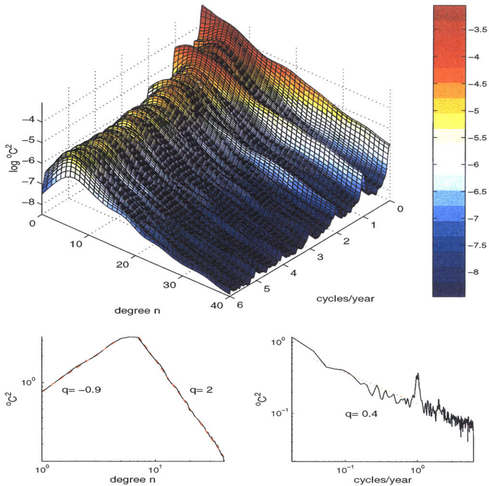
Figure 1-5: Similar to Figure 1-4 but for NCEP temperature variations with the monthly averages removed. Most notable is the peak of energy at degree n = 6 and 7 , with energy diminishing at an exponential rate towards the larger and smaller scales.
