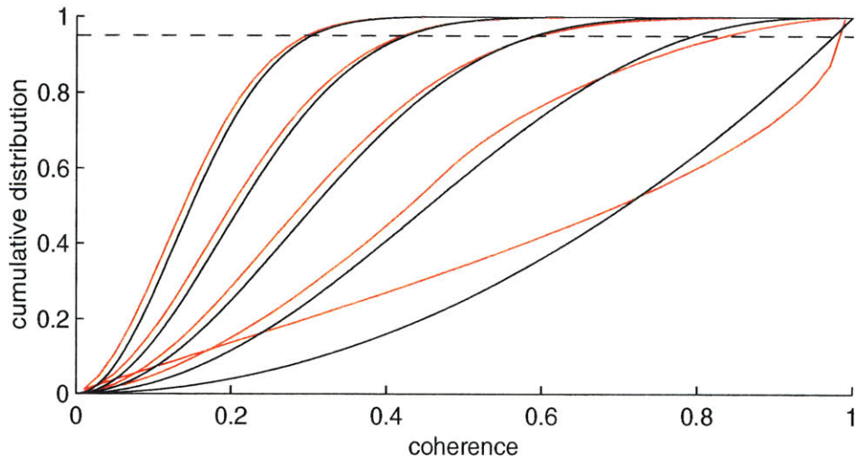
Figure 4-8: The cumulative density function (CDF) for linear coherence (black) from the analytical results of Amos and Koopman [1963] and nonlinear coherence (red) estimated using a Monte Carlo method as described in the text. From left to right the pairs of linear and nonlinear CDFs are for 32, 16, 8, 4, and 2 degrees of freedom. Results assume the phase is uniformly distributed. The nonlinear coherence CDFs tend to be shifted toward lower values, but for greater degrees of freedom this difference becomes small. The vertical dashed line indicates the 95% confidence level above which the null-hypothesis of a uniform phase distribution can be rejected.
