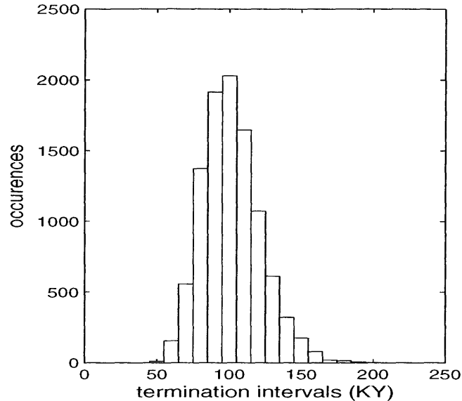
Figure 4-6: A histogram of the time between consecutive terminations derived from the random walk ice-volume model (Eq. 4.4). The selected parameterizations are a noise amplitude a=2 , a drift b=1 , and an ice-volume threshold \xi=100 . The mean interval between terminations is 100KY with a \pm 20KY standard deviation. The distribution is close to Gaussian but with a slightly elongated tail towards longer intervals.
