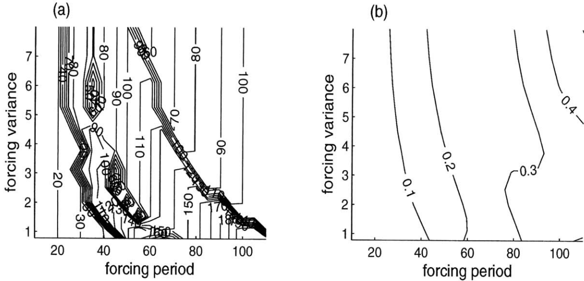
Figure 5-9: Model response to periodic forcing. a The period associated with the most energetic model response is contoured against the forcing variance and forcing period. b The variance of the model response contoured against the forcing variance and period. All model runs have 1KY time-steps for 5000KY.
