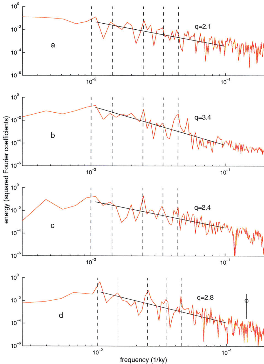
Figure 5-11: Periodograms of model results using the \mathcal{F}_{op} parameterizations: a Imbrie model, b Paillard model, and c new model. d is the periodogram of EOF1. Power-laws are indicated by the solid lines fit to the spectra between 1/10 and 1/100KY where the slope is given by q . Vertical dashed lines are centered on the bands in which EOF1 has significant concentrations of energy: 1/100, 1/70, 1/41, 1/29, and 1/23KY. The vertical solid line in d indicates the approximate 95% confidence interval. The Imbrie model and the new model have spectral peaks at each of the vertical lines.
