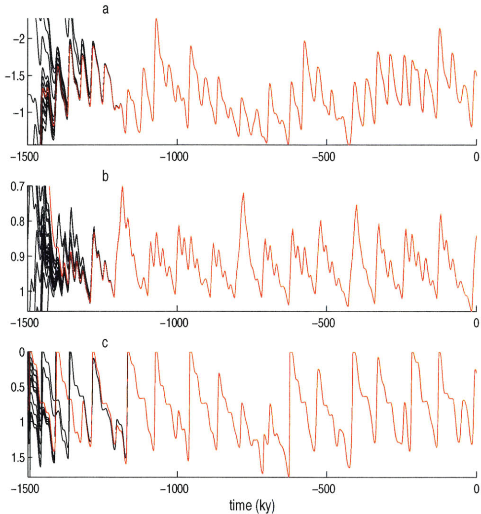
Figure 5-6: Sample trajectories of each model using randomized initial conditions: a the Imbrie model, b Paillard mode, and c the new model. Each of the models converge onto a single trajectory. The last realization from each model is plotted in red.
