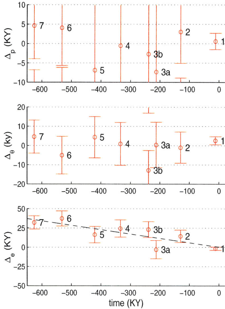
Figure 4-3: Similar to Table 4.1, the timing of terminations relative to local maxima in precession (top, \Delta^p ), obliquity (middle, \Delta^\theta ), and eccentricity (bottom, \Delta^e ) in KY. Positive values indicate the maximum in the orbital parameter lags the termination. Termination numbers are listed for each estimate along with vertical bars indicating the one standard deviation age-model uncertainty. Note that the scaling of the y-axis is plus and minus roughly half the period of each orbital parameter and that uncertainty bars wrap around. A least-squares fit of the trend in \Delta^e is indicated by the dashed line; it has a slope of -6\text{KY}/100\text{KY} .
