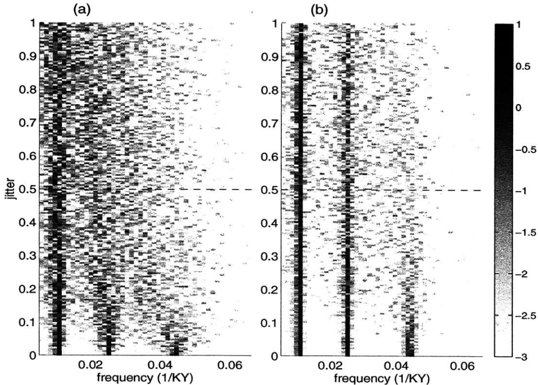
Figure 3-6: The impact of age-model jitter on the power spectrum of a harmonic processes, \mathcal{H} (Eq. 3.17). Shading indicates the logarithm of the power estimate plotted against frequency (1/KY) and the degree of jitter where s_o = 1/40\text{KY} (see Eq. 3.11). Both plots show spectra of \mathcal{H} after distorting its timescale according to the specified jitter: (a) has errors as expected for a single age-depth relationship, while (b) has errors as expected for the depth-derived age-model. The degree of jitter expected in a real core is 0.5, and is indicated by the horizontal dashed line. In (a) only the 100KY band can be distinguished, while (b) retains good resolution of the 100KY and 41KY bands and a semblance of the 23KY band.
