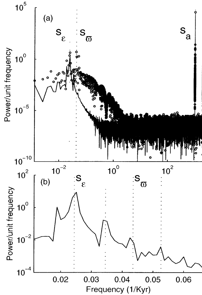
Figure 2-9: Periodograms of mean diurnal insolation plus a small amount of white noise. (a), Solid line is from insolation at 65^{\circ}\text{N} , while circles are from insolation passed through a \nu th-law device with \tau = 250 \text{ Watts/m}^2 and \nu = 1 . After rectification, low frequency energy at the obliquity band ( s_{\epsilon} ) is enhanced, and energy at the precession band ( s_{\omega} ) now appears. The ordinate and abscissa are logarithmic. For plotting purposes, an exponentially diminishing number of periodogram estimates are shown for frequencies above 1/10 \text{ kyr} except near the annual cycle and its first harmonic where full resolution is used—no significant structural changes result. (b), Periodogram of insolation at 85^{\circ}\text{N} . Vertical lines from left to right are centered on the obliquity bands at 1/41 and a minor side-band at 1/29 \text{ kyr} [Melice et al. , 2001] and precession at 1/23 and 1/19 \text{ kyr} . The abscissa is linear, and for visual clarity, only the low-frequencies are shown. The seasonal cycle, s_a , is so much more powerful than any other insolation frequency (other than the diurnal) that its rectification is of greatest concern, but all frequencies are susceptible to such effects.
