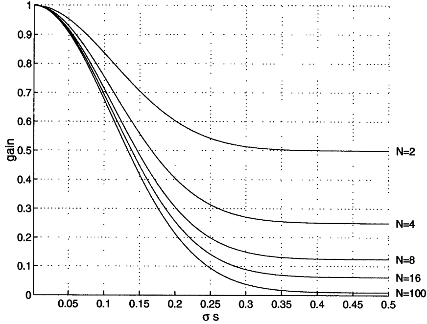
Figure 3-18: The expected gain, Eq 3.39, plotted against frequency, s , times the standard deviation of the relative age-model jitter, \sigma . Plots are for averaging N = 2, 4, 8, and 16 records. The gain scales equivalently with both \sigma and s ( \sigma s \sim \sqrt{-\ln g} ) so that it is more general to plot the gain against \sigma s . For small \sigma s the gain approaches one, while for large \sigma s the gain asymptotes to 1/N — the expected behavior for perfect synchronization and complete phase randomization respectively.
