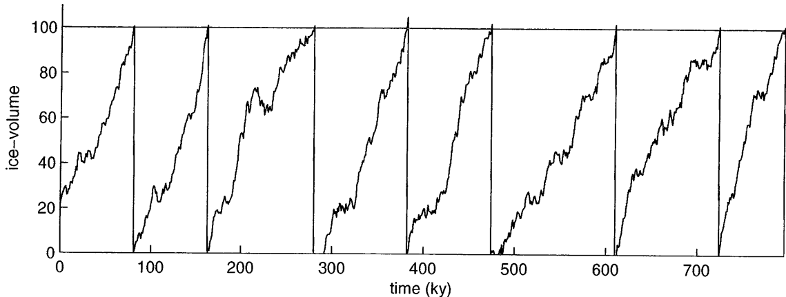
Figure 4-4: A realization of the random walk model of ice-volume (Eq. 4.4). The selected parameterizations are a noise amplitude of a=2 , a drift of b=1 , and an ice-volume threshold of \xi=100 . Terminations are triggered once the threshold (indicated by the horizontal red line) is crossed. All units are normalized.
