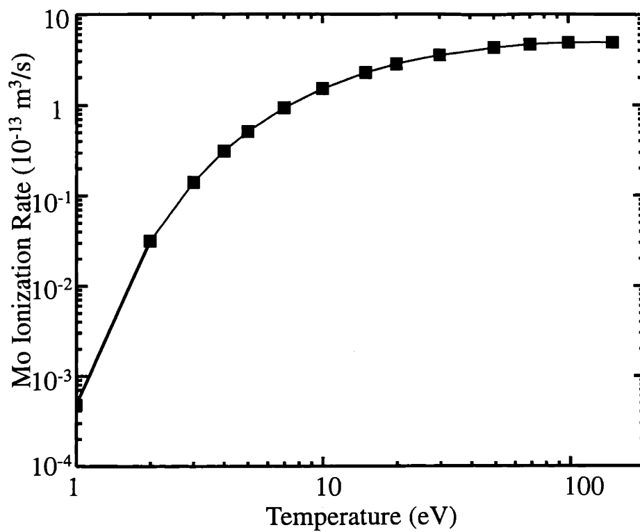
Fig. 5-4: Neutral molybdenum ionization rate as a function of temperature [64].
