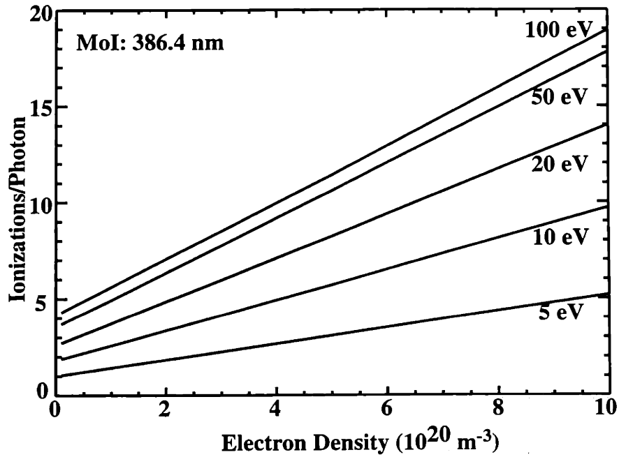
Fig. 2-16: Molybdenum ionizations per 386.4 nm emitted photon ( S/XB ) as a function of the electron density for a number of electron temperatures. Calculated using the data of Table 2-3 that have been multiplied by 3.
