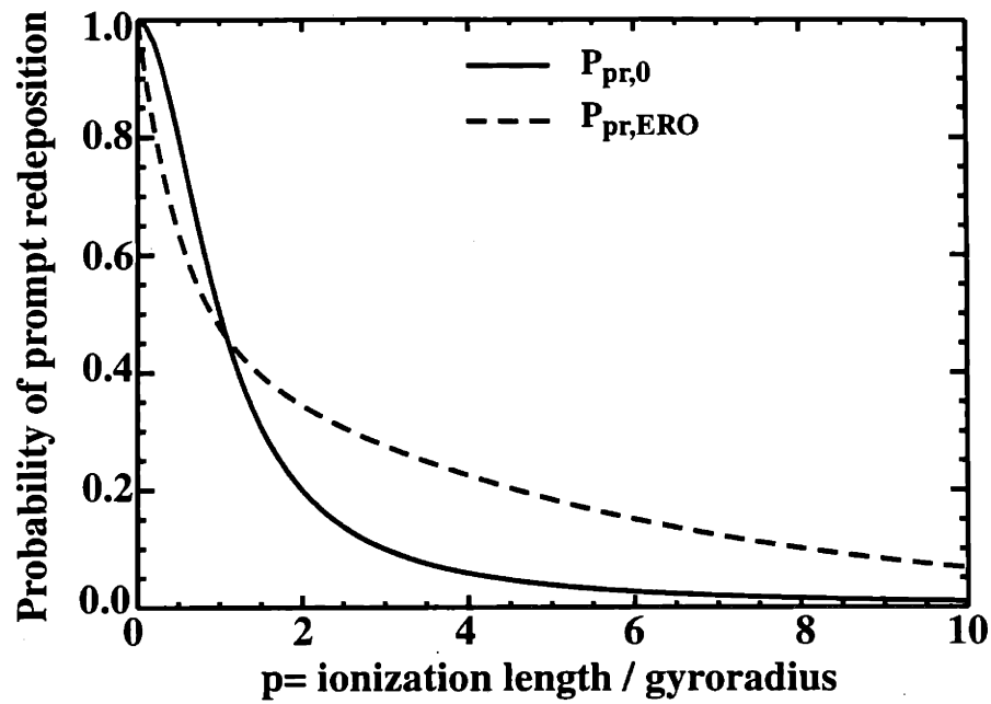
Fig. 5-6: Comparison of the probability of prompt redeposition calculated with the simplified model (Eq. 5.19) to the one obtained with the model utilizing the ERO code (Eq. 5.20).
