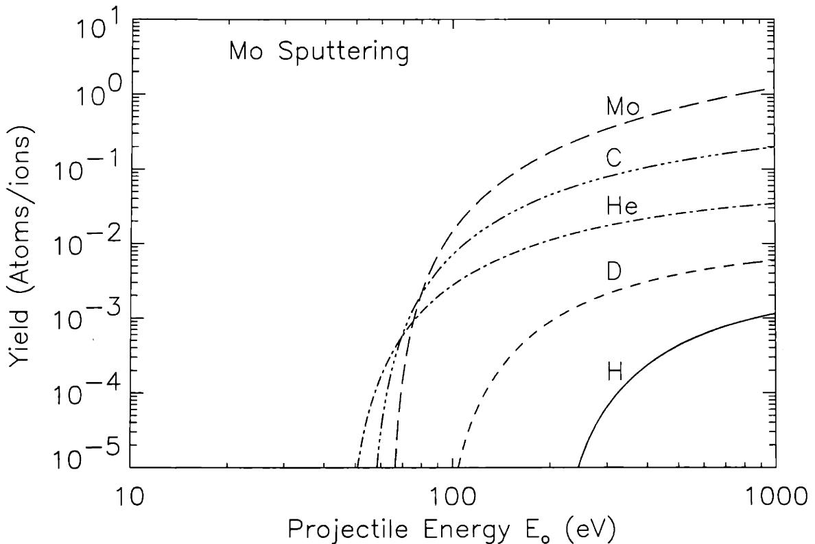
Fig. 5-1: Molybdenum sputtering yields versus projectile energy for bombardment with H, D, He, C, and Mo at normal incidence, using the revised Bohdansky formula. The parameters Q , E_{TF} , and E_{th} are obtained from Ref. [48].
