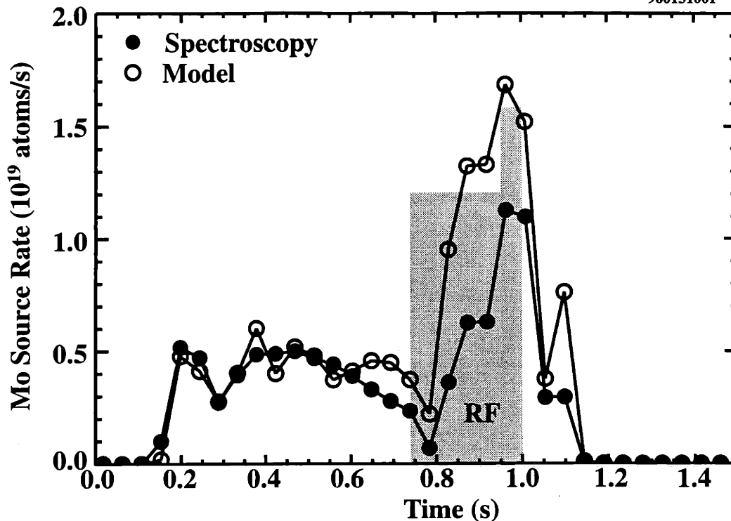
Fig. 5-13: Comparison of the calculated outer divertor source rate from spectroscopic data and the sputtering model. The RF power, which is also sketched, is increased from 1.2 to 1.6 MW at 0.95 s.
