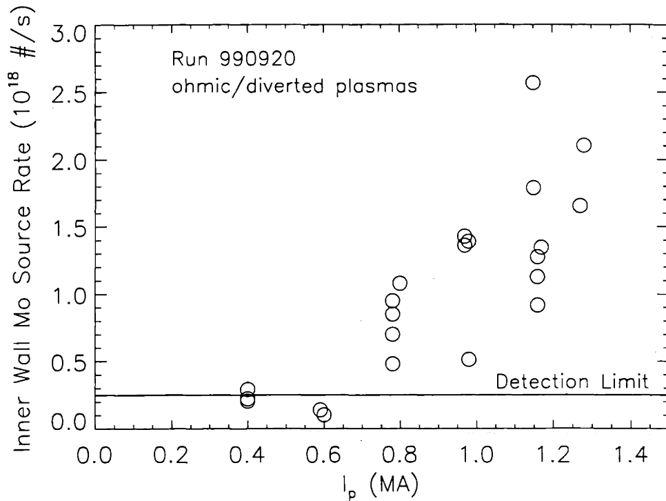
Fig 3-4: Effect of the plasma current on the inner wall molybdenum source rate during the ohmic phase of diverted plasmas.
