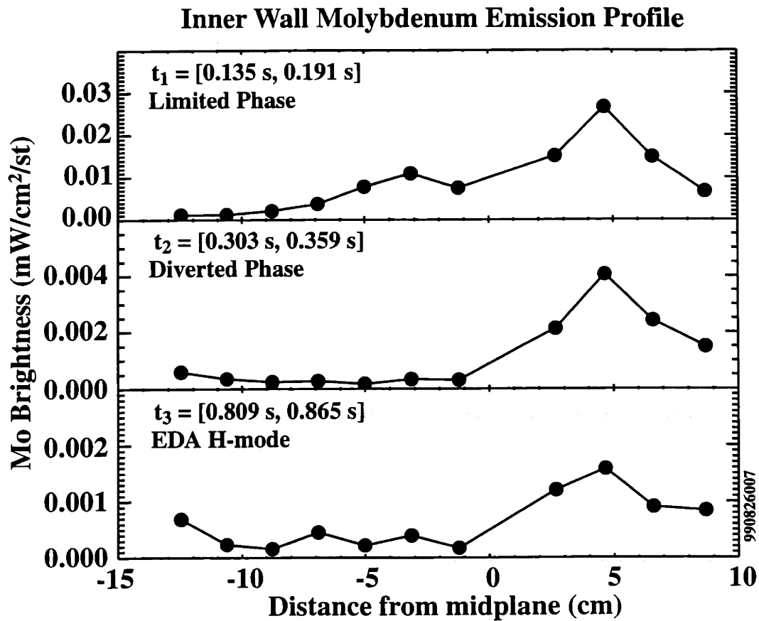
Fig. 3-15: Inner wall molybdenum emission profiles for three different plasma phases: limited, diverted ohmic, and EDA H-mode. The molybdenum brightness is plotted versus the distance from the Alcator C-Mod midplane. Signals levels smaller than \sim 0.001 \text{ mW/cm}^2/\text{st} are below the spectrometer's detection limit.
