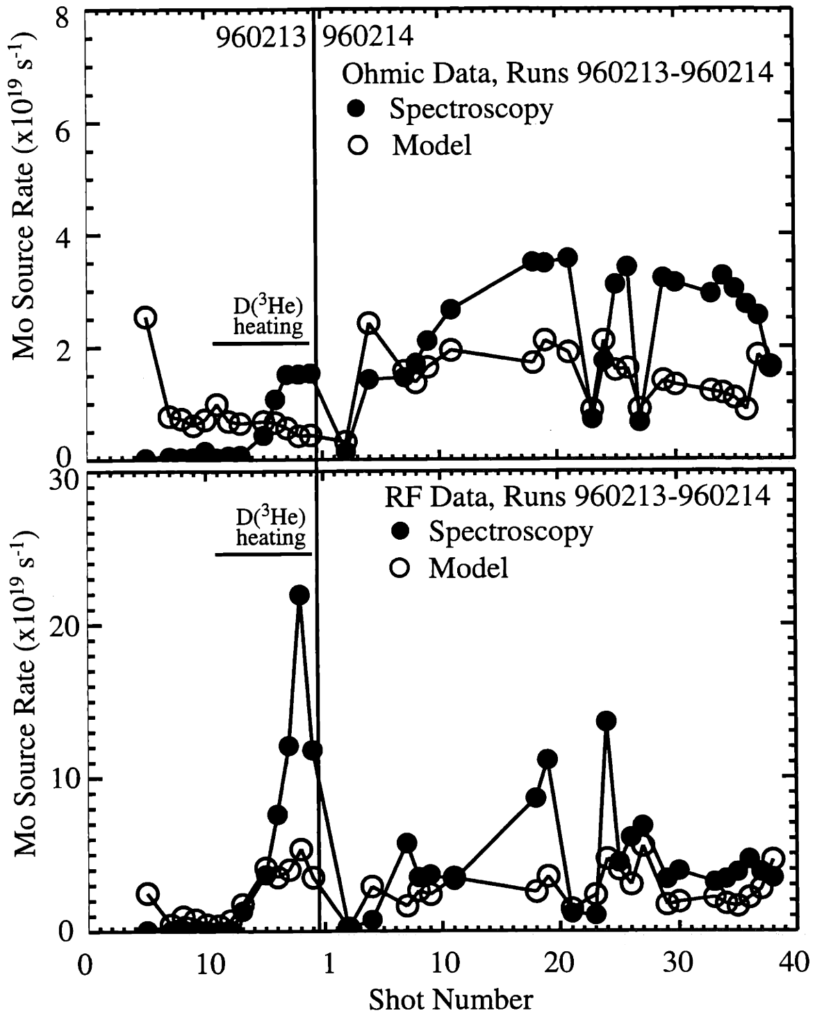
Fig. 5-18: Molybdenum source rates from spectroscopy and model for a number of shots from the 960213 and 960214 runs. Top panel: averages during the ohmic phase of each shot. Bottom panel: averages during the RF phase. The solid line defines the end of the 960213 run and the beginning of the 960214 run. The numbers for the shots are actual shot numbers.
