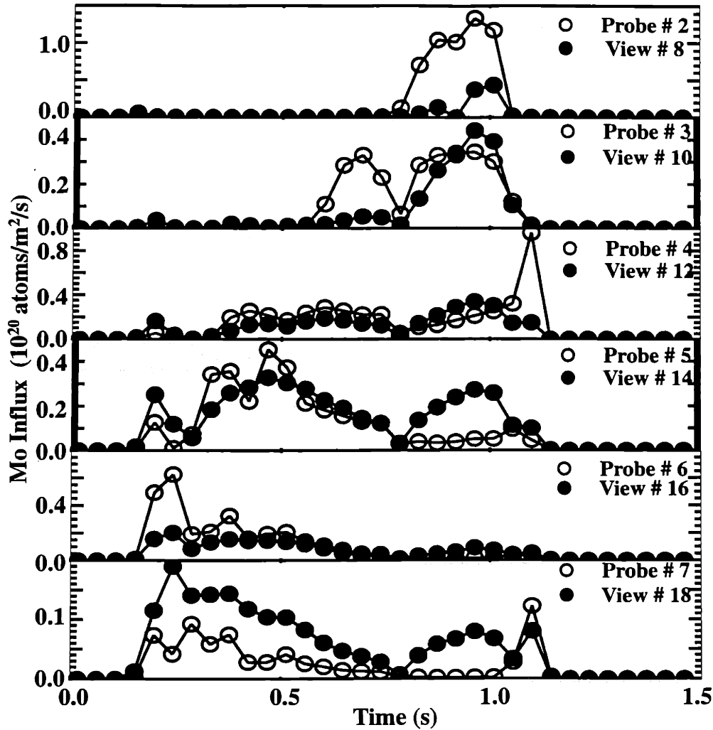
Fig. 5-14: Comparison of the spectroscopically measured molybdenum influx, for the six outer divertor chords used, to that calculated from the sputtering model for the corresponding probes.
