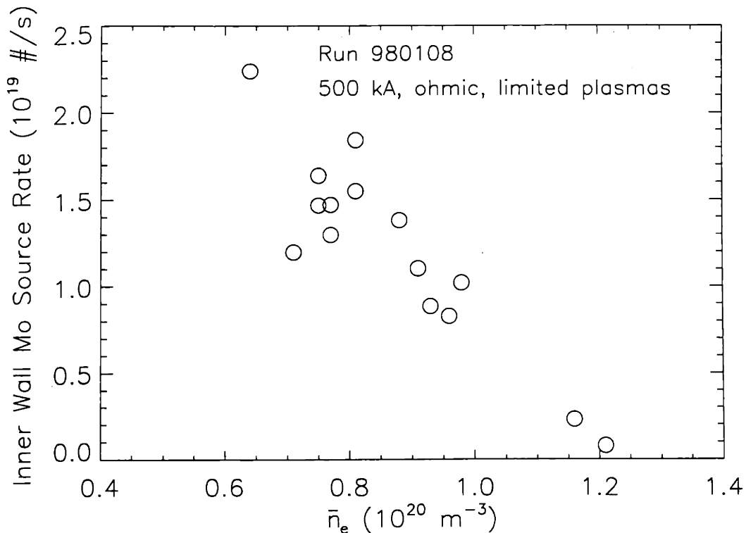
Fig. 3-5: Effect of electron density on the inner wall molybdenum source rate during the ohmic phase of inner-wall limited plasma discharges. A representative shot is shown in Fig. 3-3.
