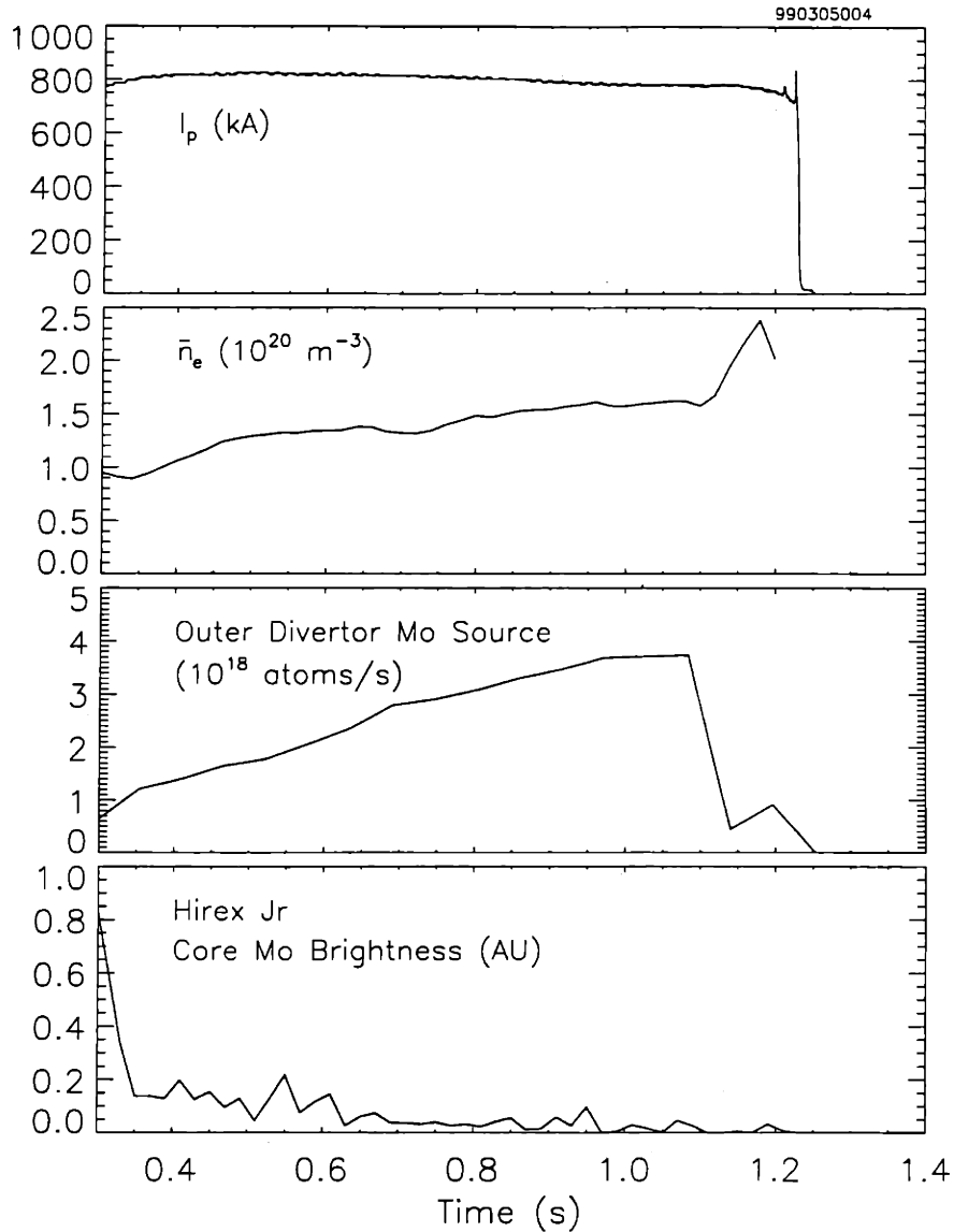
Fig. 3-18: Time history of the outer divertor molybdenum source rate for an ohmic discharge. The plasma current, volume averaged electron density, and core molybdenum brightness traces are also shown. The molybdenum brightness units are the same as the ones used in Fig. 3-2.
