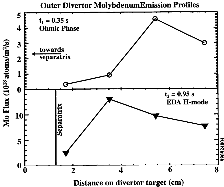
Fig. 3-29: Outer divertor molybdenum influx as a function of the location on the divertor target for ohmic and EDA H-mode conditions. The data were taken with views 10, 12, 14, and 16.
