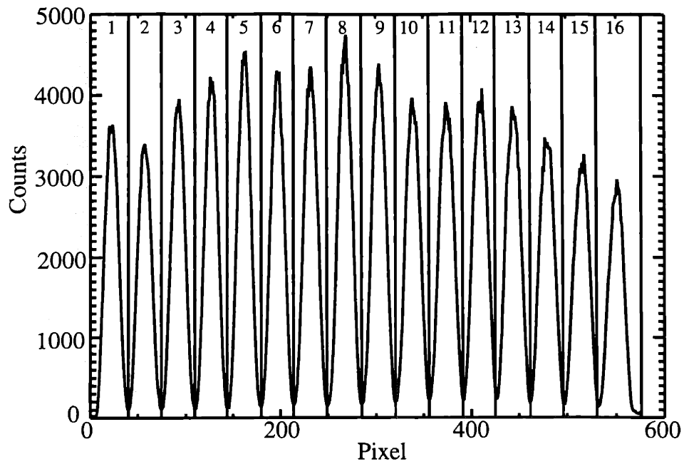
Fig. 2-2: Binning of the 576 CCD pixels in the spectrometer's spatially resolving dimension. The solid line between bins represents the 4 pixels wide zone that is not processed.
