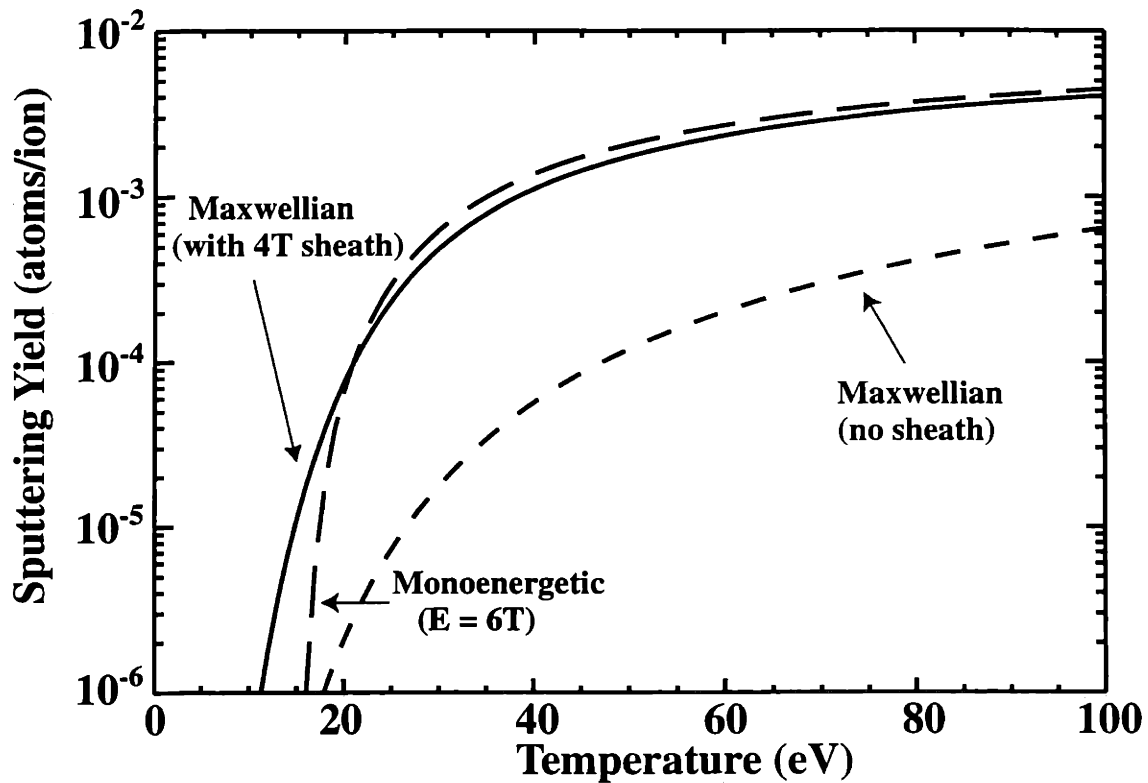
Fig. 5-9: Sputtering yield versus temperature for normal incidence of deuterium ions on molybdenum. Three curves are shown: for Maxwellian distribution of particles with and without sheath acceleration and for monoenergetic bombardment that includes sheath acceleration.
