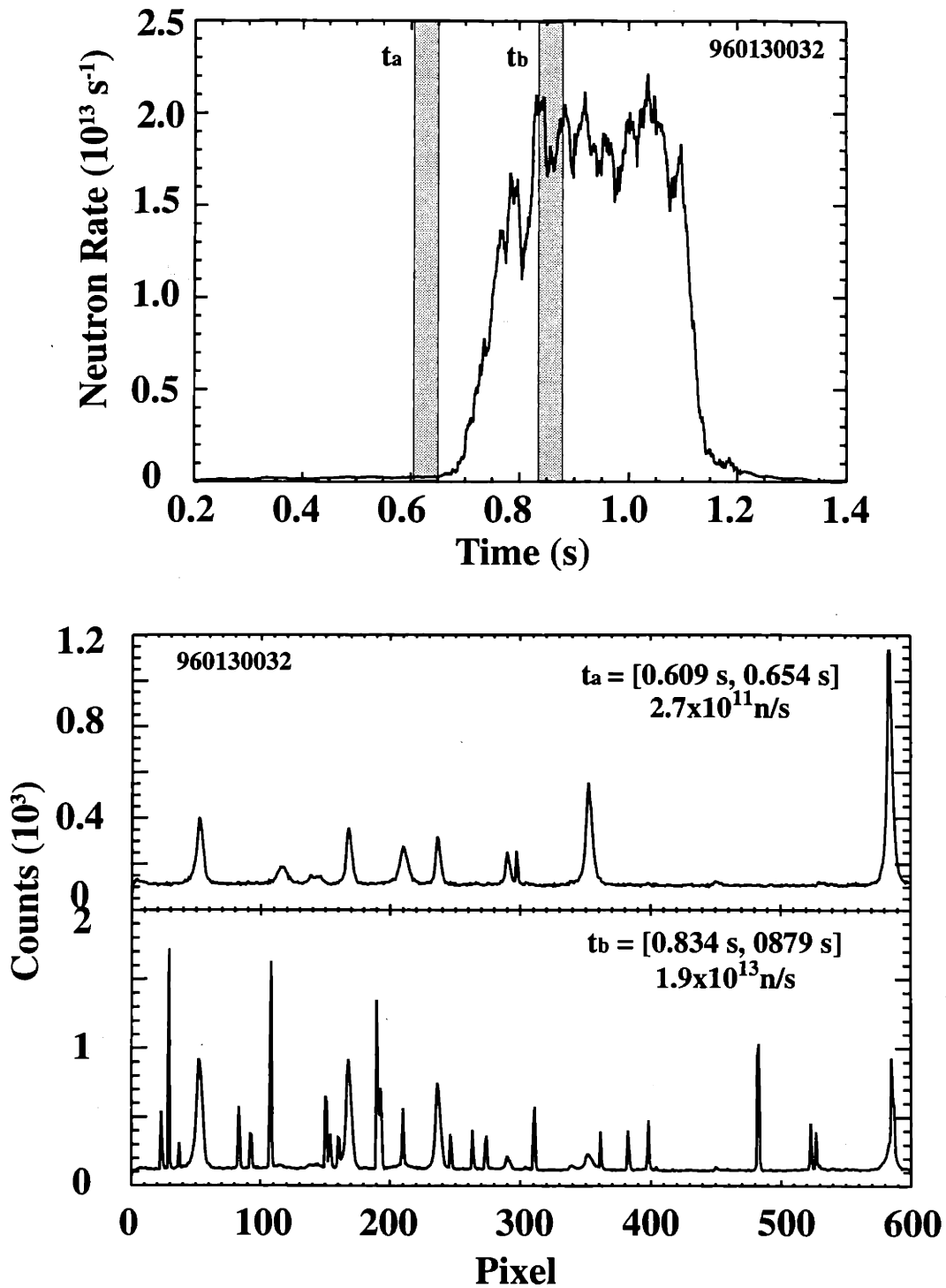
Fig. 2-11: Fusion neutron rate for plasma discharge 960130032 (top panel). Typical spectra, of the same spectral region, taken with the Chromex spectrometer (bottom panel) during the time slices indicated in the neutron rate time history. There is only one spike (around pixel 300) when the neutron rate is low but a significant number of them appear during the high neutron rate period.
