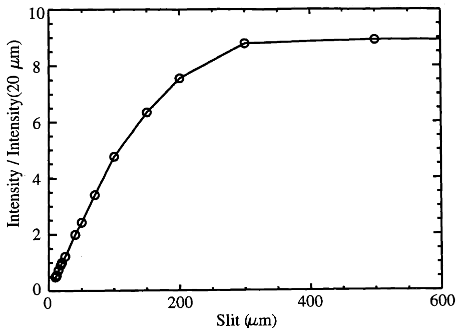
Fig. 2-7: Effect of entrance slit on signal intensity. The signal is normalized to the intensity for the 20 \mu\text{m} slit. The data were obtained with the 1200\text{ mm}^{-1} grating at 405 nm for bin 8 and pixel 621.
