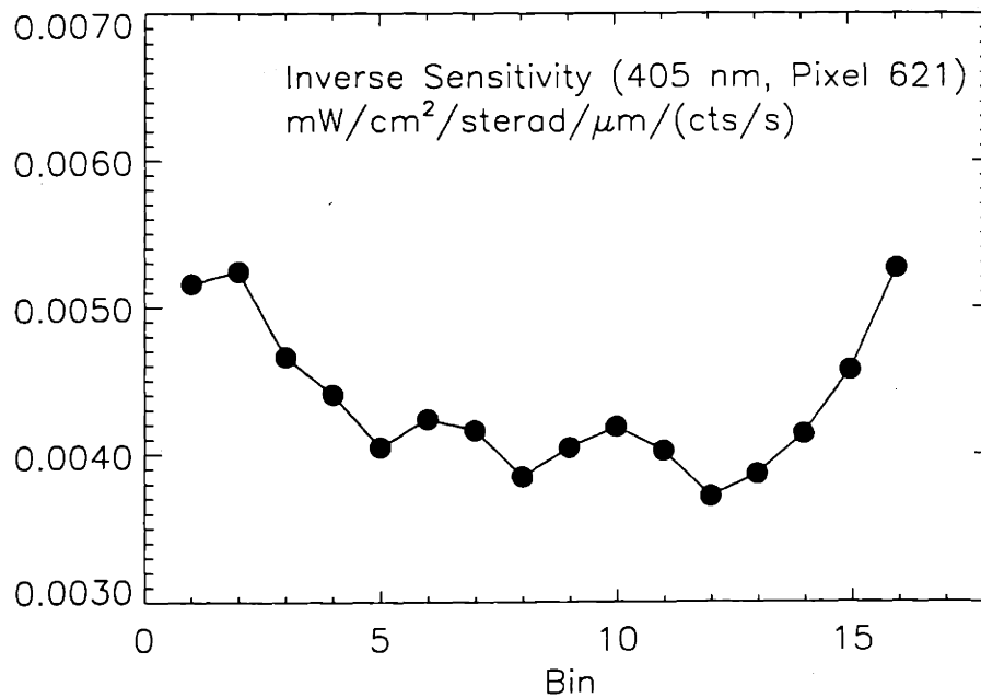
Fig. 2-6: Inverse sensitivity as a function of bin at 405 nm, with a 20 μm entrance slit, and the 1200 mm -1 grating.
