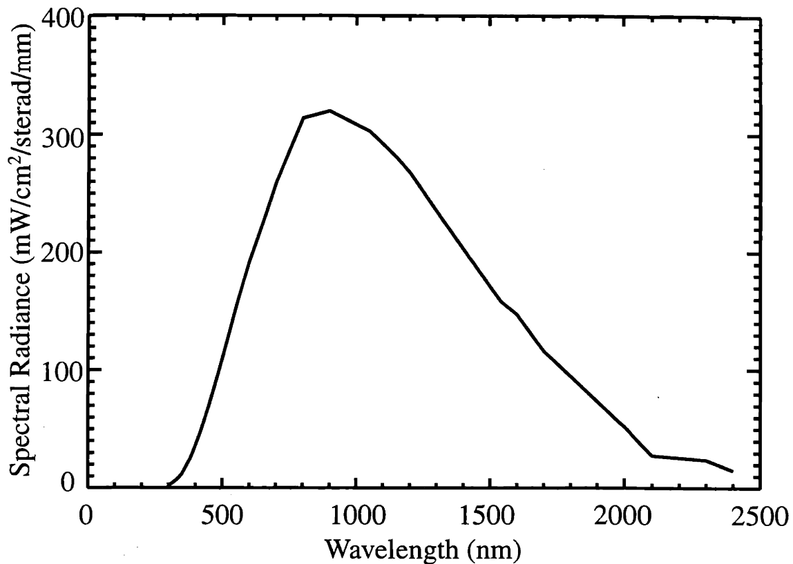
Fig. 2-4: Spectral radiance of the lamp used for the absolute intensity calibrations.
