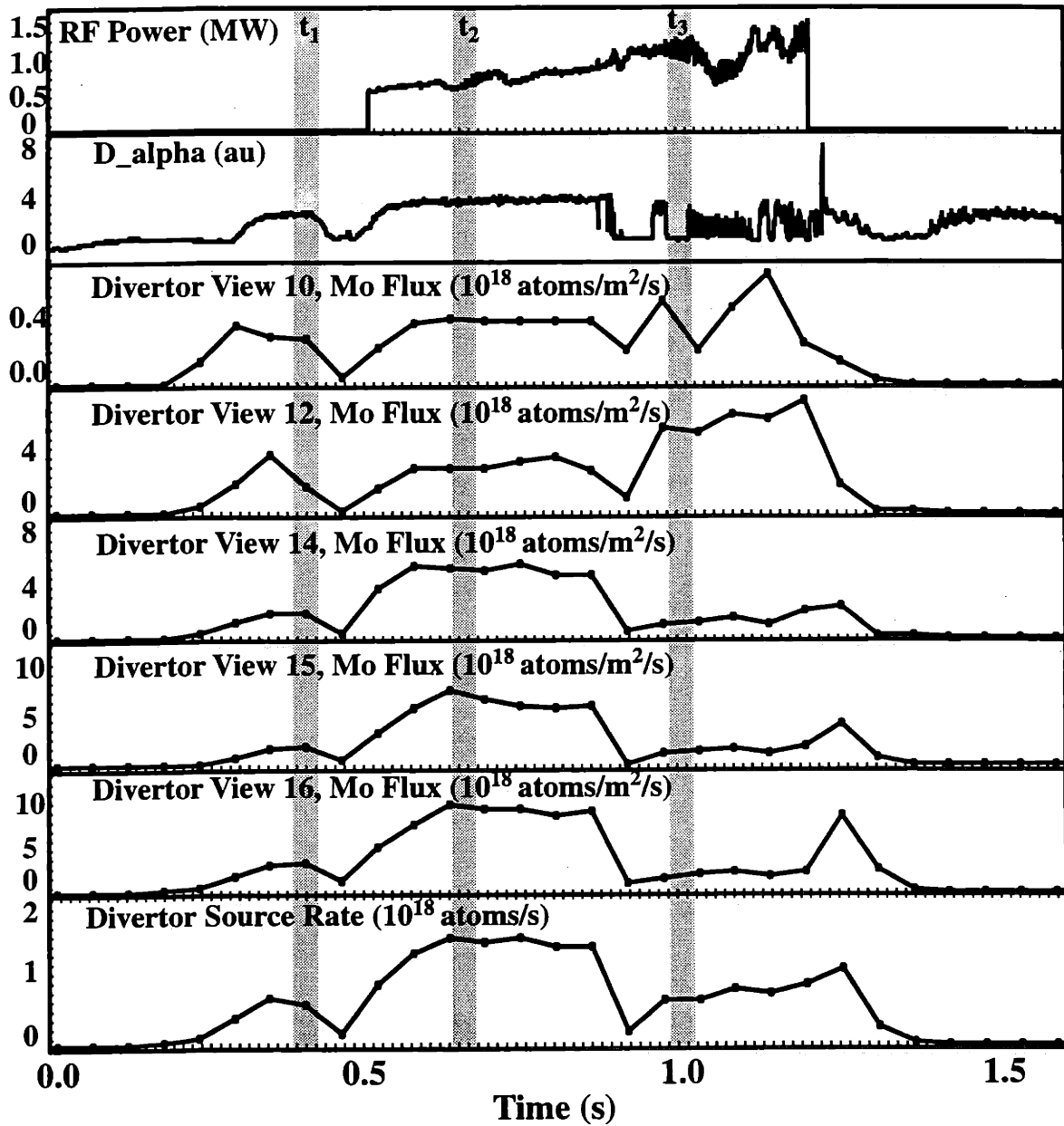
Fig. 3-26: Time histories of the RF power, the D_\alpha signal, the molybdenum influx for views 10, 12, 14, 15, 16, (see Fig. 3-17) and the molybdenum source rate for the discharge that the outer divertor emission profiles are shown in Fig. 3-27. Times " t_1 ", " t_2 ", and " t_3 " indicate the periods for which the profiles are given.
