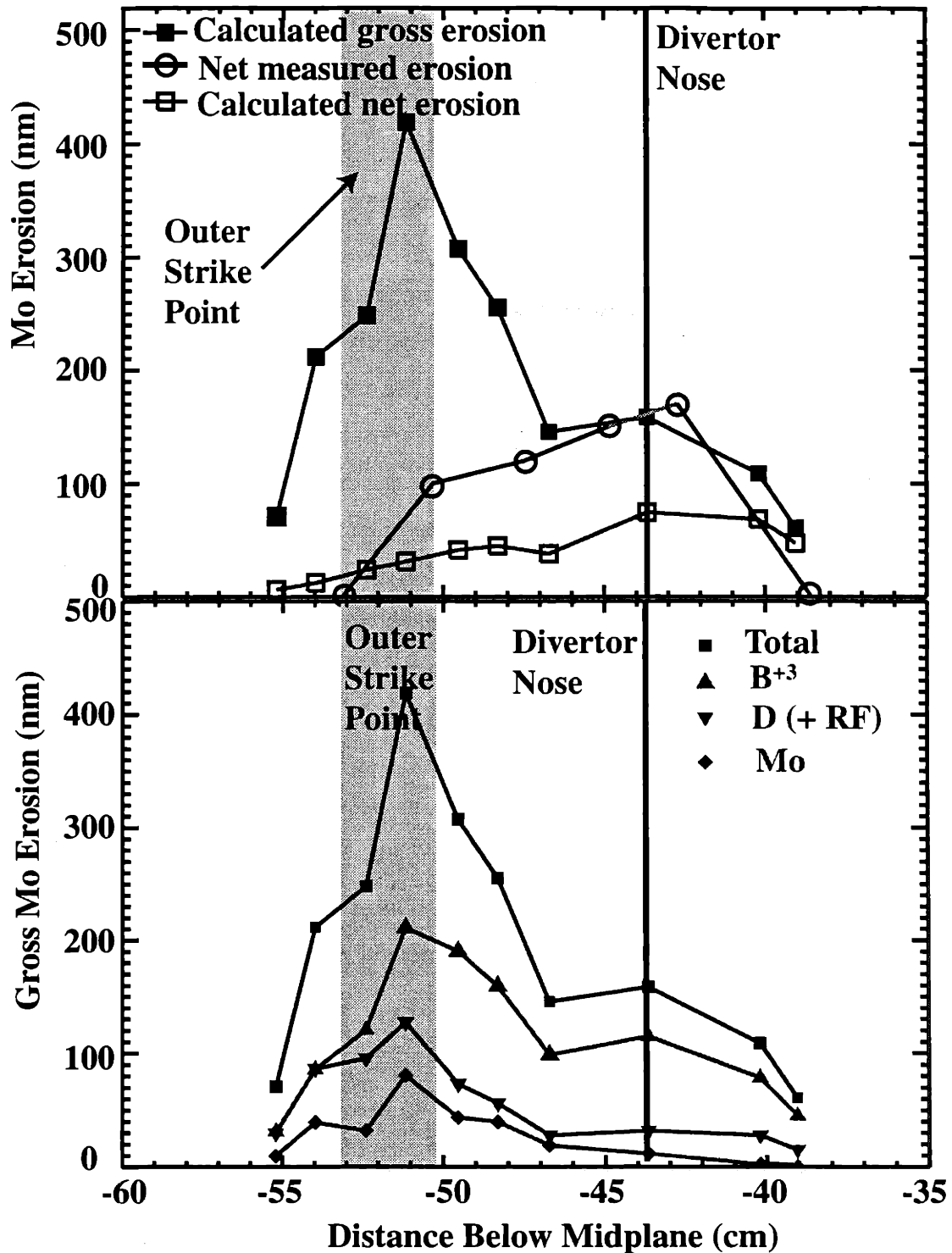
Fig. 5-23: Outer divertor campaign integrated gross and net calculated erosion and net measured erosion as a function of the distance of each of the ten probes below the midplane (top panel). Contribution of the various projectiles used in the model to the total calculated gross erosion (bottom panel).
