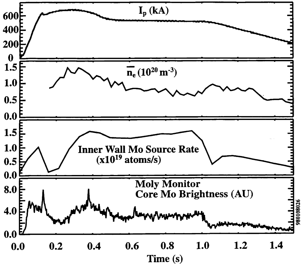
Fig 3-3: Typical time history of the inner wall molybdenum source rate for an inner-wall limited plasma discharge with no auxiliary RF heating. The plasma current, the volume averaged electron density, and the core molybdenum brightness traces (from the Moly Monitor) are also shown.
