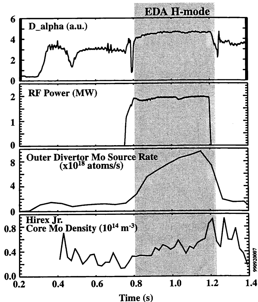
Fig. 3-24: Effect of EDA H-mode to the outer divertor molybdenum source rate. The time histories of the D_\alpha signal, the RF power, the divertor molybdenum source rate, and the core molybdenum density are plotted.
