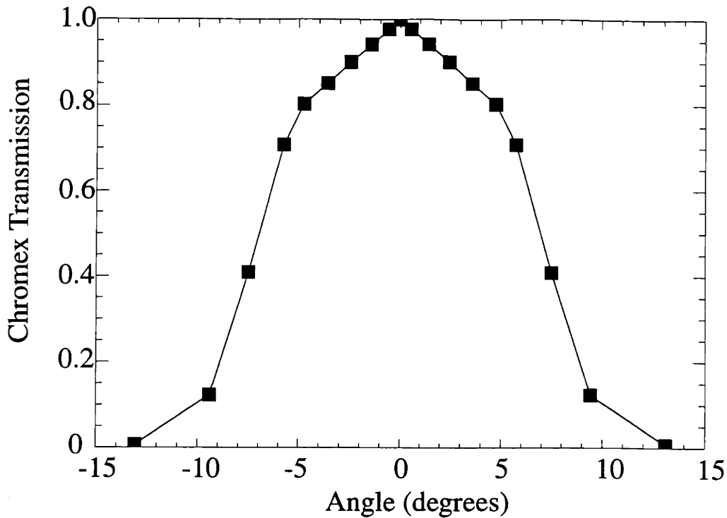
Fig. 2-1: Spectrometer's light transmission as a function of the angle from the normal to the entrance slit [13].
