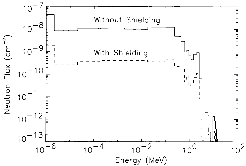
Fig. 2-12: Neutron flux per starting neutron at the CCD, with and without shielding, as calculated by the MCNP.
