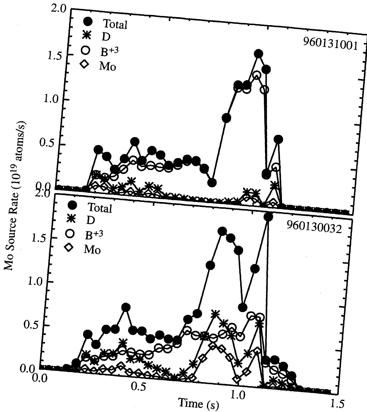
Fig. 5-20: Contribution of the various projectiles used in the model to the calculated molybdenum source rate. The data from two representative shots are given. molybdenum ions in the self-sputtering calculation. Although the probability of redeposition frequently reaches values close to one for the conditions occurring in C-Mod plasmas, it was important to investigate the effect of the rest of the molybdenum ions. Two cases were considered. First, the extreme case in which all these ions are assumed to
