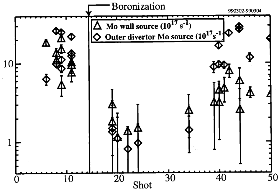
Fig. 4-4: Changes, resulting from boronization, in the outer divertor and inner wall sources for the diverted, RF-heated phase of plasma discharges.
