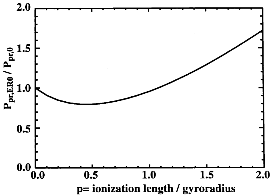
Fig. 5-7: Ratio of the probability of prompt redeposition calculated including all effects to the one obtained from the simplified model.
