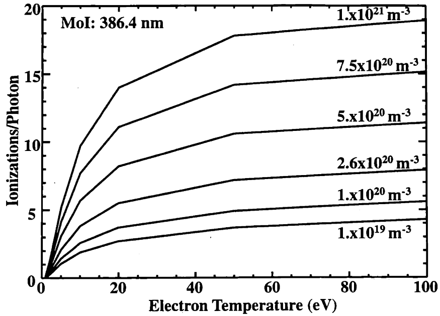
Fig. 2-15: Molybdenum ionizations per 386.4 nm emitted photon ( S/XB ) as a function of the electron temperature for a number of electron densities. Calculated using the data of Table 2-3 that have been multiplied by 3.
