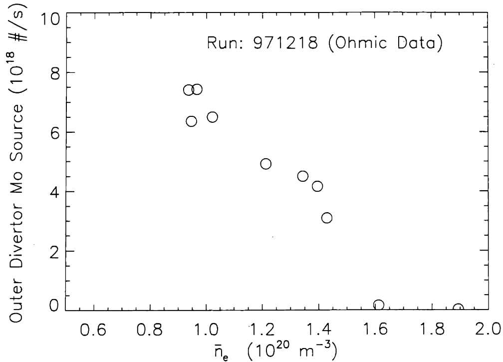
Fig. 3-20: Effect of electron density on the outer divertor molybdenum source rate during the ohmic phase of plasma discharges. The plasma current was 800 kA.
