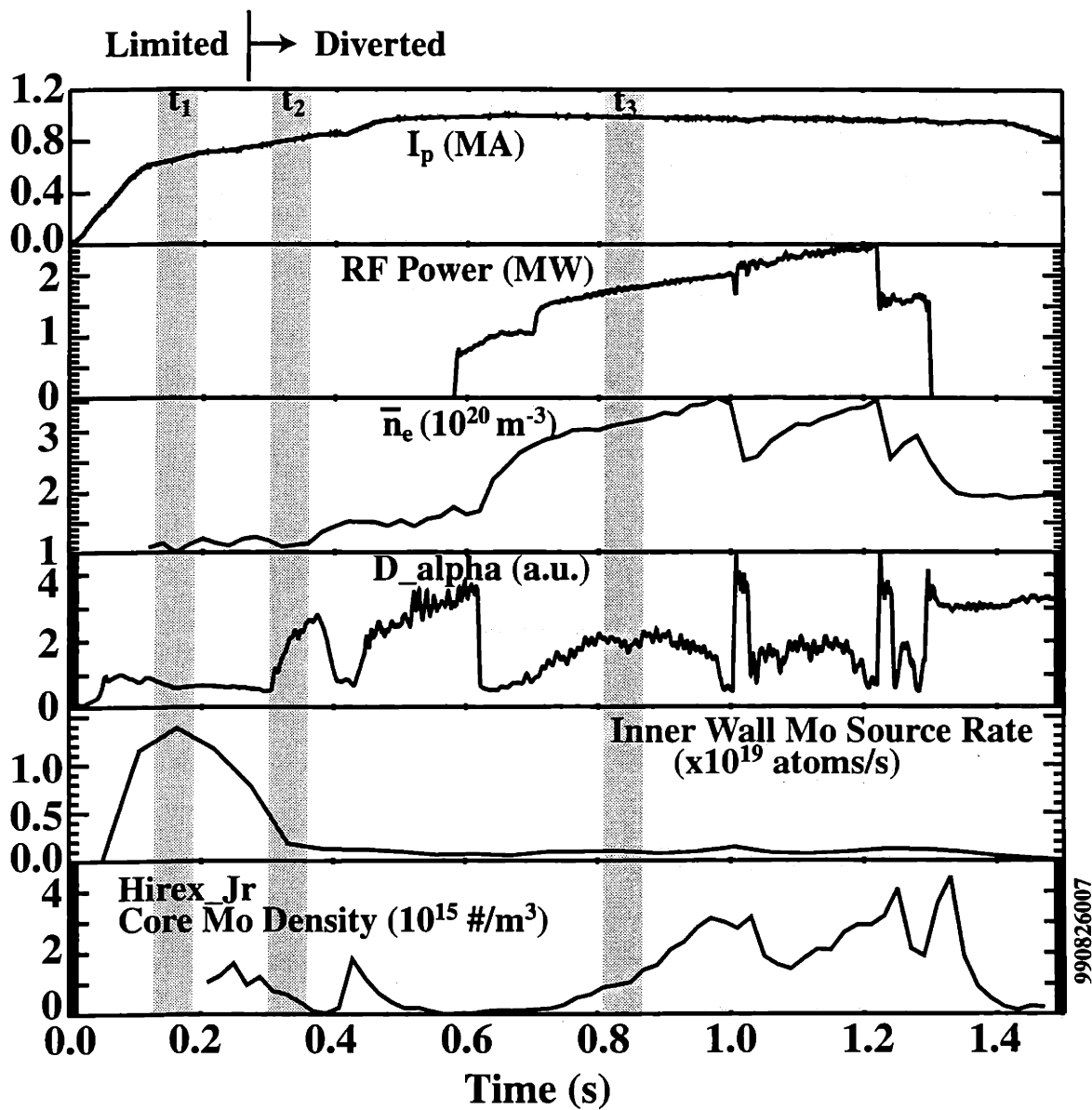
Fig. 3-14: Time histories of the basic plasma parameters and of the inner wall molybdenum source rate for the shot for which the inner wall molybdenum emission profiles are presented in Fig. 3-15. The time slices “t 1 ”, “t 2 ”, and “t 3 ” indicate the periods for which the profiles are given.
