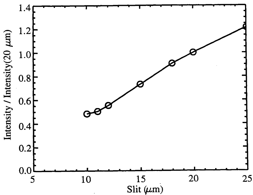
Fig. 2-8: Normalized intensities versus slit width for slits 10 to 25 \mu\text{m} wide. The data are a subset of the data shown in Fig. 2-7.
