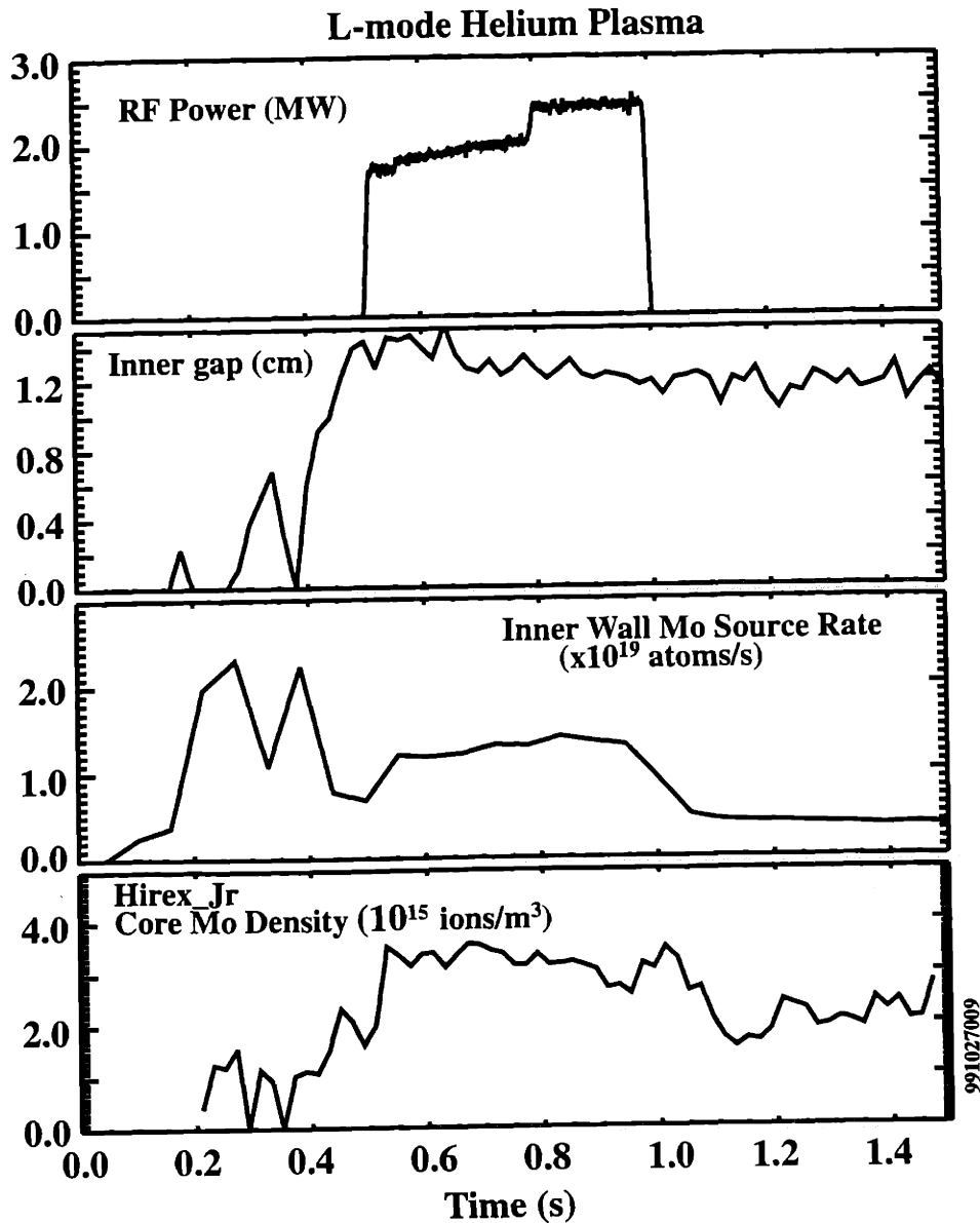
Fig. 3-13: Effect of helium plasmas on molybdenum emissions from the inner wall. The time histories of the RF power, inner gap, inner wall molybdenum source rate, and core molybdenum density are given. The molybdenum source rate during the diverted phase is a factor of 3 higher than typical values observed for deuterium plasmas.
