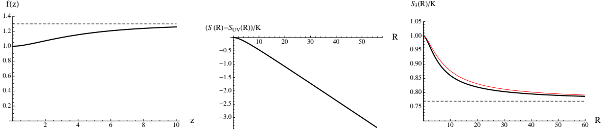
FIG. 3. Left: f(z) for the domain wall solution describing the flow of M2-brane theory to an IR fixed point preserving \mathcal{N} = 2 supersymmetry. Middle: plot of S(R) - S_{UV}(R) where S_{UV} denotes that at the UV fixed point. The UV divergences cancel when taking the difference, but the resulting expression does not have a well-defined large R limit, with a linear R -dependence. As in the case of a free massive scalar and Dirac field of Sec. VI, the presence of such a linear term can be understood as a finite renormalization between the short distance cutoffs of the UV and IR fixed points, as discussed in Sec. II. Right: \mathcal{S}_3(R) for this flow. We normalize the value at UV to be 1. The horizontal dashed line denotes the expected value (7.17) for the IR fixed point. The black line (lower line) is obtained from numerical calculation by using (7.27). For this flow, \epsilon in (7.30) is \epsilon \approx 0.3 , and thus equation (7.37) should be a reasonable approximation, whose results are plotted using the red line (upper line). Note that the part linear in R in -S_{\text{finite}} as seen in the second plot is automatically eliminated when considering \mathcal{S}_3(R) .
