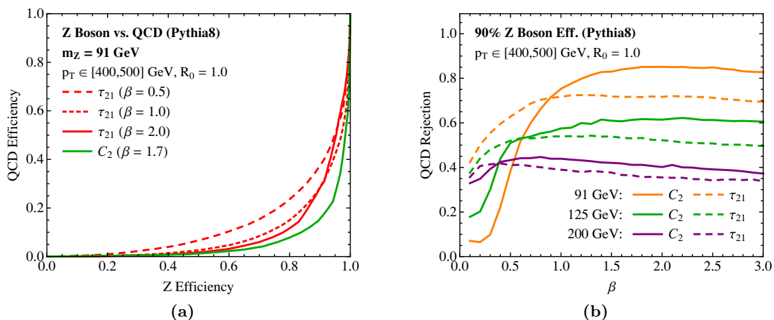
Figure 10. Left: the discrimination curves for boosted hadronic Z bosons ( m_Z = 91 GeV) compared to QCD jets with \tau_{2,1}^\beta for various values of \beta . For comparison is shown the C_2^{(\beta)} curve with the best discrimination ( \beta = 1.7 ). The subjet axes for N -subjettiness are defined as those that minimize the \beta = 1 measure (broadening axes). Right: QCD rejection rate for 90% boosted Z efficiency as a function of \beta , sweeping the value of the Z boson mass to m_Z = \{91, 125, 200\} GeV. Because these curves are with 90% Z efficiency, they are not directly comparable to figure 9b. Note that as m/p_T decreases, the performance of C_2 improves relative to \tau_{2,1} .
