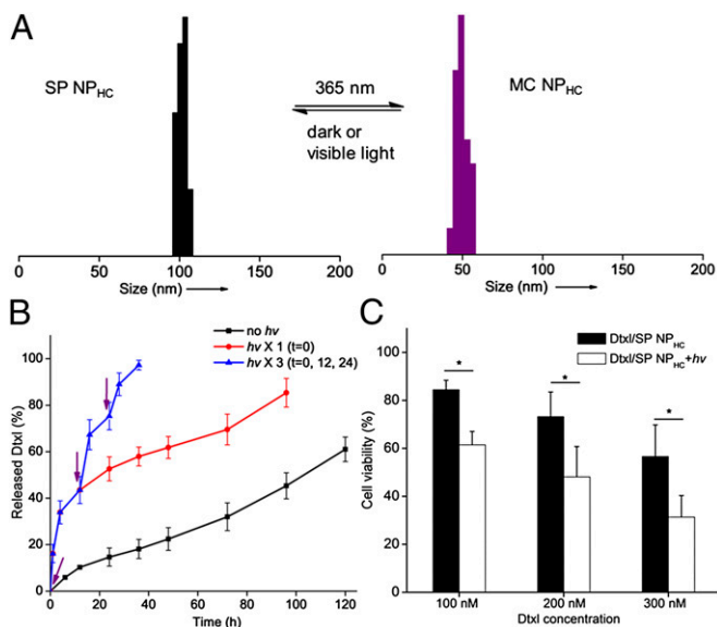
Fig. 1. In vitro characterization of photoswitching SP NP Hc . (A) Dynamic light-scattering measurement of size changes of SP NP Hc s upon alternating UV (35 s) and visible light illumination (500–600 nm, 5 min, 0.5 W/cm 2 ). (B) Release of Dtxl from SP NP Hc in the absence of irradiation; with UV irradiation for 10 s at t = 0 or with repeated UV irradiation at t = 0, 12, 24 h. The times of irradiation are indicated by purple arrows ( n = 5 ). (C) Effect of Dtxl/SP NP Hc on HT-1080 cell viability, by MTT assay. Cells were incubated with NP Hc for 4 h, washed with NP-free media, irradiated (10 s, 1 W/cm 2 ), and further incubated for a total time of 24 h. Data are means \pm SD, n = 6 ; asterisks indicate P < 0.005 . Dtxl, docetaxel; hv, UV irradiation; NP Hc , hybrid NPs with cholesterol; SP, spiropyran.
