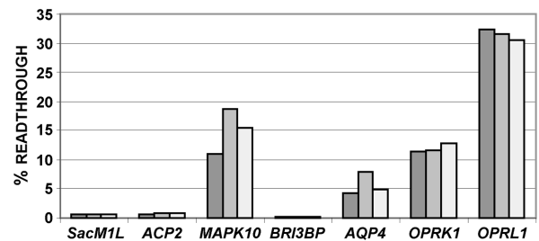
Figure 2. (A) Sequence boundaries of seven readthrough candidates cloned into a dual-luciferase plasmid. Main ORF stop codons are in red font and the conserved CTAG motif is highlighted in bold and underlined. Plasmids were transfected into HEK-293T cells and 24 hr later lysates analysed for readthrough by both western blotting with anti-Renilla (B) and dual-luciferase assay to determine readthrough efficiencies (C). For (B) each TGG in-frame control (I) is adjacent to its respective test (T) construct. For (C) readthrough efficiencies were calculated as the ratio of test construct luciferase activity to its TGG in-frame control from three independent experiments.
