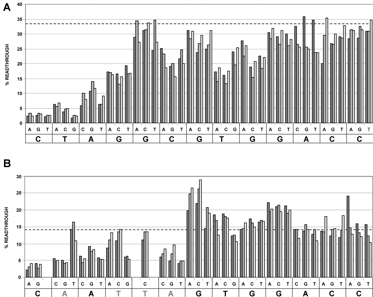
Figure 4. Systematic mutational analysis of the 13 nucleotides immediately 3' of OPRL1 TGA (A) and OPRL1-CARYYA TGA (B). The dotted lines represent the mean readthrough efficiencies of the wild-type OPRL1 (A) and OPRL1-CARYYA (B). Sequences at the bottom of each graph are those of the 13 nucleotides immediately 3' of OPRL1 TGA (A) and OPRL1-CARYYA TGA (B). The triplet of nucleotides immediately above each nucleotide of these sequences represent the substitution mutations (those in B introducing a zero frame stop codon were excluded).
