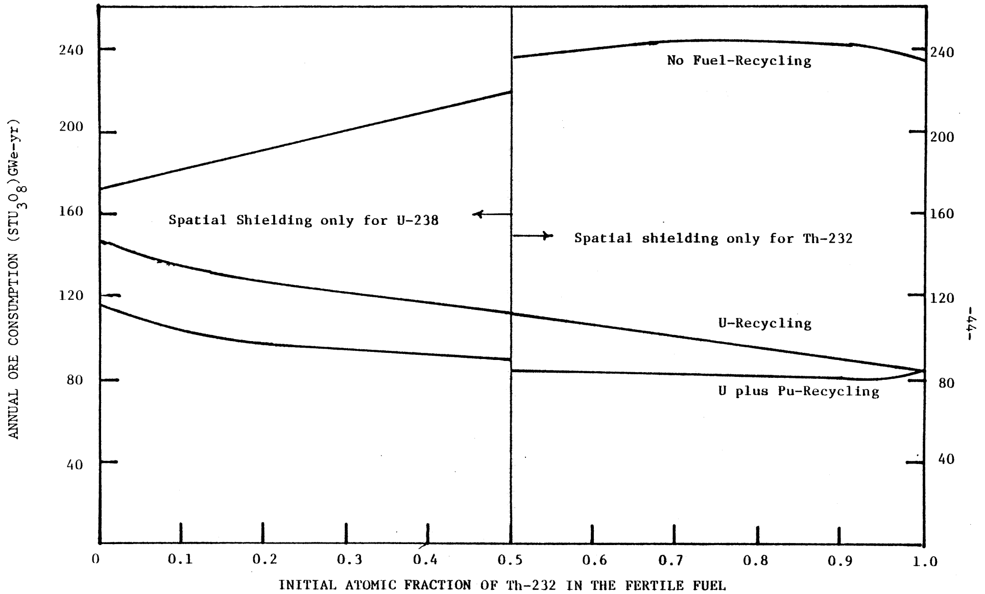
Figure 2.2 ANNUAL ORE CONSUMPTION IN MIXED THORIUM-URANIUM CORES [C-5]
