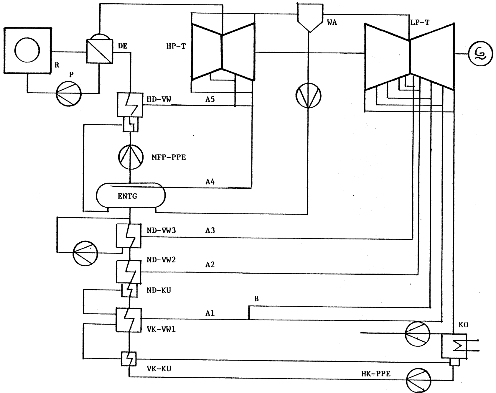
FIGURE 5.2 NUCLEAR STEAM SUPPLY SYSTEM LAYOUT
