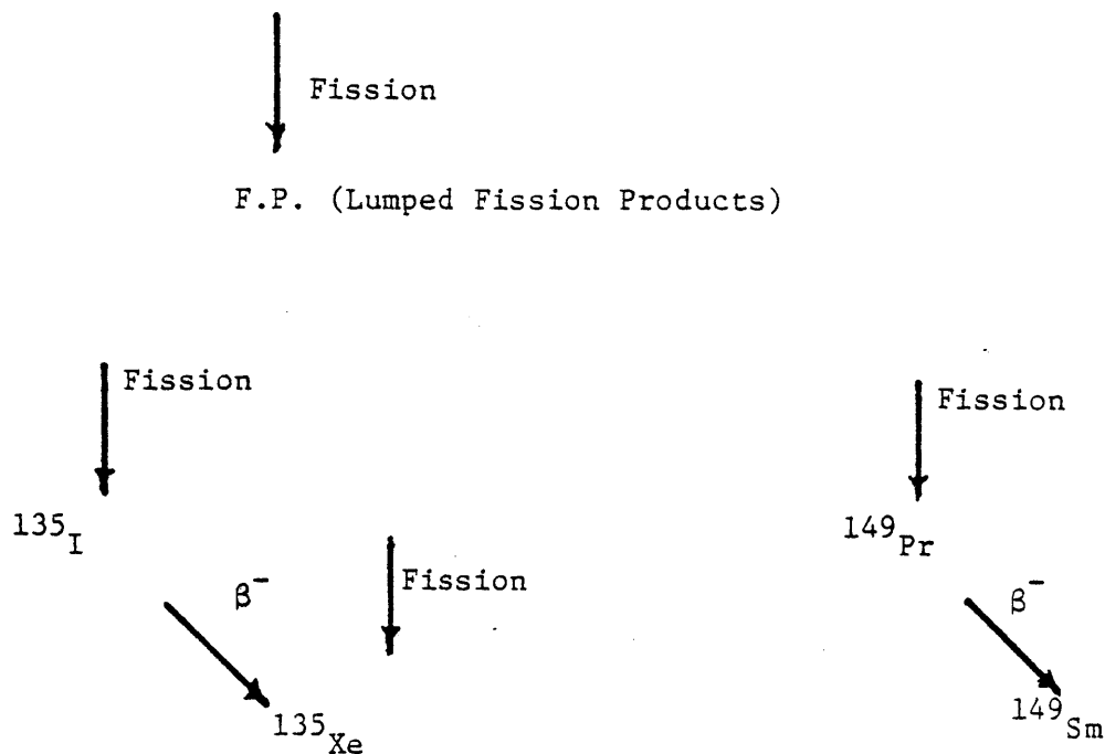
FIGURE 3.3 DEPLETION AND FISSION PRODUCT CHAINS USED IN THE PRESENT STUDY
