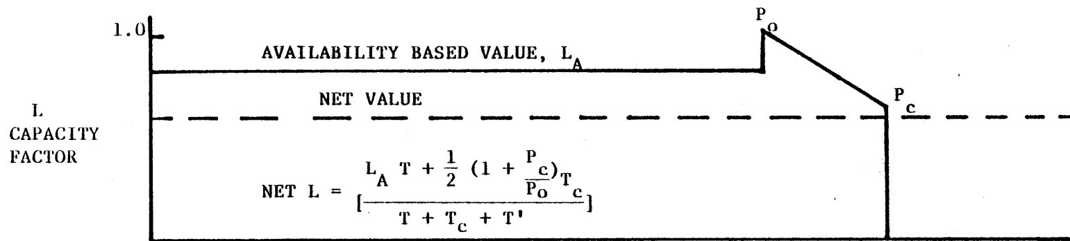
FIGURE F.1 DEFINITION OF CAPACITY FACTOR INCLUDING COASTDOWN OPERATION
