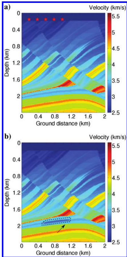
Figure 10. (a) The center part of the original Marmousi model is used as the true baseline velocity model. The maximum source-receiver offset is 2 km. Five shots (red stars) are used to generate synthetic data. (b) True time-lapse velocity model with a negative velocity change marked with a black dashed line. The black arrow points to the area where the boundary of the changes is located in the middle of the layer. We designed this half-layer velocity change intentionally to show how IDWT would smear the changes within a layer.
