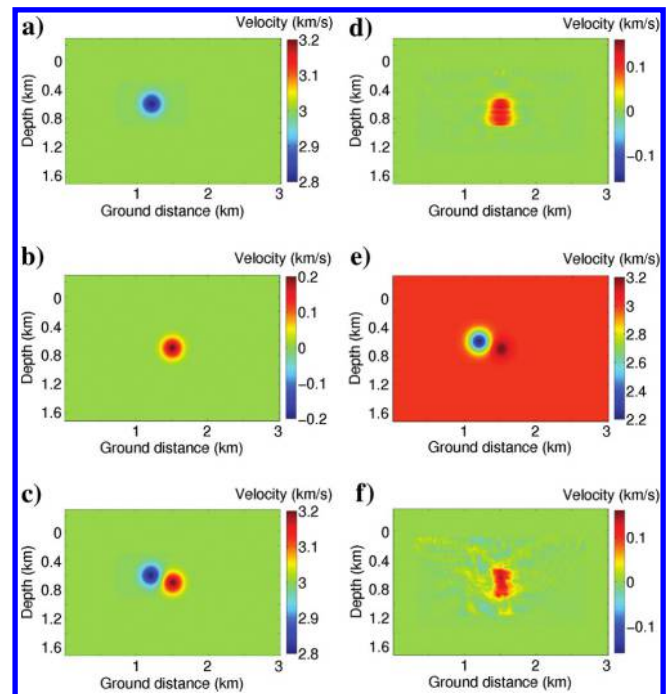
Figure 6. (a) True baseline velocity model with a Gaussian anomaly with peak velocity change of 200 m/s. We assume the anomaly is not known, and we use a constant velocity model for the baseline migrations. (b) True time-lapse velocity changes with peak value of 200 m/s. (c) True time-lapse velocity model I with two Gaussian anomalies (a plus b). (d) The time-lapse velocity changes found using IDWT. (e) True time-lapse velocity model II. We increase the peak amplitude of the Gaussian anomaly in the baseline velocity model to 800 m/s, and we use the same time-lapse velocity changes as in (b). (f) The time-lapse velocity changes inverted by IDWT. The shape of the anomaly is distorted because of the large error in the baseline velocity model, but the basic location and amplitude are preserved.
