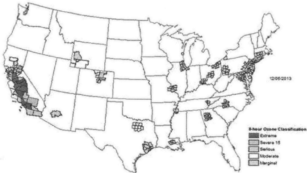
Figure 2: Areas in nonattainment (shaded) for the 8-hour ozone NAAQS (2008 standard) as of December 2013 (U.S. Environmental Protection Agency, 2013a). Partially shaded counties indicate that only part of the county is in nonattainment.
