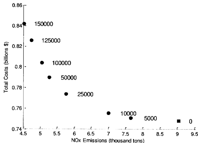
Figure 11: Total cost versus NO x emissions on high ozone days in ERCOT under various time-differentiated prices. Labels next to each point indicate the time-differentiated price assessed per ton of NO x emissions.
