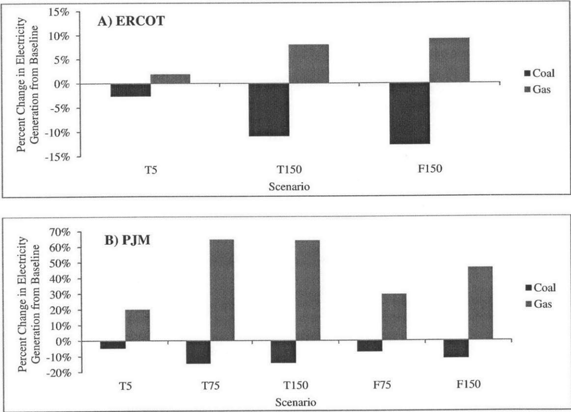
Figure 32: Percent change in electricity generation from baseline over the entire summer by coal-fired (black) and gas-fired (gray) generators in ERCOT (A) and PJM (B) under various time-differentiated prices (labeled with 'T' and the price in thousands $/ton) and technology-based standards (labeled with 'F' and the time-differentiated price on which SCR installations are based).
