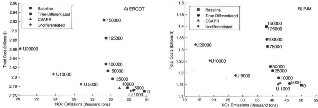
Figure 23: Costs versus NOx emissions for the entire summer in ERCOT (left) and PJM (right) for various time-differentiated prices (circles, labeled in $/ton) and un-differentiated prices (gray diamonds, labeled with 'U' and the price in $/ton). An undifferentiated price based on outcomes expected under the CSAPR (gray triangle) is also presented.
