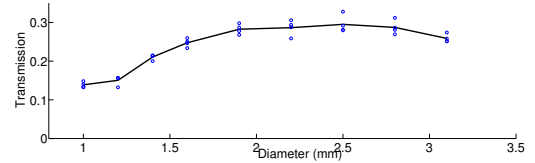
Fig. 5. Transmission as a function of cross-section diameter (mm) measured for a fiber of 8 cm of bending radius. Multiple conflicting diameter-related factors influence transmission including number of light bounces and incidence angle resulting in a sweet spot.
