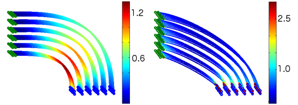
Fig. 10. On the right, fibers generated by minimizing the thin-plate energy resulting in higher curvature in concentrated regions. On the left, minimizing the third derivative energy which results in more uniform curvature. Plots display color coded curvature at different scales.
