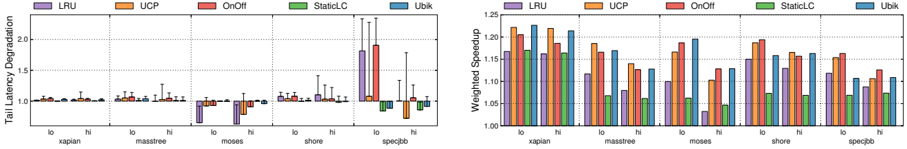
Figure 10: Tail latency degradation (lower is better) and weighted speedup (higher is better) of all schemes vs a private LLC baseline, for the 400 mixes simulated, split by latency-critical app and load, using OOO cores. The left graph shows both overall (bar) and worst-mix (whisker) tail latencies; the right graph shows average weighted speedups.
