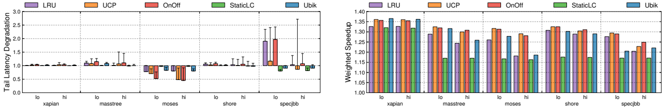
Figure 11: Results with simple in-order (IPC=1) cores: tail latency degradation (lower is better) and weighted speedup (higher is better) of all schemes vs a private LLC baseline, for the 400 mixes simulated, split by latency-critical app and load.
