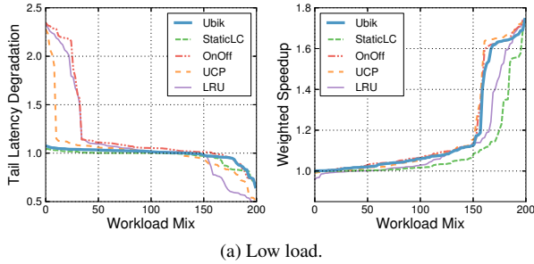
Figure 9: Distribution of tail latency degradation (latency-critical apps, lower is better) and weighted speedup (batch apps, higher is better) for all schemes vs a private LLC baseline, for the 400 mixes simulated, split into low and high loads (200 mixes each).
