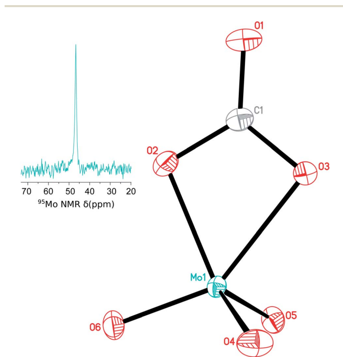
Fig. 1 Left: ^{95}\text{Mo} NMR resonance of [\text{MoO}_3(\kappa^2\text{-CO}_3)]^{2-} . Right: solid-state structure of [\text{NEt}_4]_2[\text{MoO}_3(\kappa^2\text{-CO}_3)] (ellipsoids at the 50% probability level, cations omitted for clarity). Representative interatomic distances [ \text{\AA} ] and angles [ ^\circ ]: C1–O1 1.2258(13) , C1–O2 1.3357(14) , C1–O3 1.3048(13) , Mo1–O2 2.0674(9) , Mo1–O3 2.2191(9) , Mo1–O4 1.7351(8) , Mo1–O5 1.7390(8) , Mo1–O6 1.7436(8) ; C1–O2–Mo1 97.75(6) , C1–O3–Mo1 91.74(7) , O6–Mo1–O3 148.75(3) , O4–Mo1–O2 120.28(4) , O5–Mo1–O2 121.93(4) , O4–Mo1–O5 110.10(4) , O4–Mo1–O6 105.15(4) , O5–Mo1–O6 105.34(4) ; C1–O3–Mo1–O6 2.09(11) , C1–O2–Mo1–O4 75.02(8) , C1–O2–Mo1–O5 -71.35(8) .
