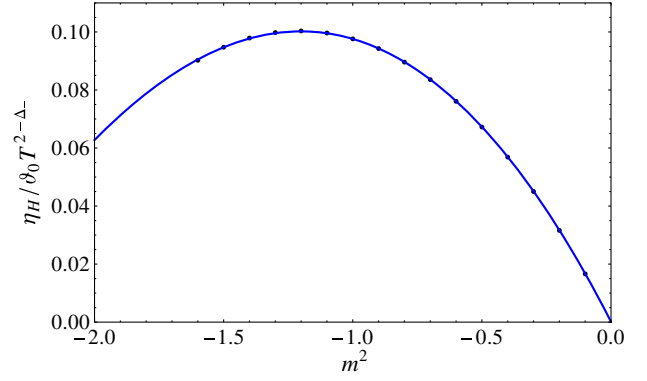
FIG. 4 (color online). \eta_H/\vartheta_0 T^{2-\Delta_-} as a function of m^2 for \vartheta_0/T^{\Delta_-} = 1/6 .
