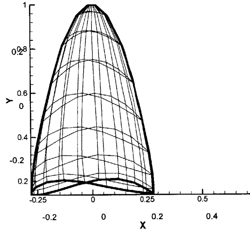
Figure 3-1: XY -coordinates for blade thickness discretization on the pressure and suction sides.
