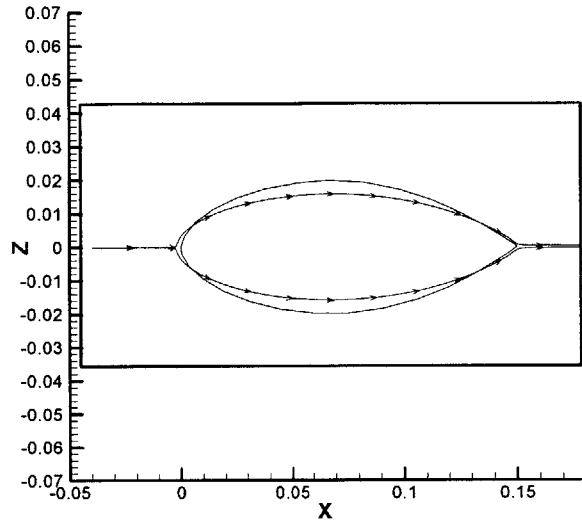
Figure 4-1: Linearized slender-body theory velocity streamline results for a NACA66 modified blade section with \frac{t}{D} = 0.020 and \alpha = 0^\circ in a uniform inflow.
