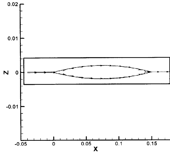
Figure 4-15: Linearized slender-body theory velocity streamline results for a Biconvex blade section with \frac{t}{D} = 0.002 and \alpha = 0^\circ in a uniform inflow.
