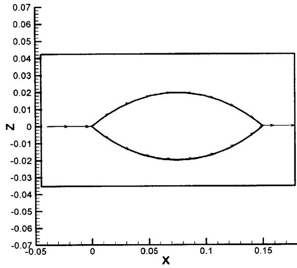
Figure 4-4: Source panel method velocity streamline results for a Biconvex blade section with \frac{t}{D} = 0.020 and \alpha = 0^\circ in a uniform inflow.
