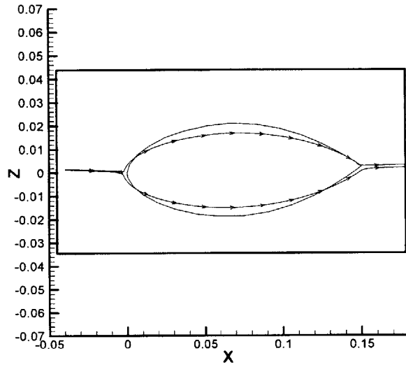
Figure 4-5: Linearized slender-body theory velocity streamline results for a NACA66 modified blade section with \frac{t}{D} = 0.020 and \alpha = 1^\circ in a uniform inflow.
