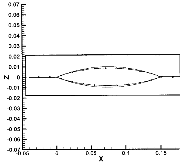
Figure 4-13: Linearized slender-body theory velocity streamline results for a Biconvex blade section with \frac{t}{D} = 0.010 and \alpha = 0^\circ in a uniform inflow.
