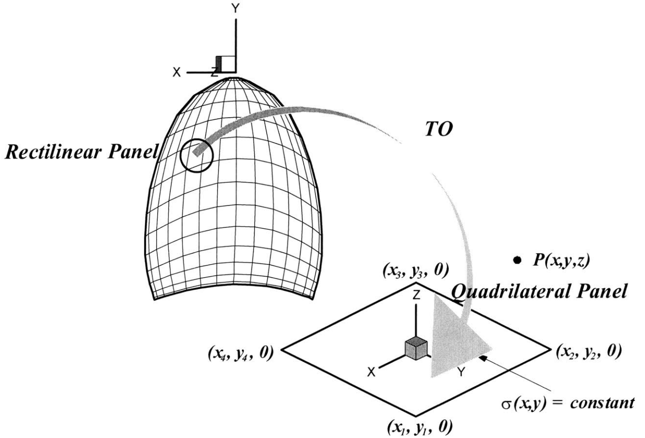
Figure A-1: Rectilinear to Quadrilateral constant-strength source panel transformation.
