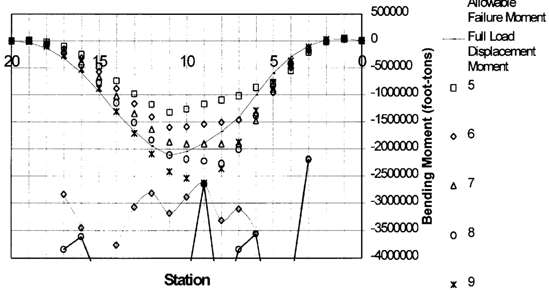
CVN 77 Sagging Bending Moment +11Ktons at stations 5 to 9
