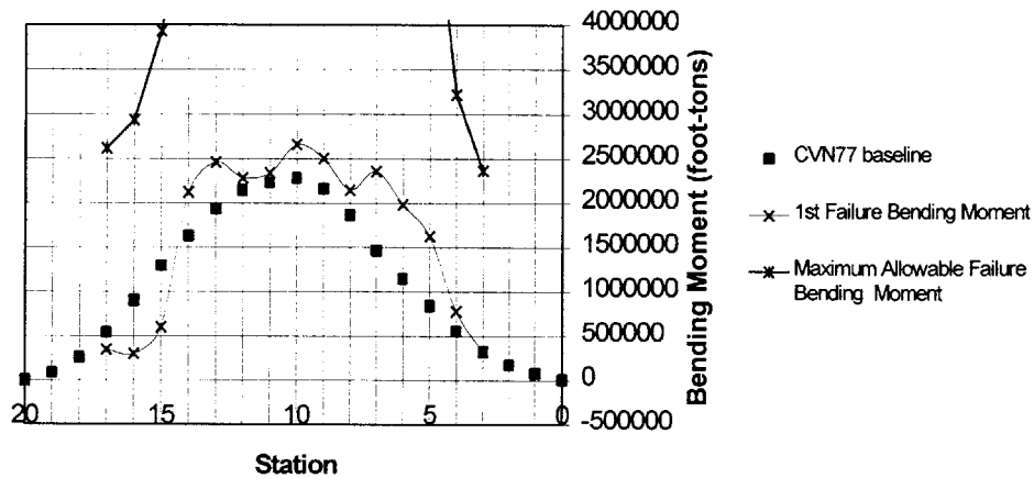
Figure 5. CVN 77 Hogging Baseline Bending Moment Comparison.
