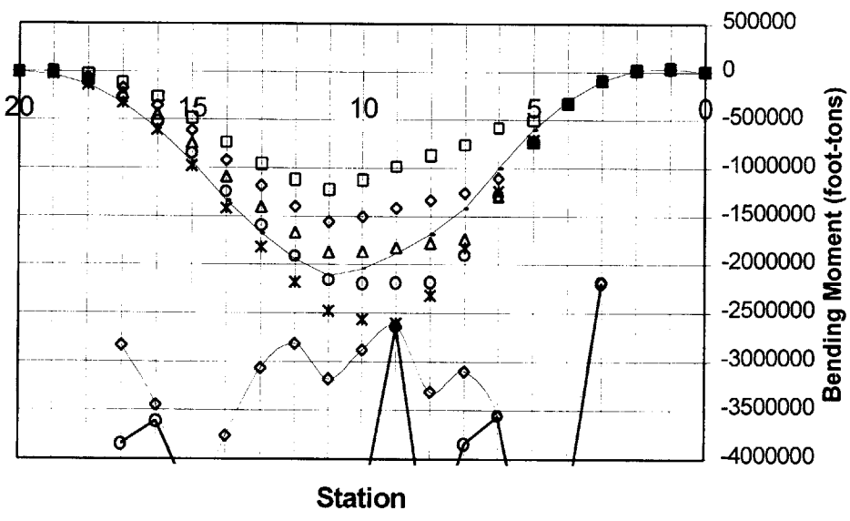
CVN 77 Sagging Bending Moment +10Ktons at stations 5 to 9
