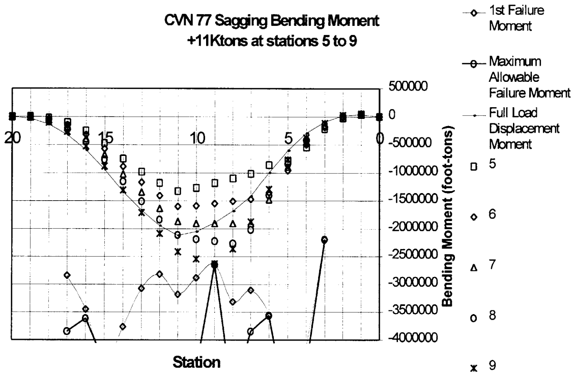
Figure 9. Sagging Bending Moment with 11,000 LTON point load applied at stations 5 to 9.
