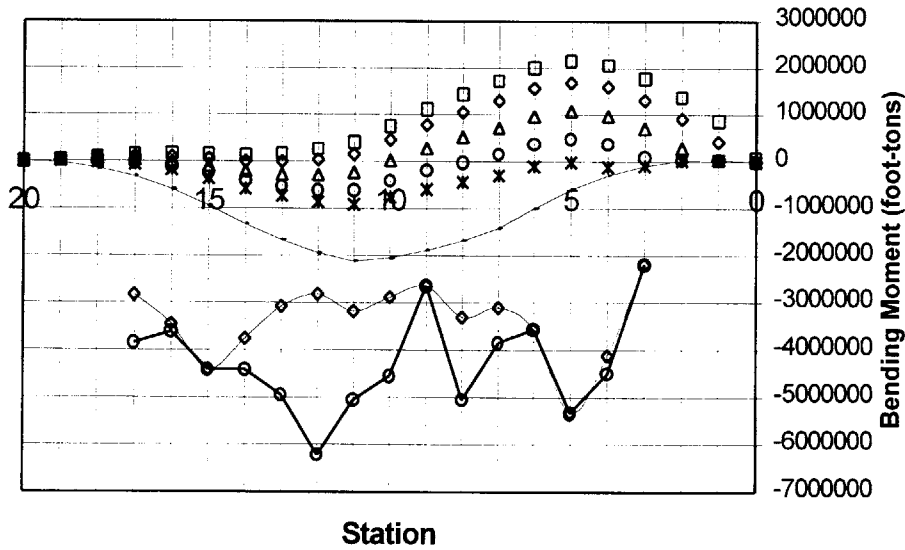
CVN 77 Sagging Bending Moment +10Ktons at stations 0 to 4
