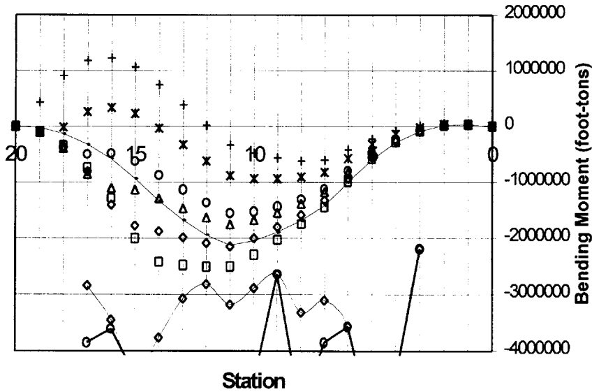
CVN 77 Sagging Bending Moment +15Ktons at stations 15 to 20
