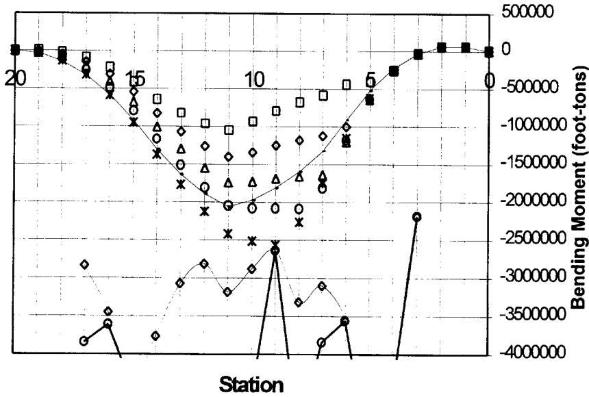
CVN 71 Sagging Bending Moment +11Ktons at stations 5 to 9
