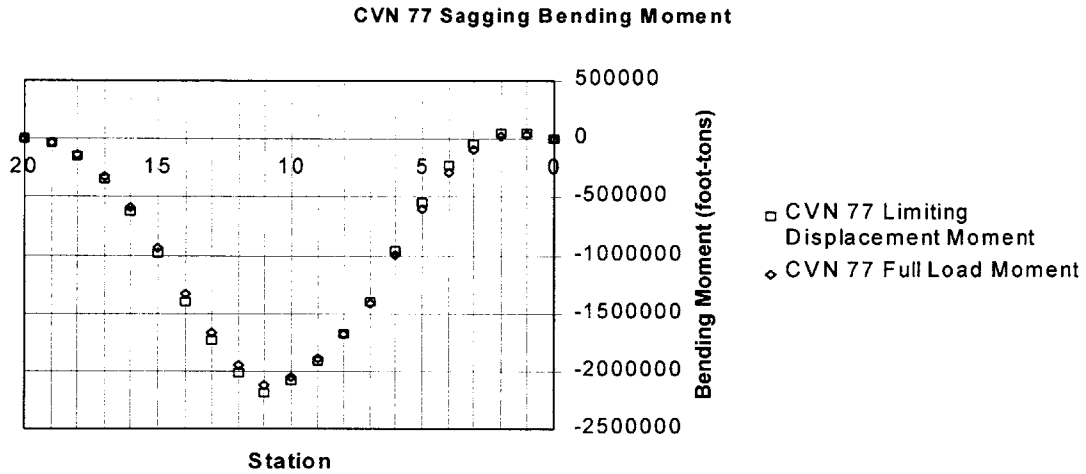
Figure 7. CVN 77 Full Load and Limiting Displacement Sagging Bending Moment Comparison with 11,000 LTONS added proportional to full load weight distribution.
