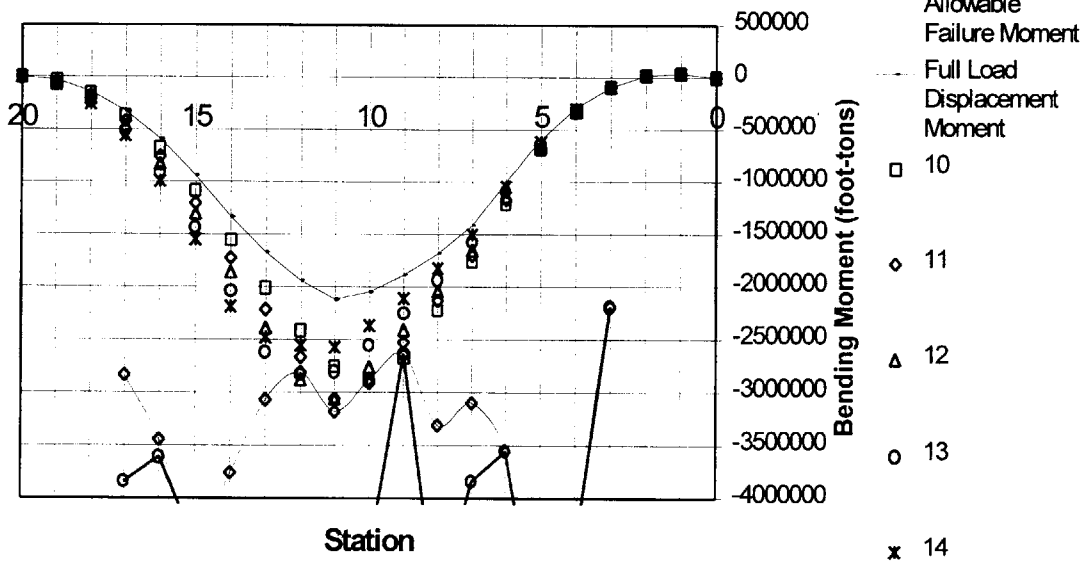
CVN 77 Sagging Bending Moment +10Ktons at stations 10 to 14
