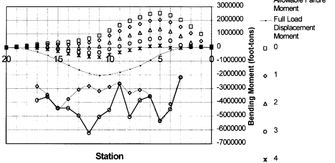
CVN 71 Sagging Bending Moment +11Ktons at stations 0 to 4
