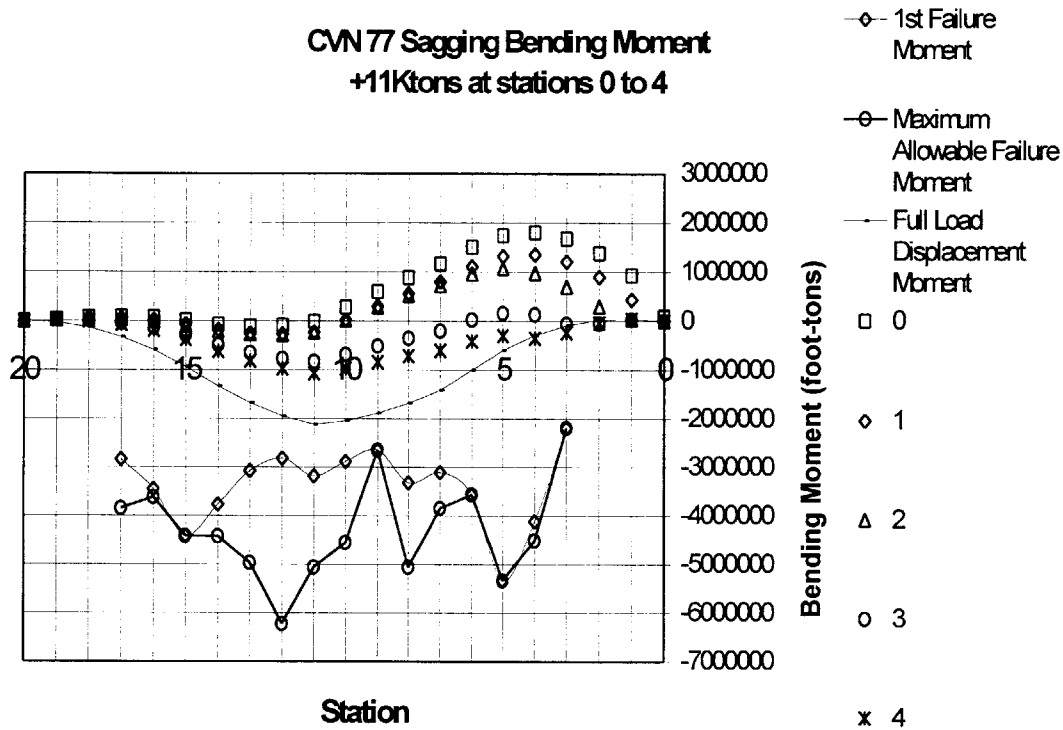
Figure 8. Sagging Bending Moment with 11,000 LTON point load applied at stations 0 to 4.
