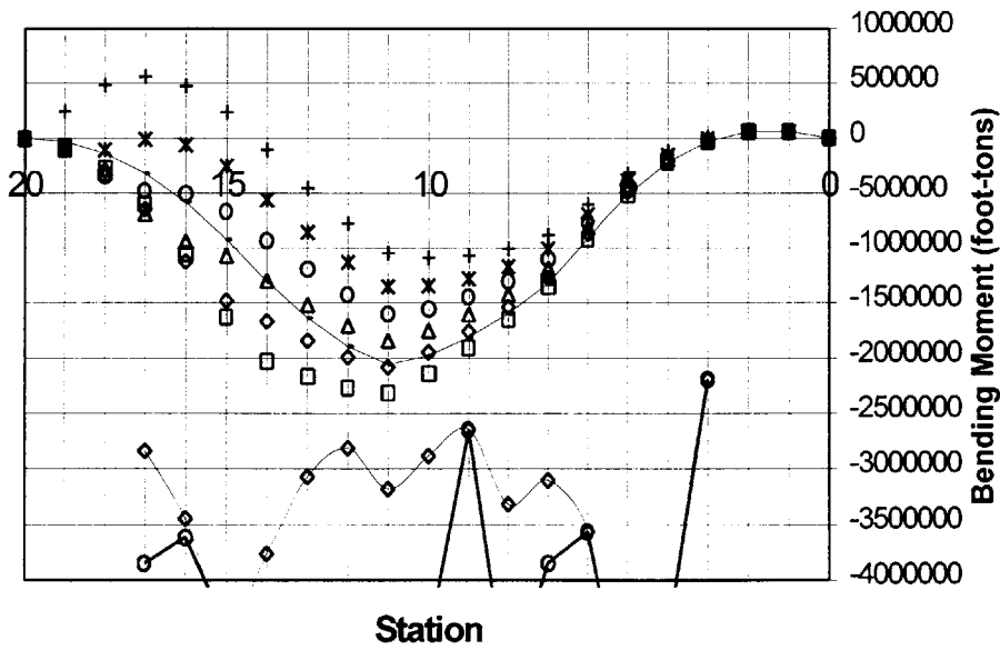
CVN 71 Sagging Bending Moment +10Ktons at stations 15 to 20
