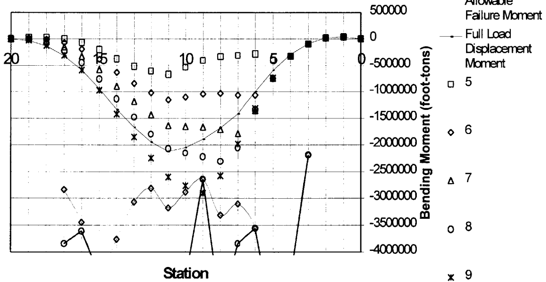
CVN 77 Sagging Bending Moment +15Ktons at stations 5 to 9
