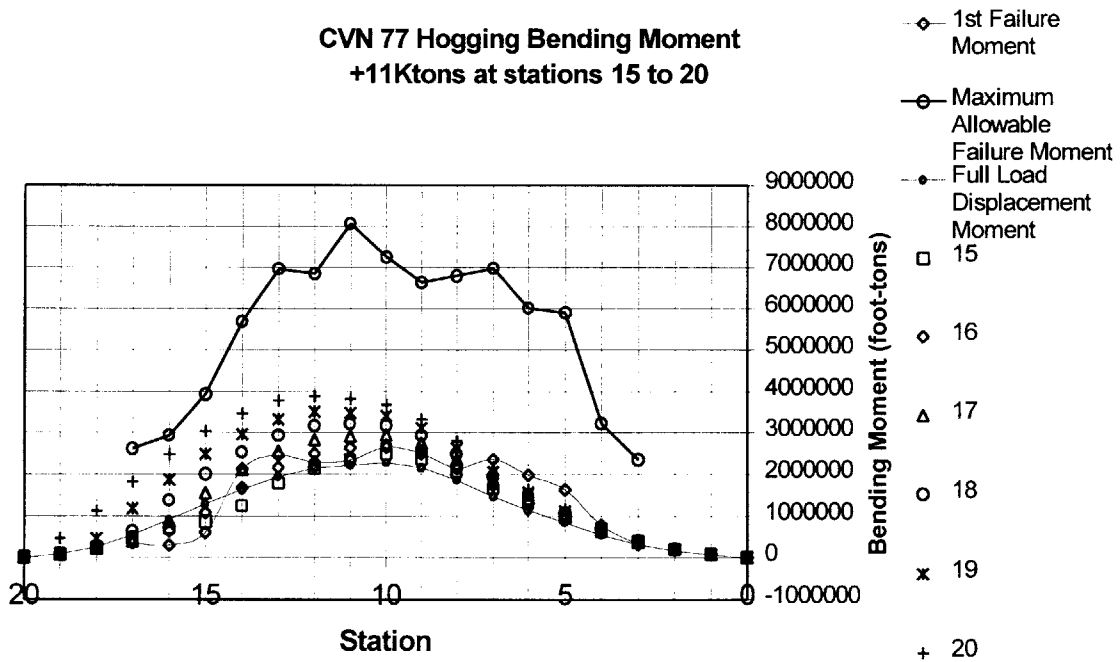
Figure 15. Hogging Bending Moment with 11,000 LTON point load applied at stations 15 to 20.
