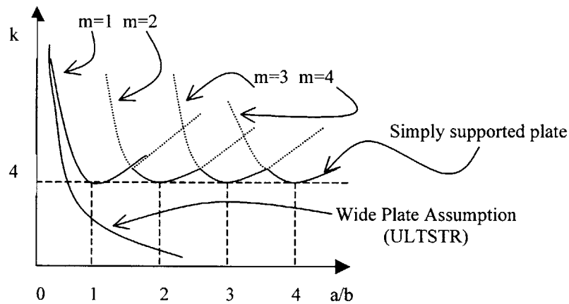
Figure 3. Buckling Coefficient vs. Aspect Ratio.
