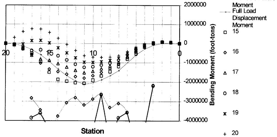
CVN 77 Sagging Bending Moment +11Ktons at stations 15 to 20
