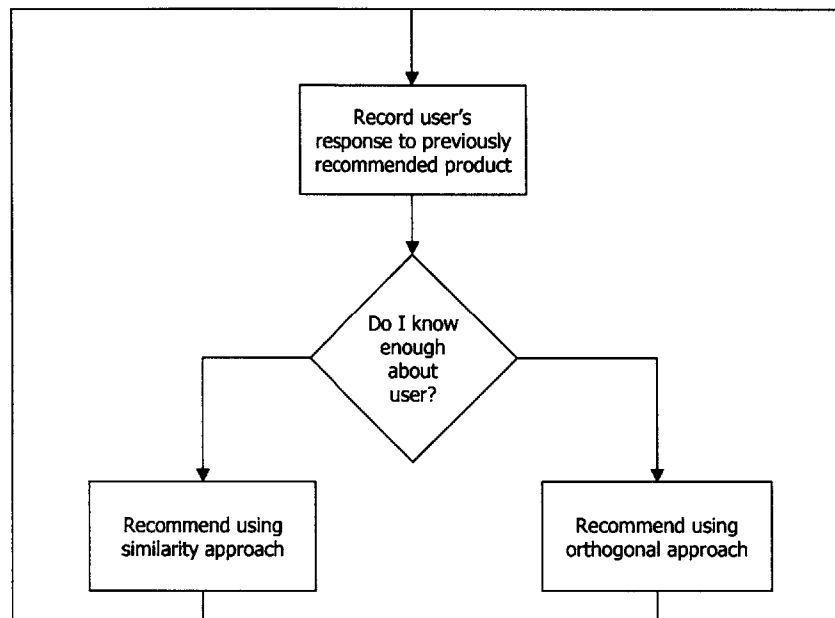
Figure 10: Learning flow with both similarity and orthogonal approaches
