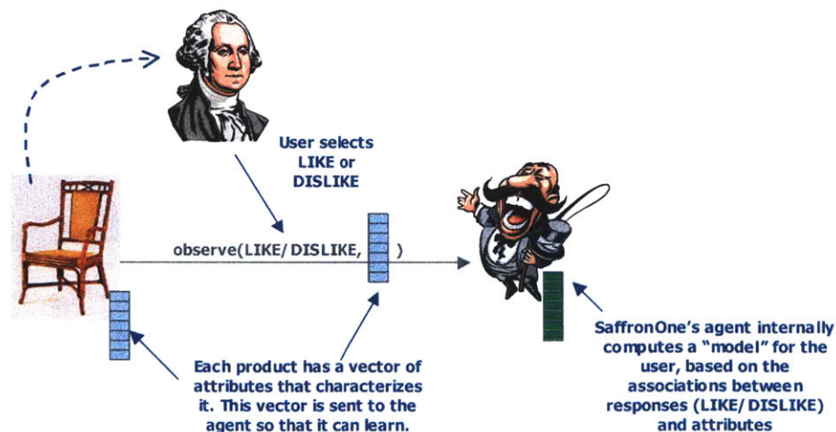
Figure 22: Learning in SaffronOne through the observe() call
