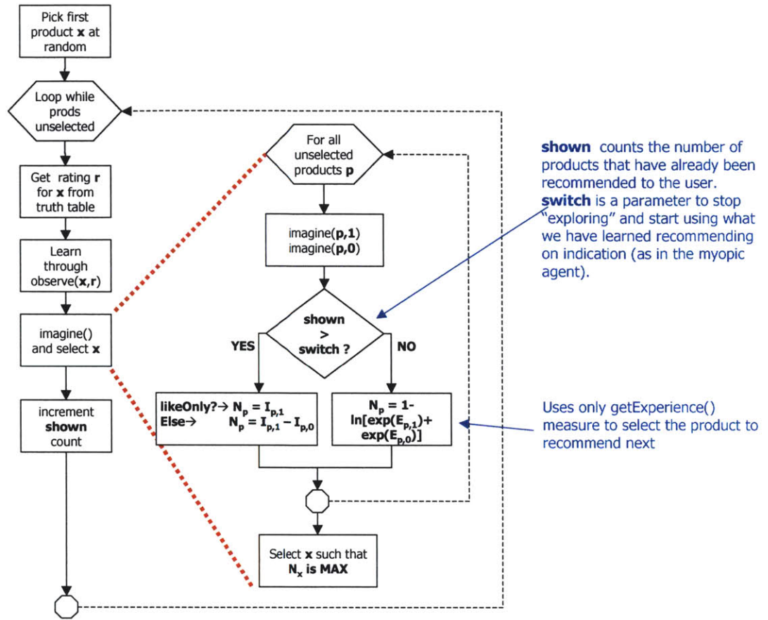
Figure 27: Active learning agent logic flow
