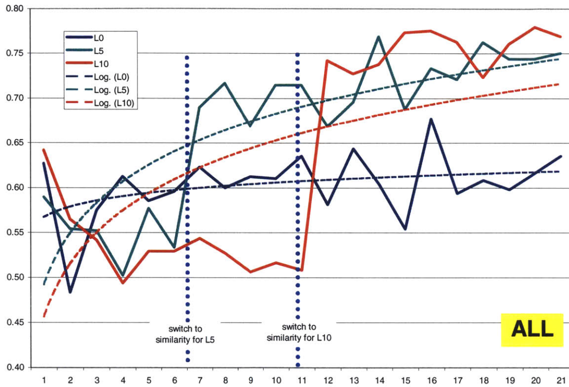
Figure 13: Results - all subjects
