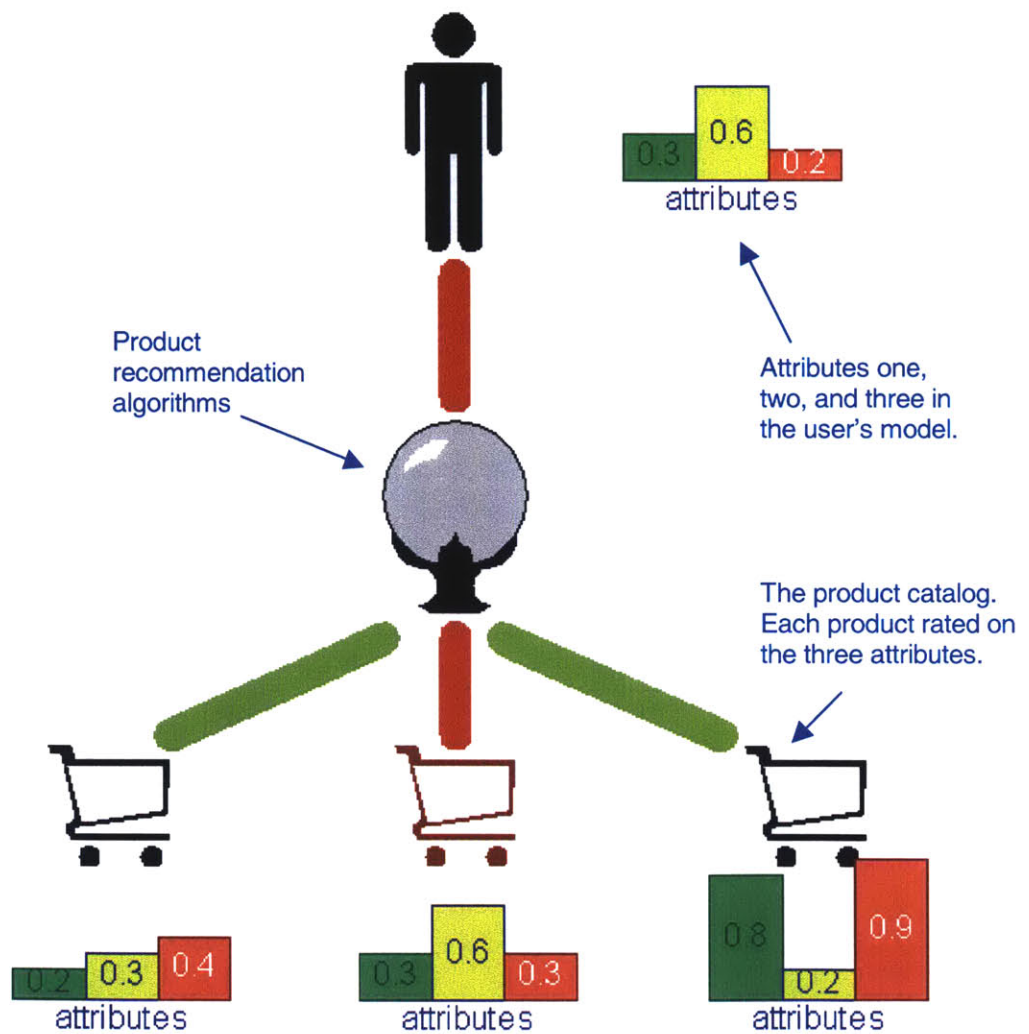
Figure 6: Attribute-based selection example
