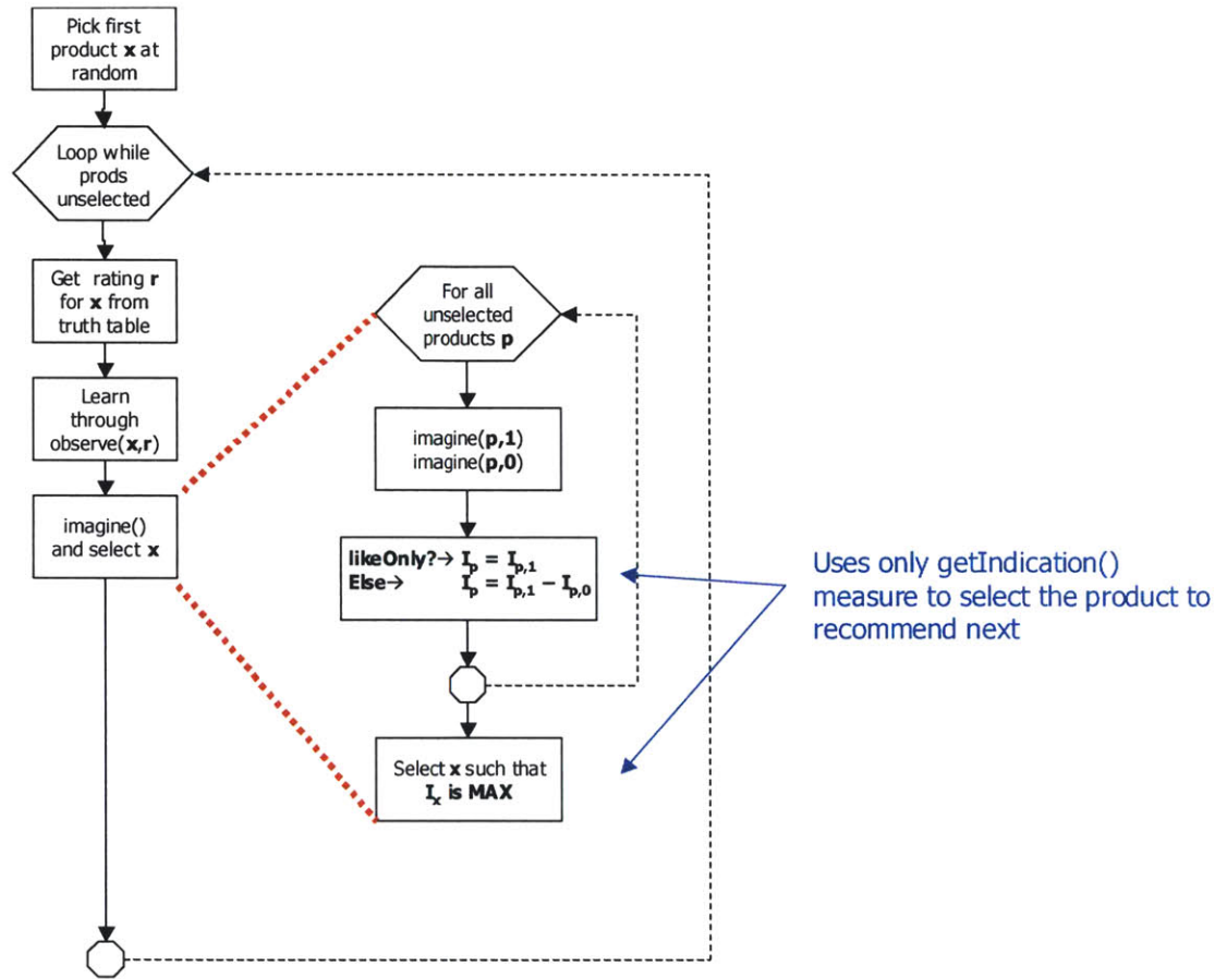
Figure 26: Myopic agent logic flow
