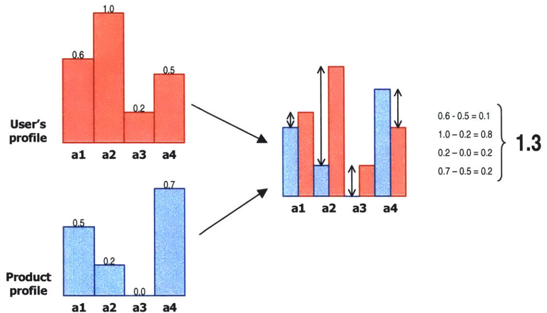
Figure 11: Computing the similarity by profile distance
