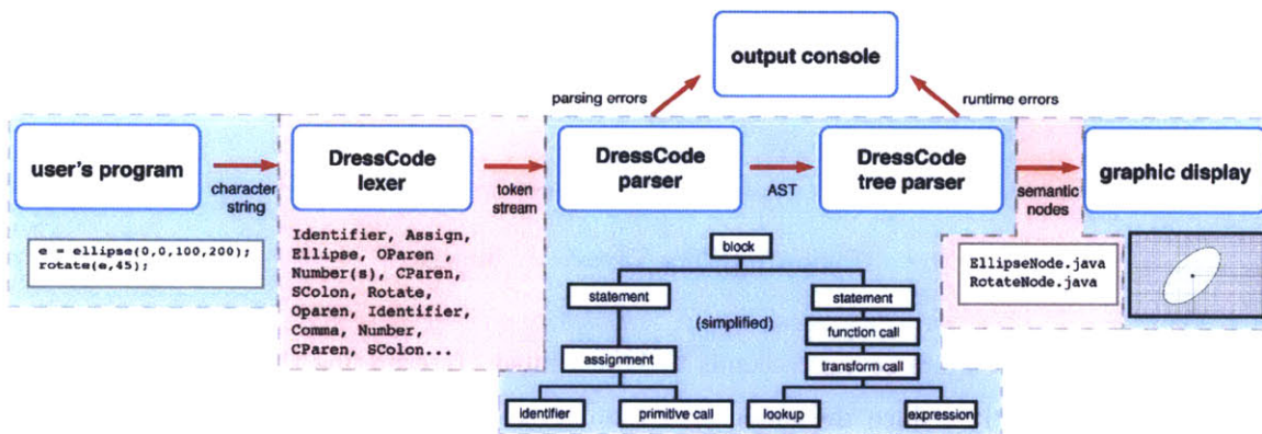
Figure 7-2: Interpreter structure
