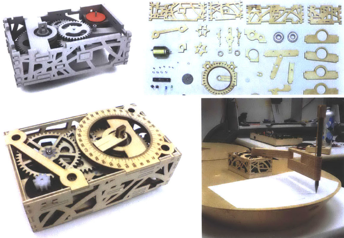
Figure 2-10: Plywood Servo by Peter Schmitt (2011). (Clockwise from upper-left: 3D CAD model of partially constructed servo, laser-cut plywood parts and electronic components, Audiograph, completed servo.)
