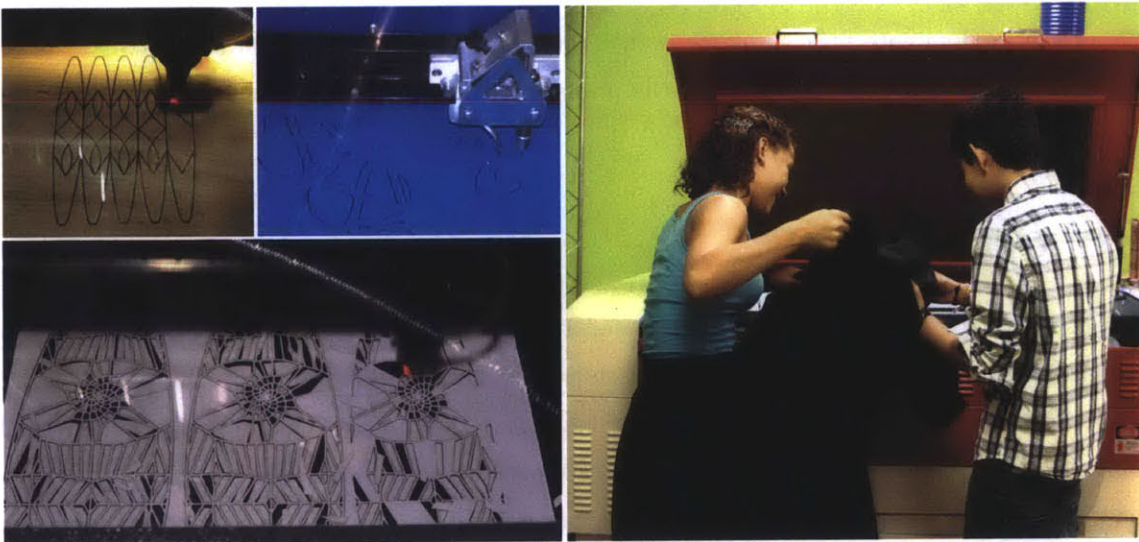
Figure 2-8: Various materials on the laser cutter. (Clockwise from top-left: laser-cut wood veneer, laser-cut fabric, loading fabric into the laser cutter directly from the bolt, laser-cut paper)
